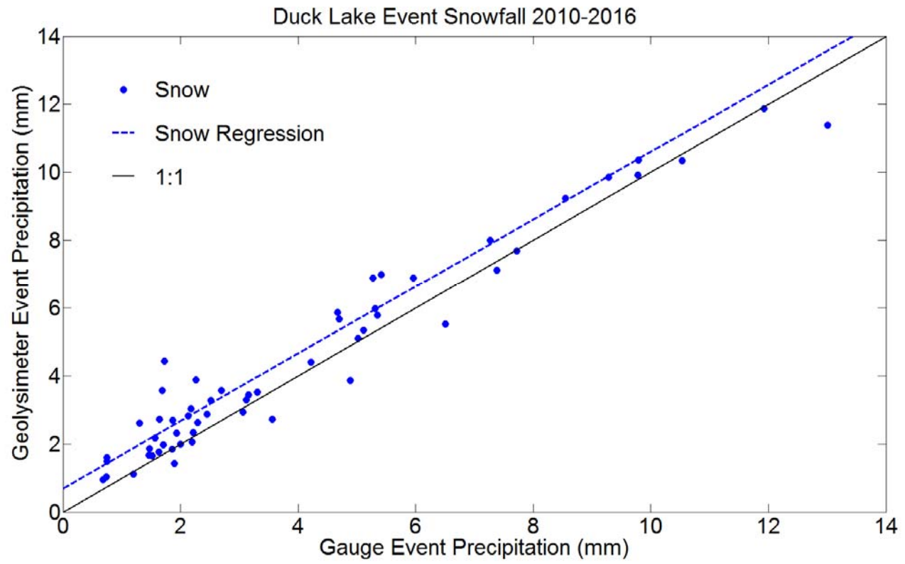
Figure 5: Duck Lake geolysimeter event snowfall compared with gauge event snowfall. Regression line for snow and the 1:1 line are also shown.
