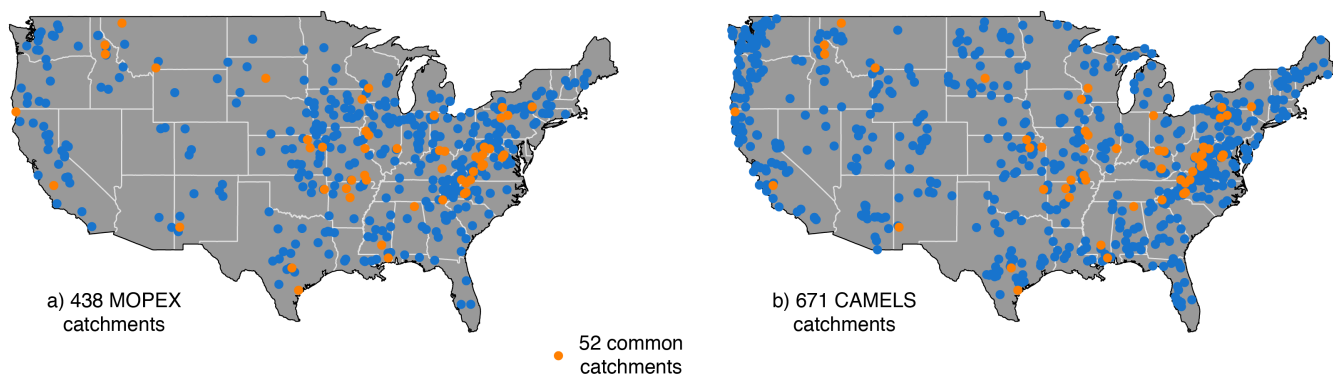
Figure 7: A comparison of the spatial distribution of the catchments from a) the MOPEX data set and b) the CAMELS data set.
