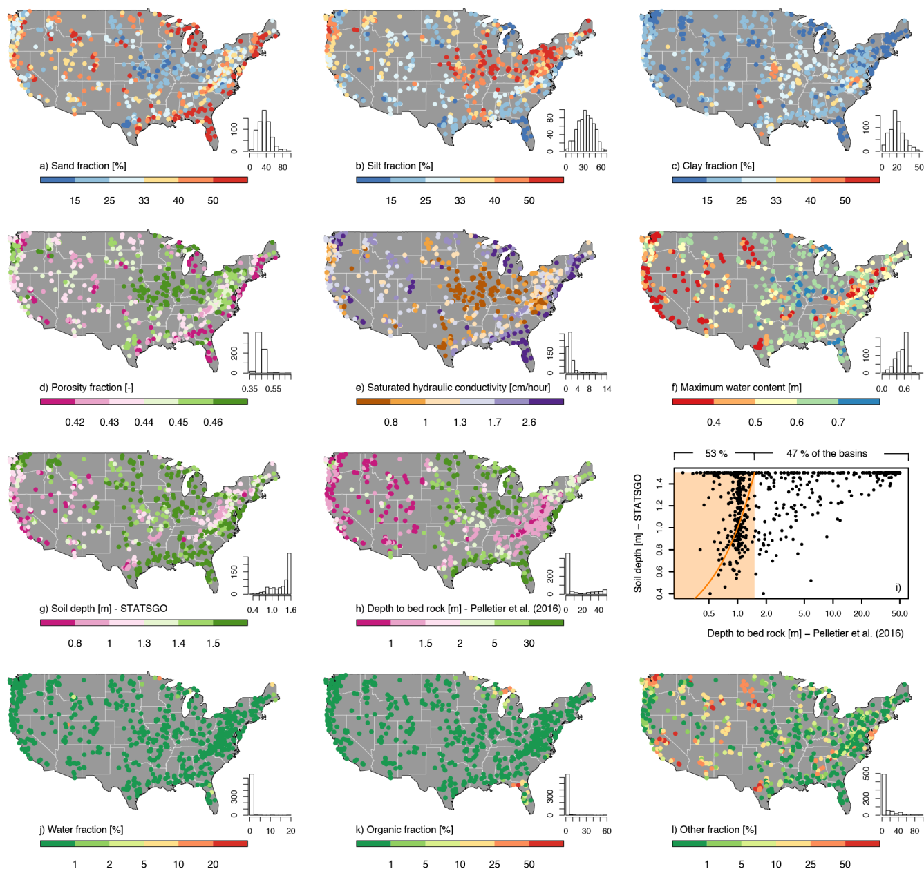
Figure 5: a-h and j-k) Maps of the soil characteristics over the CONUS. The histograms indicate the number of catchments (out of 671) in each bin. i) Comparison of the estimates of the depth to bed rock from STATSGO and P16. The orange area includes all the catchments for which there can be an agreement between the two data sets (i.e. estimates from both data sets are smaller than or equal to 1.5m). The orange curve is a 1:1 curve (note the logarithmic scale on the x-axis).
