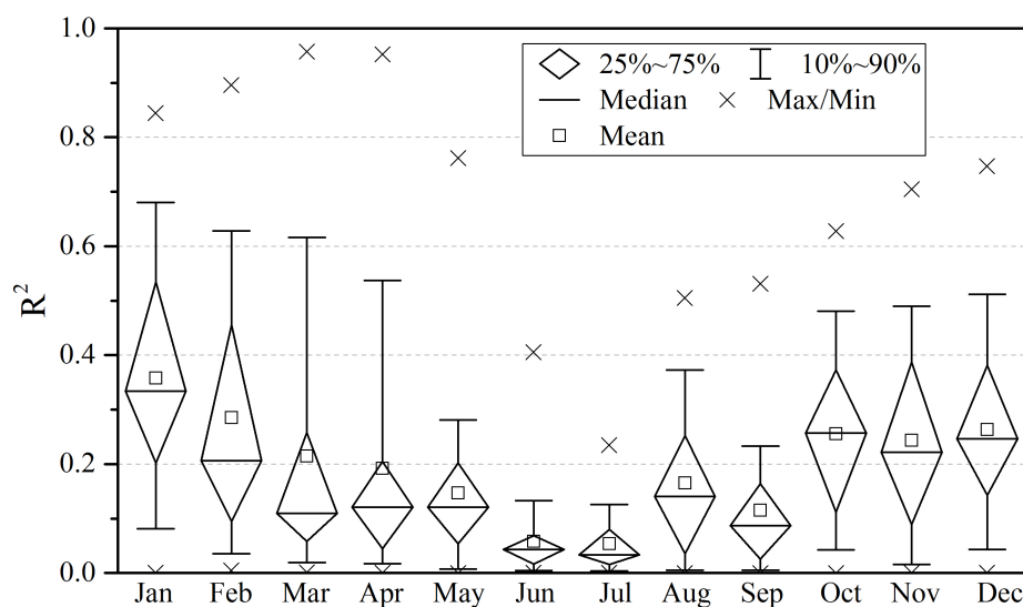
Fig. 1. Figure 5 The box plot of R^2 between monthly ETwb and ETbudyko using the extended Budyko equation, i.e., P-\Delta S as equivalent P , and \Delta S is obtained from abcd model.
