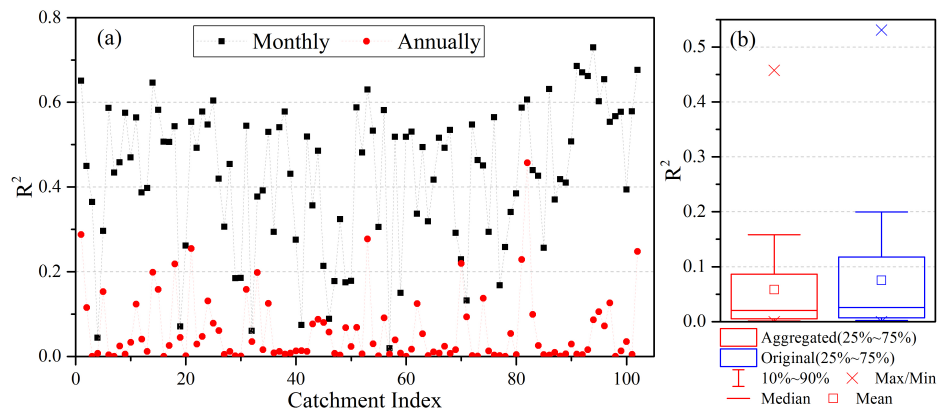
Fig. 2. Figure 6 The R^2 between ETwb and ETBudyko at monthly timescale and that aggregated to annual timescale in (a), and (b) the boxplot of R^2 of this aggregated annual ETBudyko and the original R^2 of annua
