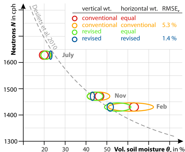
Figure 5. Recalibration of the CRNS sensor in the Sheepdrove Organic Farm (Lambourn, UK) using different combinations of vertically and horizontally weighted averages. Sizes of the circles indicate the corresponding uncertainty range of the measurement. The revised approach clearly removes the bias by the exceptional stripe around the sensor, improving the calibration performance with regards to the widely accepted theoretical relation (dashed).
