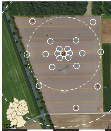
Figure 6. Recalibration of the CRNS sensor in an agricultural maize field (Braunschweig, Germany). Sizes of the circles indicate the corresponding uncertainty range of the measurement, while every such measurement corresponds to a calibration curve \theta(N, N_0) . The conventional weighting approach is not able to provide a single unique theoretical line through the three calibration days and further predicts unrealistic reduction of hydrogen pools during maximum plant height (July) and after harvest (Oct). The revised approach converges the datasets to confirm the accepted neutron theory almost in a single calibration curve within uncertainties (ellipses).
