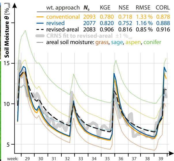
Figure 9. Time series of CRNS and TDT soil moisture at the T.W. Daniel Experimental Forest . The area was split into four categories (dotted lines), to which the corresponding soil moisture measurements were assigned. The areal coverage was then averaged (dashed line) with the revised weighting approach, leading to the best performance against the CRNS signal.
