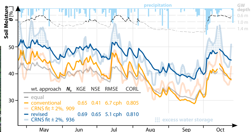
Figure 8. Time series of CRNS soil moisture and ground water at the forested river catchment Wüstebach . Fitting the CRNS data to the SoilNet conventional average almost completely hides effects like litter and interception water, groundwater rise, or ponding close to the stream. The revised approach emphasizes those additional hydrological processes, while still robustly increasing the sensor performance.
