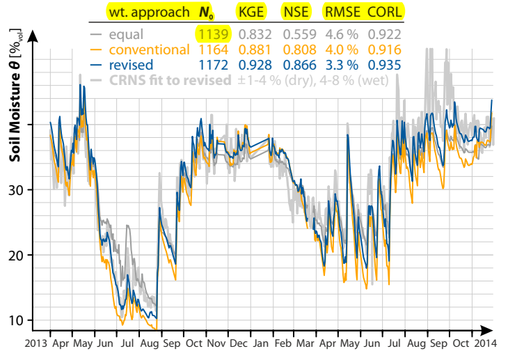
Figure 6. Time series of the CRNS soil moisture data at the SoilNet validation site in Schäfertal (Harz mountains, Germany). The revised weighting approach improves four performance measures, although the SoilNet probes are unevenly distributed in the CRNS footprint. The uncertainty introduced by the insufficient coverage ranges from 1 to 8 % vol depending on wetness conditions.
