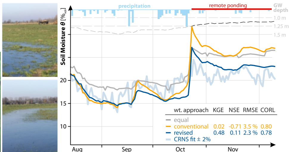
Figure 7. Time series of soil moisture measured in a pasture/floodplain Grosses Bruch . The rain events in mid-October 2014 lead to rise of the groundwater level and ponding in regions that are several tens of meters away from the neutron sensor. In that period, equal and conventional weighting leads to overestimation of apparent soil moisture near the CRNS probe, to which the detector has higher sensitivity than to the remote ponds.
