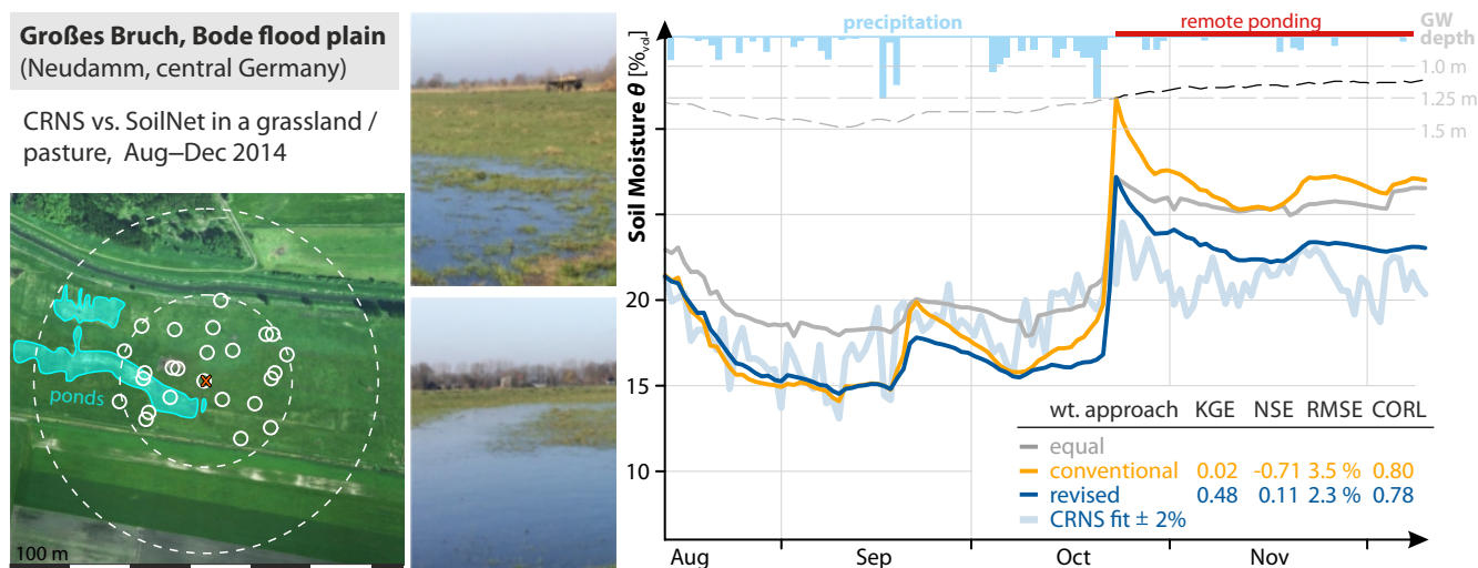
Figure 7. Time series of soil moisture measured in a pasture/floodplain Großes Bruch . The rain events in mid-October 2014 lead to rise of the groundwater level and ponding in regions that are several tens of meters away from the neutron sensor. In that period, equal and conventional weighting leads to overestimation of apparent soil moisture near the CRNS probe, to which the detector has higher sensitivity than to the remote ponds.
