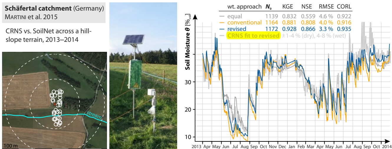
Figure 6. Time series of the CRNS soil moisture data at the SoilNet validation site in Schäferfart (Harz mountains, Germany). The revised weighting approach improves four performance measures , although the SoilNet probes are unevenly distributed in the CRNS footprint. The uncertainty introduced by the insufficient coverage ranges from 1 to 8 % vol depending on wetness conditions.
