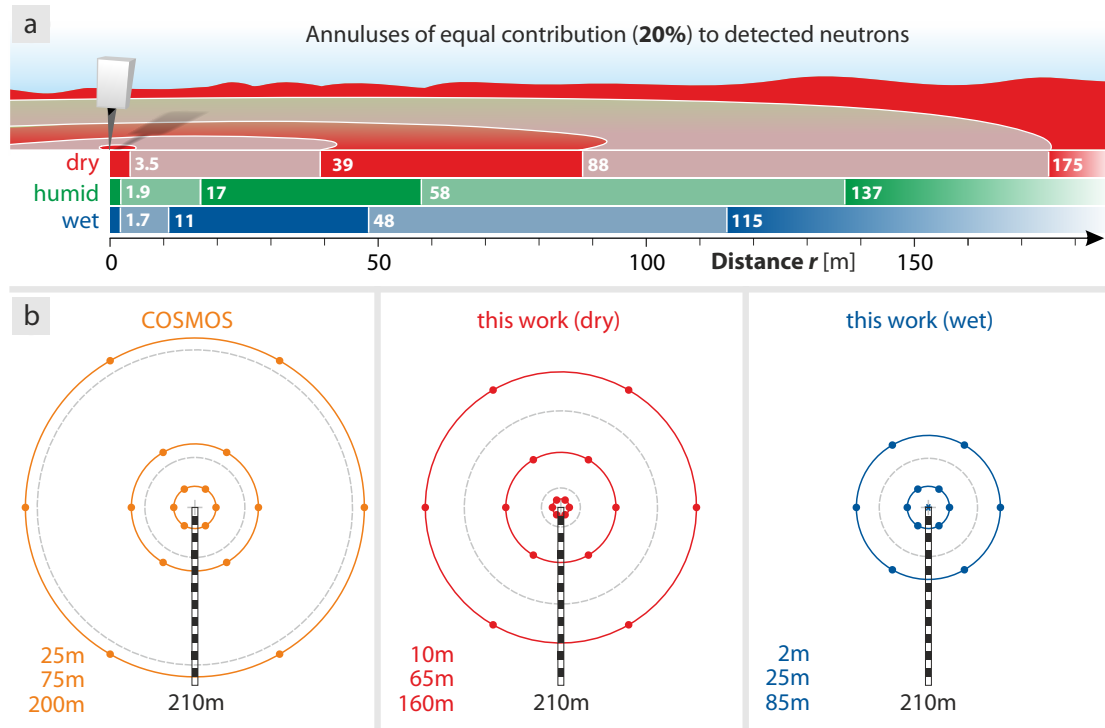
Figure 10. (a) Illustration of regions of equal contribution (20% quantiles) to the neutron signal for three climates, h = \{2, 7, 20\} \text{ g/m}^3 , \theta = \{2, 20, 50\} \% . (b) The COSMOS standard sampling scheme based on W_r^{\text{conv}} , compared to two exemplary 3-radii-schemes based on the revised function W_r^* for dry ( h = 1 \text{ g/m}^3 , \theta = 1 \% ) and wet ( h = 10 \text{ g/m}^3 , \theta = 40 \% ) conditions. Circles represent the borders of the 33% quantiles, r_i (grey, dashed), and arbitrary sampling distances R_i within these annuli (colored, solid).
