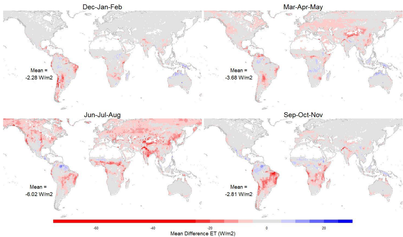
Figure 6: Difference between the seasonal average ET from MPIBGC and DOLCE calculated over the period 2000–2009.
