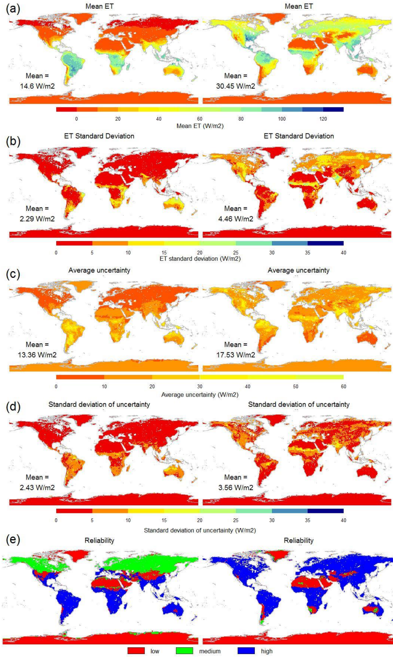
Figure 8: Seasonal (a) global mean ET and (b) its variability (standard deviation), (c) time average of uncertainty (the standard deviation uncertainty \sqrt{\sigma_e^2} shown in Equation 11) (d) standard deviation of uncertainty over time (e) reliability, defined as high ( \frac{Uncertainty\ SD}{mean\ ET} \leq 1 in blue), medium ( |mean\ ET| \leq 5 , Uncertainty\ SD < 10 and \frac{Uncertainty\ SD}{mean\ ET} \geq 1 in green) and low (in red). DJF is shown in the left column and JJA in the right column.
