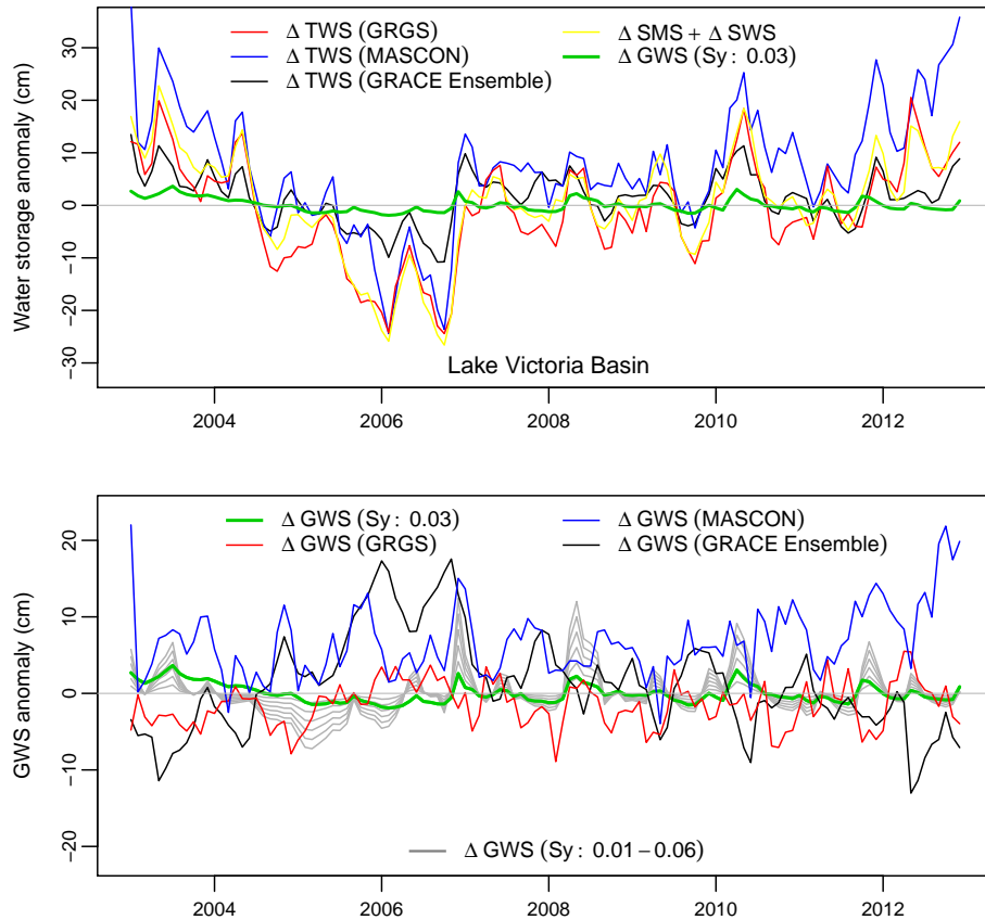
Fig. 1. Figure R1. Time-series records of GRACE \Delta TWS, sum of in-situ \Delta SWS and \Delta SMS, and in-situ \Delta GWS for LVB (top); and estimated \Delta GWS (bottom). Gridded scaling factors applied to GRCTellus and JPL-Mascons.
