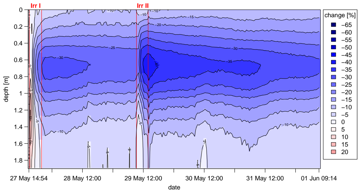
Figure 9. Chronological sequence of resistivity change relating to the initial model of a 1D depth profile 1.5 m downslope of the irrigation area.
