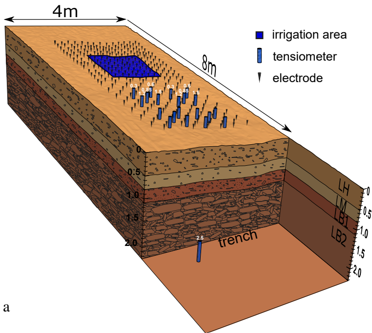
Figure 1. Experimental Setup: a) Schematic overview of subsurface layers (LH, LM, LB1, LB2), with measured electrode and tensiometer positions and irrigation area, b) ERT electrodes, colours marking the three measuring grids.
