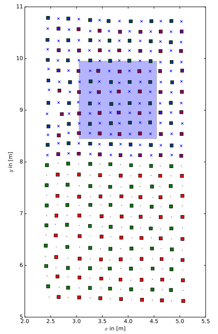
Figure 1. Experimental Setup: a) Schematic overview of subsurface layers (LH, LM, LB1, LB2), with measured electrode and tensiometer positions and irrigation area, b) ERT electrodes, colours marking the three measuring grids.
