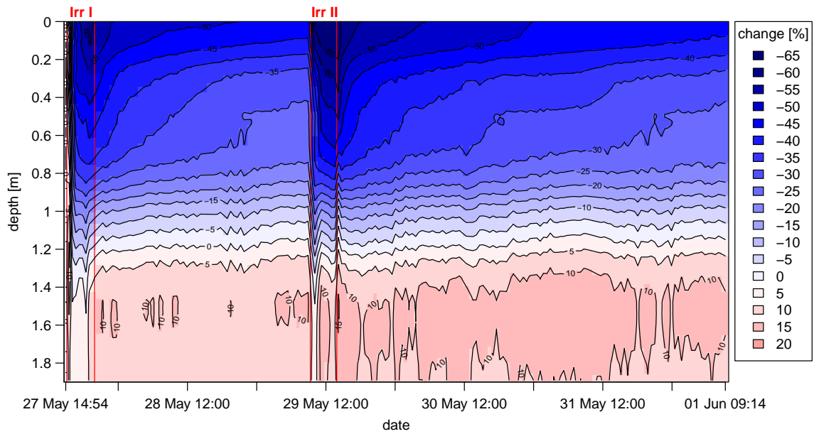
Figure 8. Spatio-temporal distribution-Chronological sequence of resistivity ratio-change relating to the initial model of a 1D depth profile centrally beneath the irrigation area.
