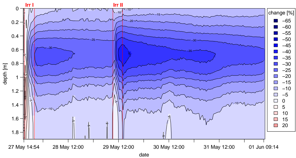
Figure 9. Spatio-temporal distribution-Chronological sequence of resistivity ratio-change relating to the initial model of a 1D depth profile 1.5 m downslope of the irrigation area.
