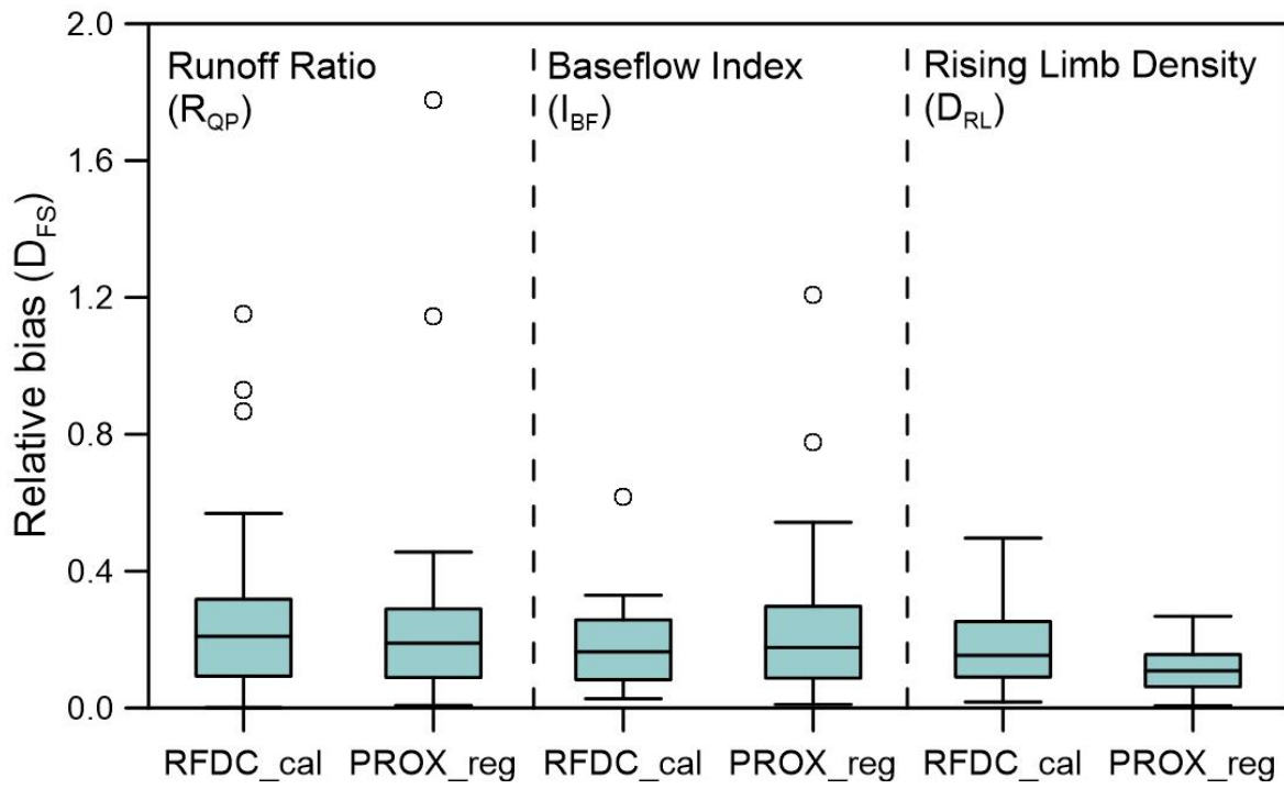
655 Figure 8: Flow signature reproducibility comparison between RFDC_cal and PROX_reg in terms of R_{QP} (a), I_{BF} (b), and D_{RL} (c).
