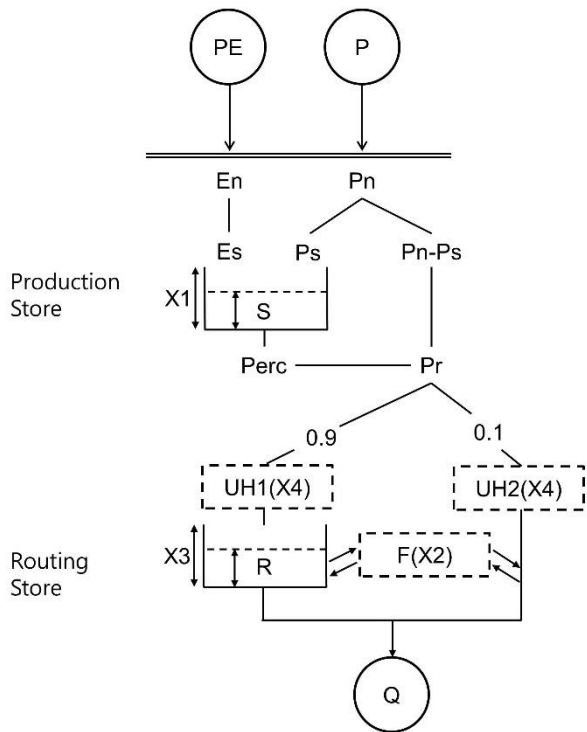
620 Figure 2: The schematised structure of GR4J (X1-X4: model parameters, PE: potential evapotranspiration, P: precipitation, Q: runoff, other letters indicate variables conceptualising internal catchment processes).
