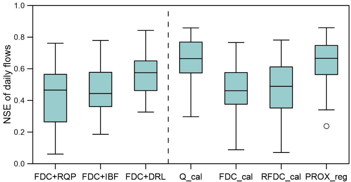
660 Figure 9: Predictive performance of the FDC calibrations additionally conditioned by R_{QP} (FDC+RQP), I_{BF} (FDC+IBF), and D_{RL} (FDC+DRL) in comparison to the other modelling approaches. Q_{cal} and FDC_{cal} refer to the hydrograph and the FDC calibration in gauged catchments respectively. 38 catchments with positive NSEs for all the modelling approaches were used in the box-plots.
