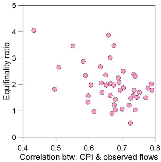
650 Figure 7: The input-output consistency vs. equifinality increased by replacing the hydrograph calibration with the FDC calibration. The equifinality ratio is defined as the ratio between the prediction areas of the 50 behavioural parameters gained from the FDC calibration and the hydrograph calibration.
