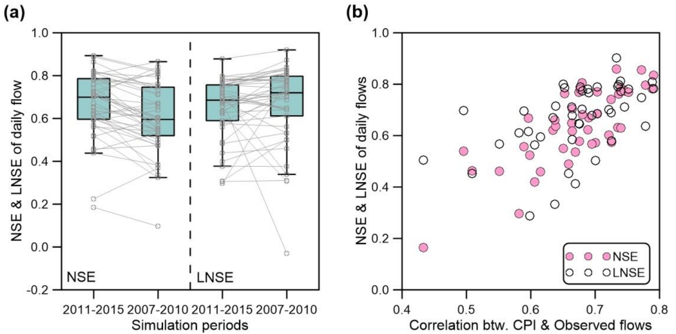
625 Figure 3: (a) box plots of high flow (NSE) and low flow (LNSE) reproducibility of the behavioural parameters obtained from the hydrograph calibration at the 45 catchments, (b) the relationship between the input-output consistency and the model performance. The straight lines in the box plots connect the performance metrics for the calibration (2011-2015) and the validation periods (2007-2010) in each catchment.
