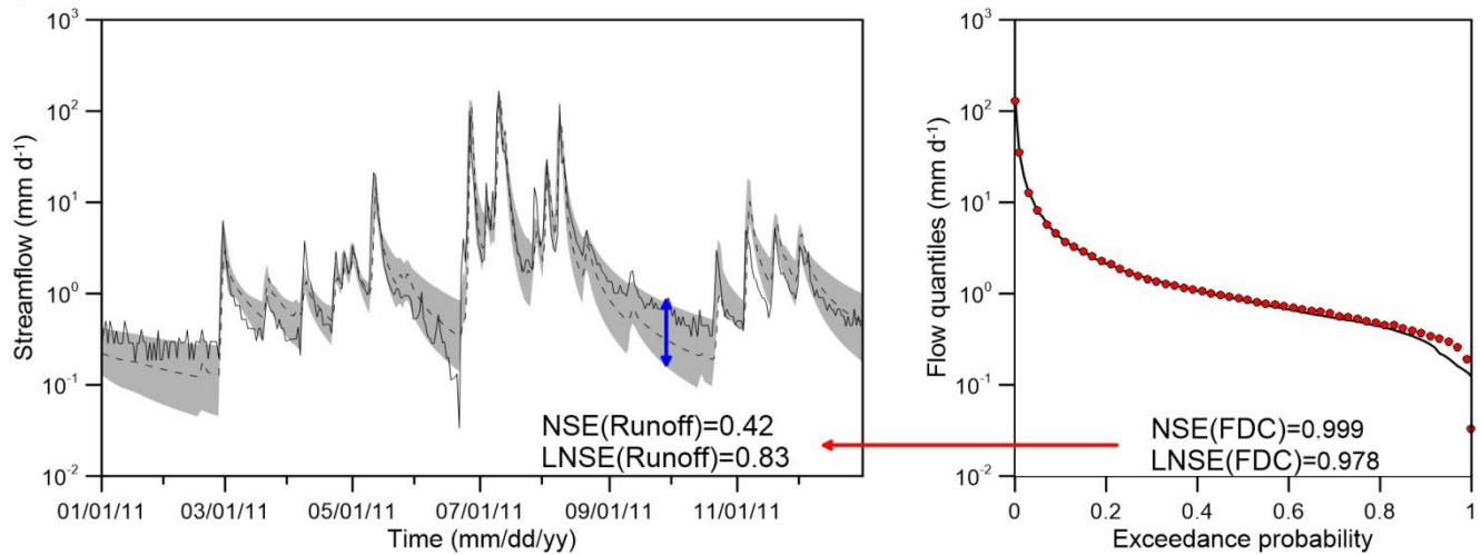
645 Figure 6: The observed and predicted hydrographs, the prediction areas, and the observed and predicted FDCs given by (a) the hydrograph calibration and (b) the FDC calibration for the Catchment 2.
