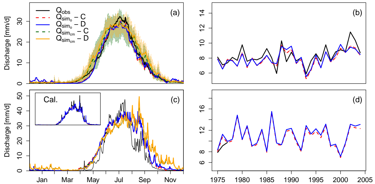
Figure 3. Discharge comparisons in the historical period. The hydrological regime (a and c) and annual discharges (b and d) are shown for Nigardsbreen catchment (a and b) and for Wolverine (c and d). Observed discharge is compared with both ( Q_{sim_o} ) and ( Q_{sim_{cm}} ) for both glacier model conceptualisations. The coloured areas in panel A indicate the range of discharge outputs as a result of the different climate models forcing. The results are shown for the historical period (1975-2004). Note that ( Q_{sim_{cm}} ) is not shown in the inter-annual variability graphs because climate models only statistically represent historic climate and that observed discharge for the Wolverine catchment was only available for 1975-1977. The inset in c shows the agreement between Q_{obs} and Q_{sim_o} for the Wolverine catchment during the calibration period
