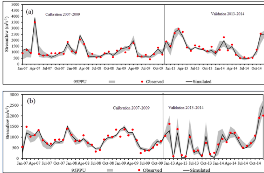
Figure 5. Observed vs. simulated streamflow and 95% uncertainty interval (95PPU) of behavioral simulations over time (defined as simulations with Nash-Sutcliffe efficiency NSE > 0.5) for the BH (a) and MT (b) watersheds respectively.
