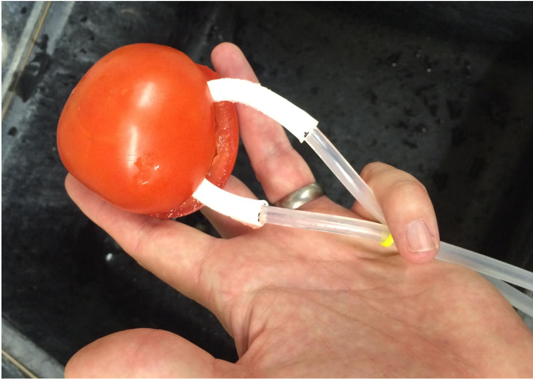
Figure 2. Photograph of membrane-inlet probe (opaque white tubing) partially inserted into a tomato.
