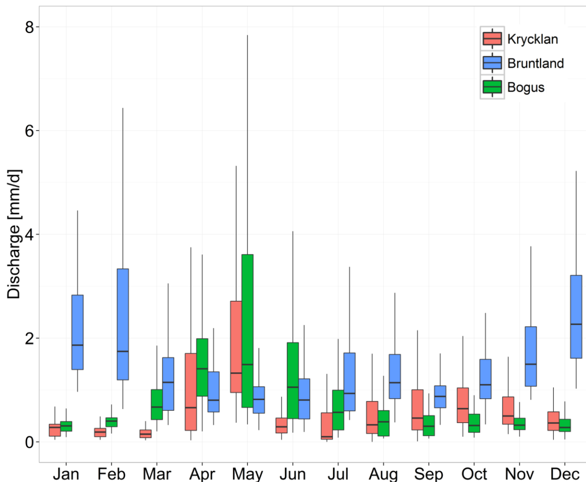
5 Fig. 2. Boxplots showing the seasonality of streamflow for each catchment by grouping daily streamflow (5 years of data for Bruntland, 8 for Bogus and 10 for Krycklan) to monthly bins. Coloured box shows the 25 th and 75 th quantiles, small horizontal line the median and vertical line the extent of 5 th and 95 th percentiles. High flows for Krycklan and Bogus are brought about by snowmelt occurring typically in April-May. For Bruntland flows are more evenly distributed through the year with highest flow during December-February with occasional snowmelt influence.
