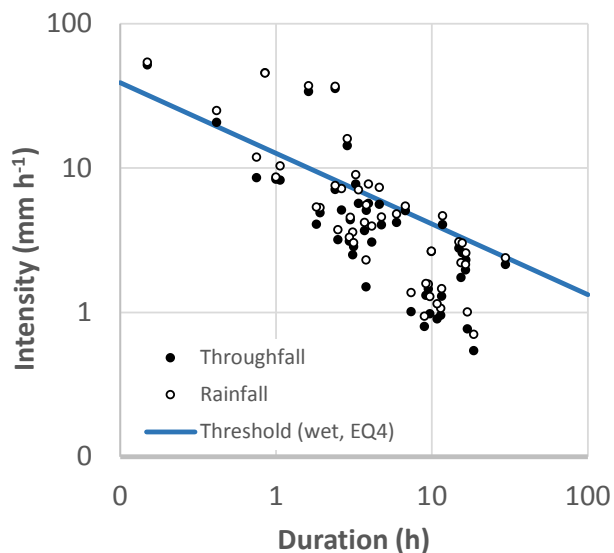
(c) \text{API}_2 > 20 \text{ mm} (wet)
