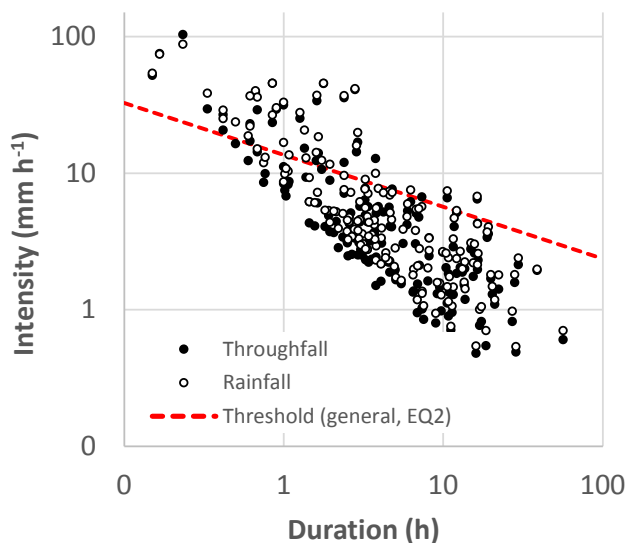
(c) \text{API}_2 > 20 \text{ mm} (wet)
