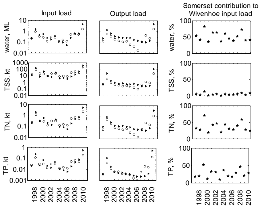
Figure 3: Annual input and output loads of water ( \text{ML y}^{-1} ), TSS and nutrients ( \text{kt y}^{-1} ) for Somerset (o) and Wivenhoe (▶) reservoirs for water years 1997-2010, and the percentage contribution of Somerset to Wivenhoe input loads.
