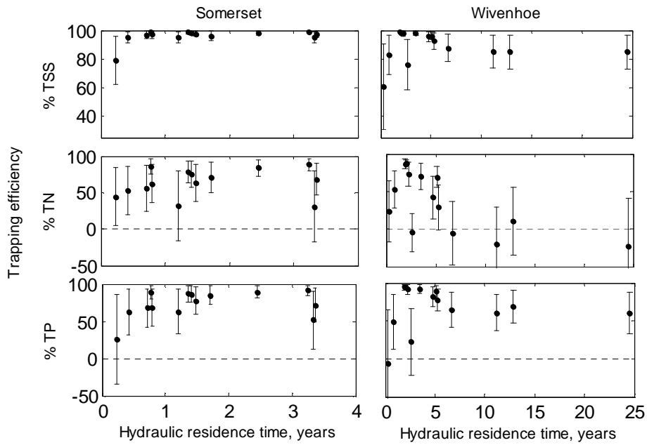
1 2 Figure 7: Percentage of annual TSS, TN and TP loads retained in Somerset and Wivenhoe reservoirs compared to hydraulic 3 residence time (y). Dashed line indicates zero trapping, boundary between net positive import and export.
