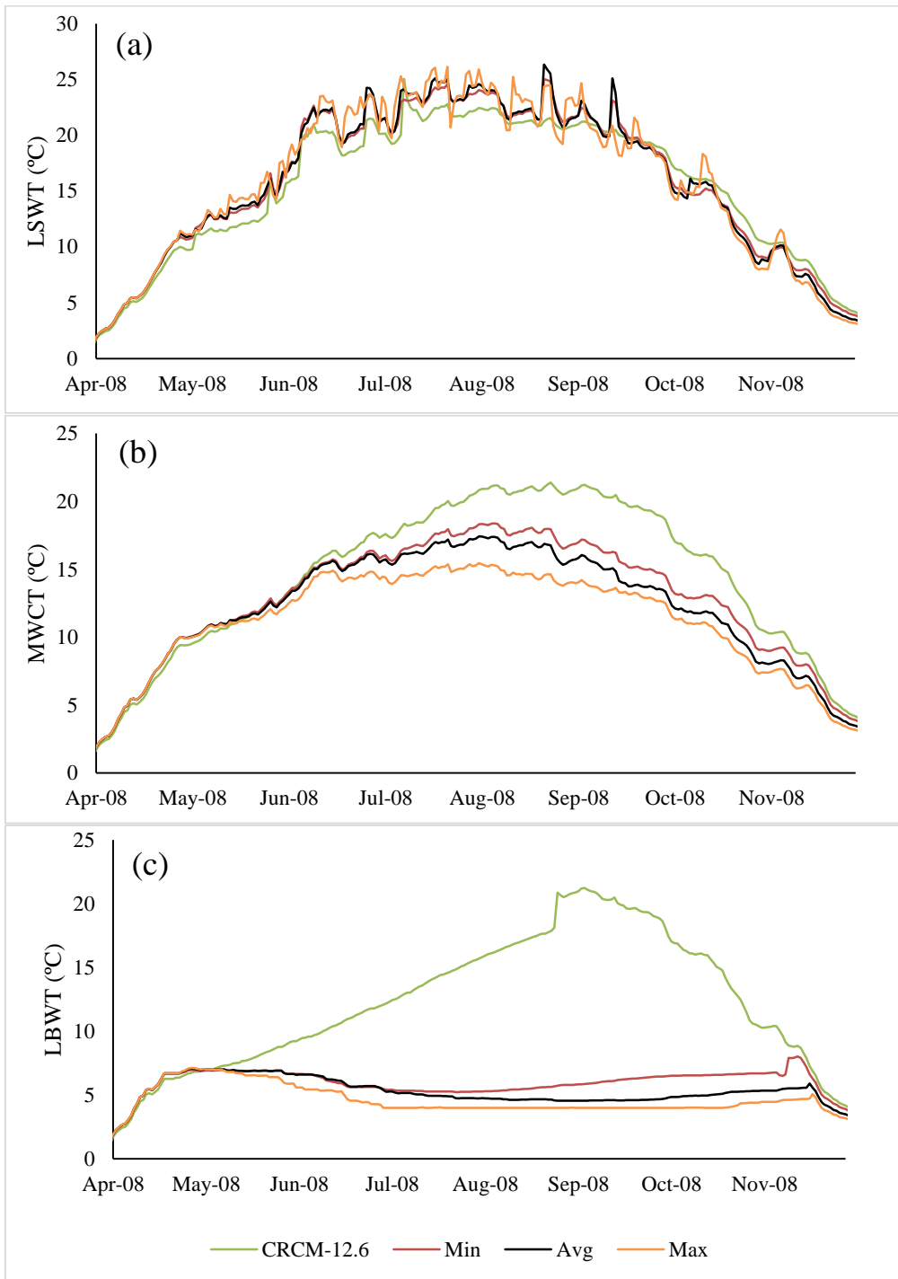
Fig. 11 LSWT (a), MWCT (b), and LBWT (c) simulation results in 2008 for CRCM-12.6 simulation and the lowest (Min), average (Avg), and the highest (Max) K_d values are shown.
