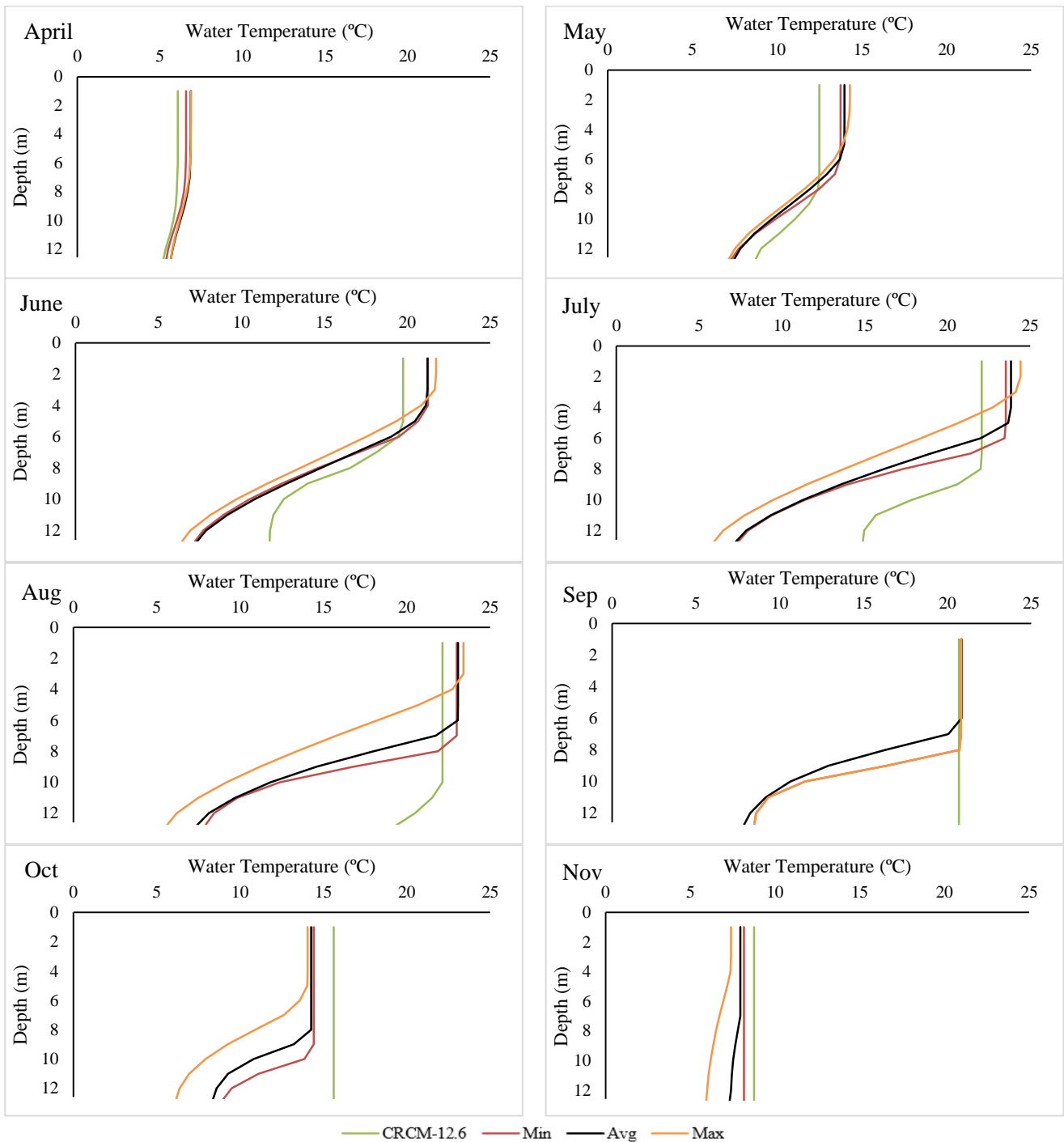
Fig. 14 Monthly average temperature profile in 2008 for CRCM-12.6 simulation and the lowest (Min), average (Avg), and the highest (Max) K_d values are shown.
