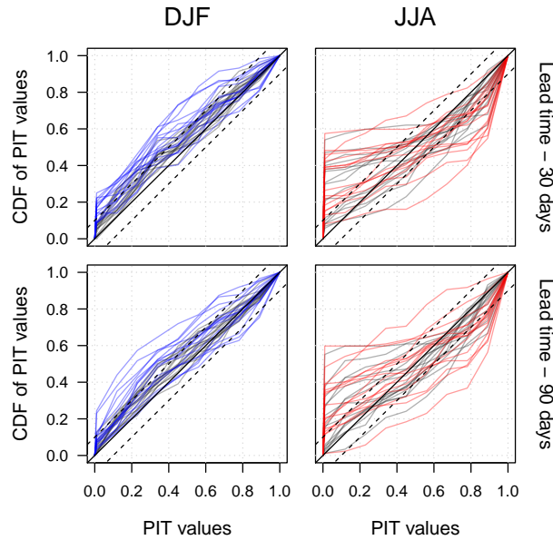
Figure 5. PIT diagram of streamflow forecasts from raw precipitation forecasts (coloured lines) and Ensemble Streamflow Prediction (grey lines) for lead times of 30 days (top) and 90 days (bottom). Each column corresponds to a target season. Each line represents the PIT diagram in a catchment for forecast horizons within the target season. Dotted lines represent the Kolmogorov-significance \pm 1 tolerance bands for a 5% significance test from the diagonal.
