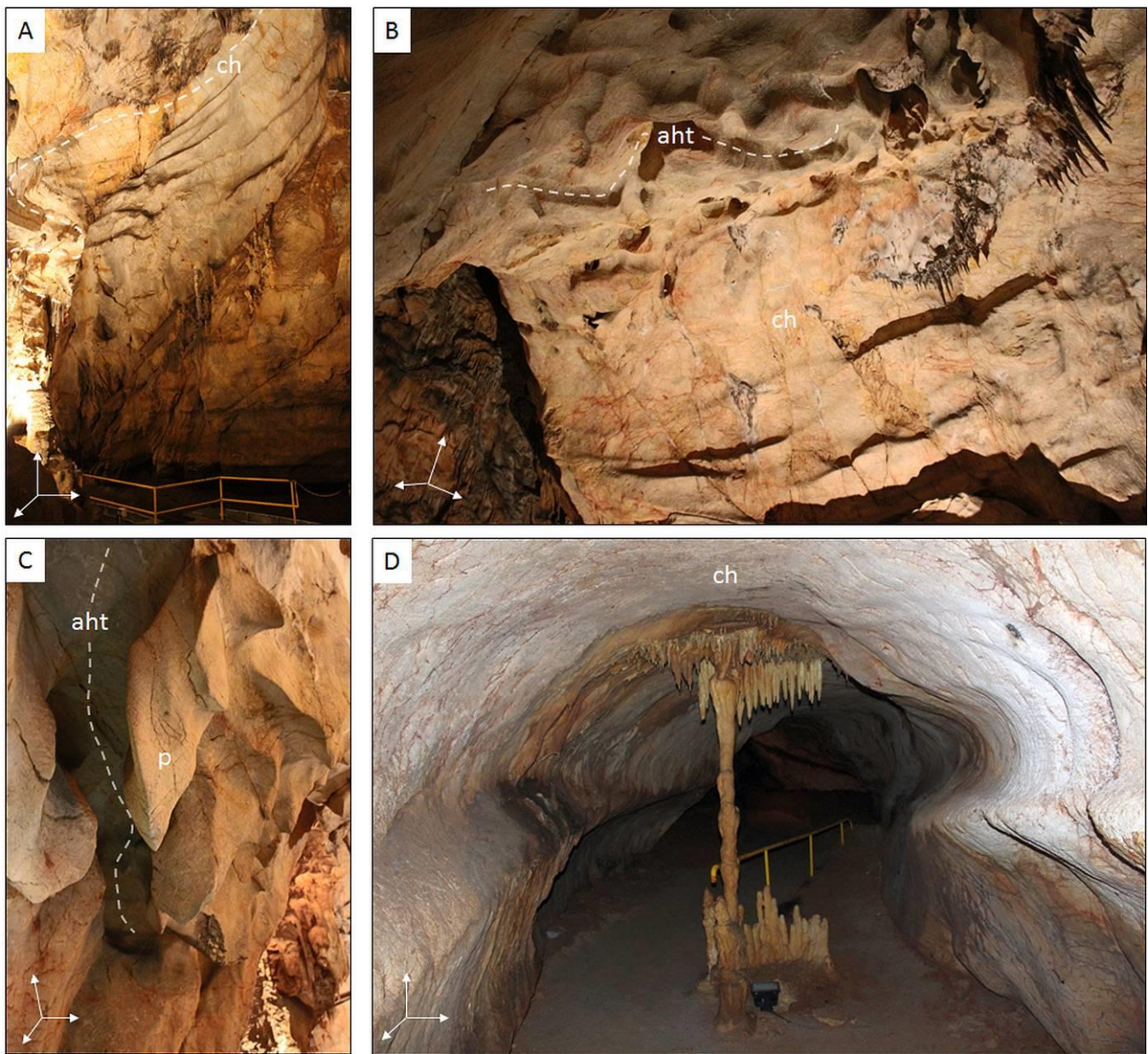
Fig. 2. Examples of ceiling channels (ch), pendants (p), and anastomosing half tubes (aht) in the Domica cave as speleothems associated with the phreatic regime. Presence of the speleothems in the ceiling and walls of the Gothic Dome indicate paragenetic (antigravitational) development (A, B, C), while it is more difficult to infer from the Dry passage (D) from where much of the accumulated sediment was not evacuated and the passage was reshaped during multiple phases of vadose and phreatic conditions. The highest parts of the channels can be situated as high as 16 metres (A, B) or 2 metres above the floor on sediment accumulation (D).
