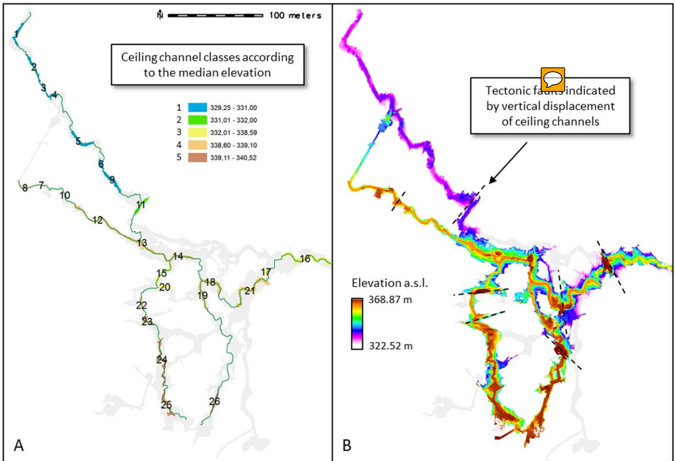
Fig. 10. Ceiling channels resulting from the semi-automatic classification of the Domica ceiling grouped according to their median elevation (A) reported in Tab. 6 and interpretation of their vertical displacement (B).
