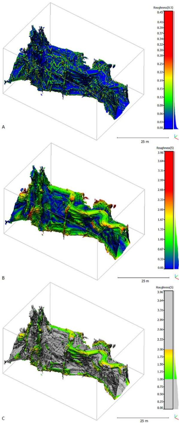
Fig. 16. Roughness of the 3D cave surface model in the Gothic Dome derived at 0.5 m scale (A), and 5 m scale (B), and selection of speleoforms having values between 1 and 2 (C), respectively.
