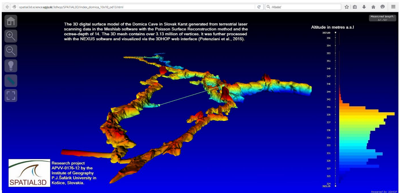
Fig. 17. Print-screen snapshot of the web-interface allowing for interactive viewing and basic measurements of the 3D surface model of the Domica cave.
