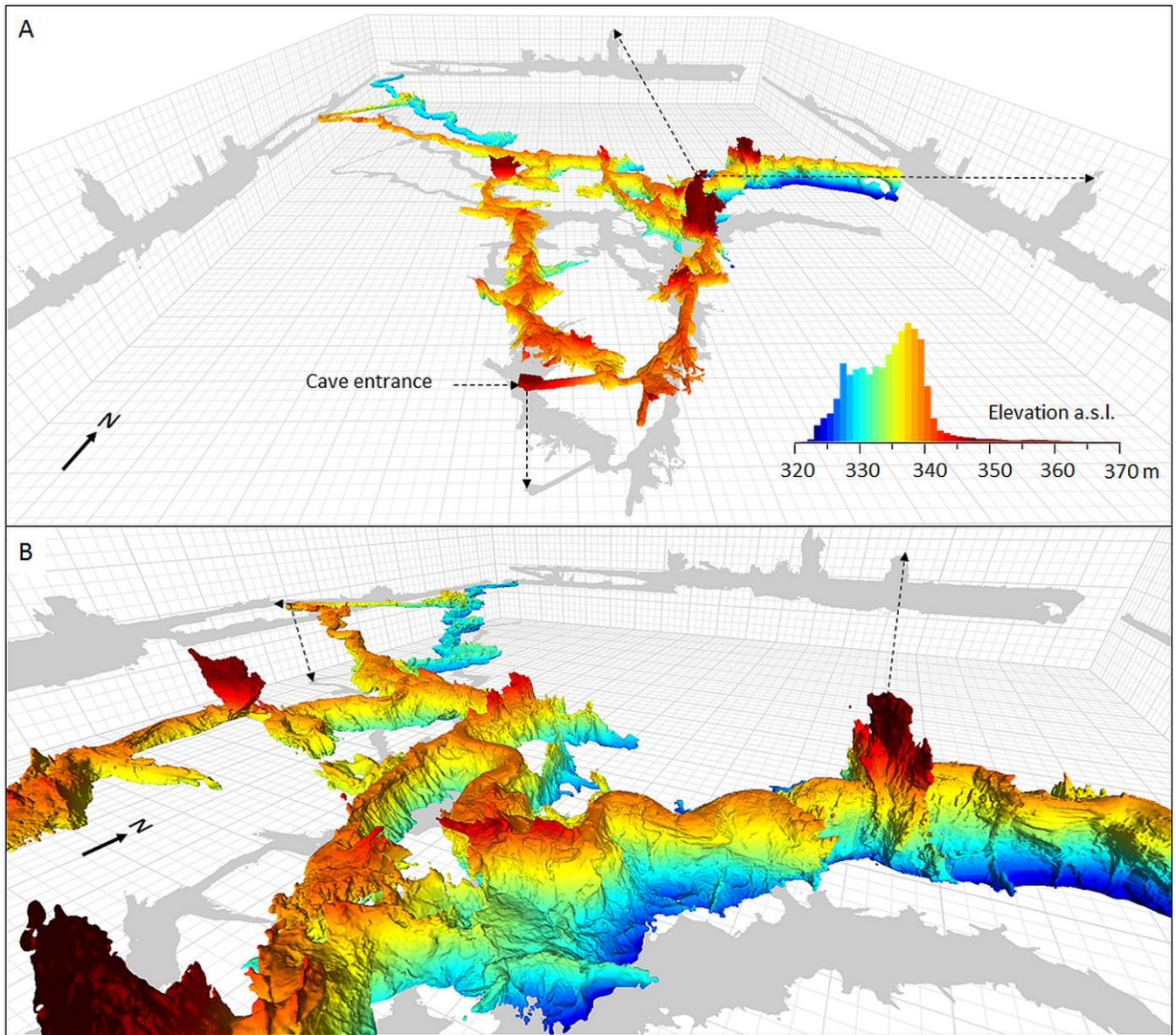
Fig. 5. 3D model of the Domica cave oriented towards north (A) and its detailed view towards north-west (B) showing a meandering ceiling channel. The model is coloured by the value of altitude above mean sea level which distribution is shown by the histogram. The 3D geometry is orthogonally projected on the XY, YZ, and XZ planes. The size of the major and minor cells in the background grid is 20 m and 5 m along all three axes, respectively. Note the flat, horizontal ceiling levels projected on the vertical XZ and YZ planes.
