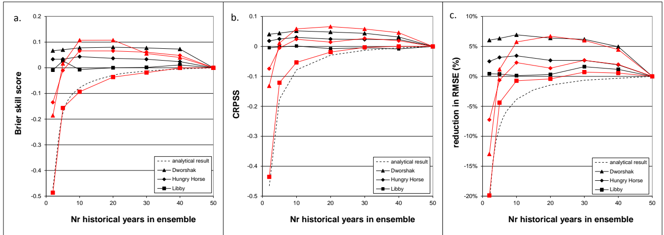
20 Figure 7: Forecast skill of the subsampler method (in red) compared to subsampler-resampler method (in black) as a function of number of historical ESP ensemble traces. a. Brier Skill Score (80% threshold) b. CRPSS and c. relative reduction of RMSE. Skill scores are averaged over 50 years of hindcasts for May and June monthly streamflow at lead times between 3 and 12 months.
