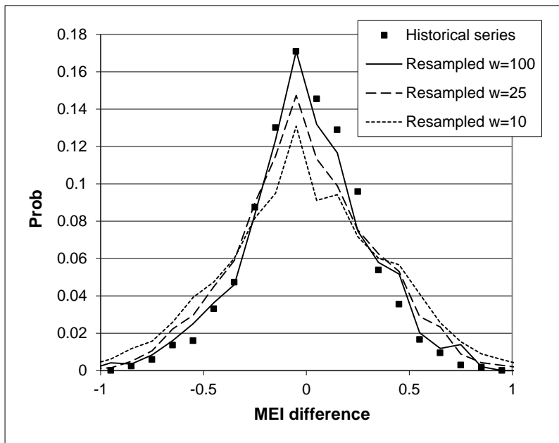
Figure 3: Distribution of MEI differences between consecutive months; historical series and three resampled time series with w -values of 10, 25 and 100.
