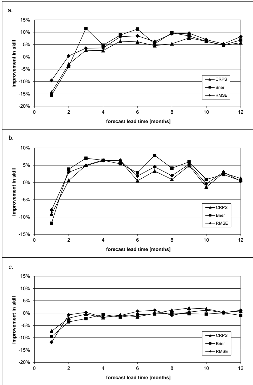
5 Figure 8: Improvement in May/June streamflow forecast skill of the subsampler-resampler ( w=25 ) method relative to the standard ESP as a function of lead time for: a: Dworshak, b: Hungry Horse, c: Libby test stations. Three different skill metrics: CRPS, Brier Score and RMSE.
