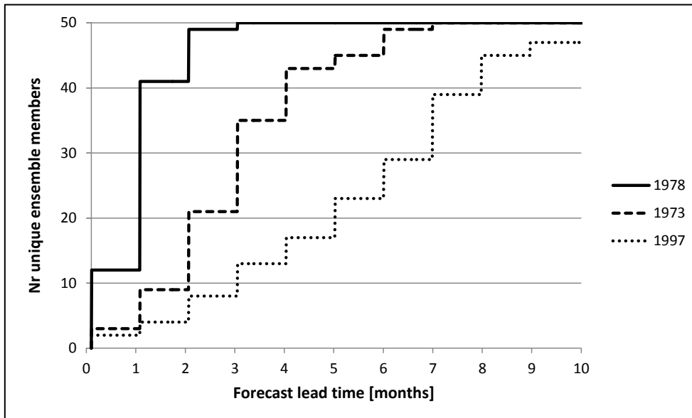
Figure 6: Number of unique ensemble traces in 50-member ensembles of resampled time series ( w=25 ), starting from December 1st, 1978, 1973 and 1997.
