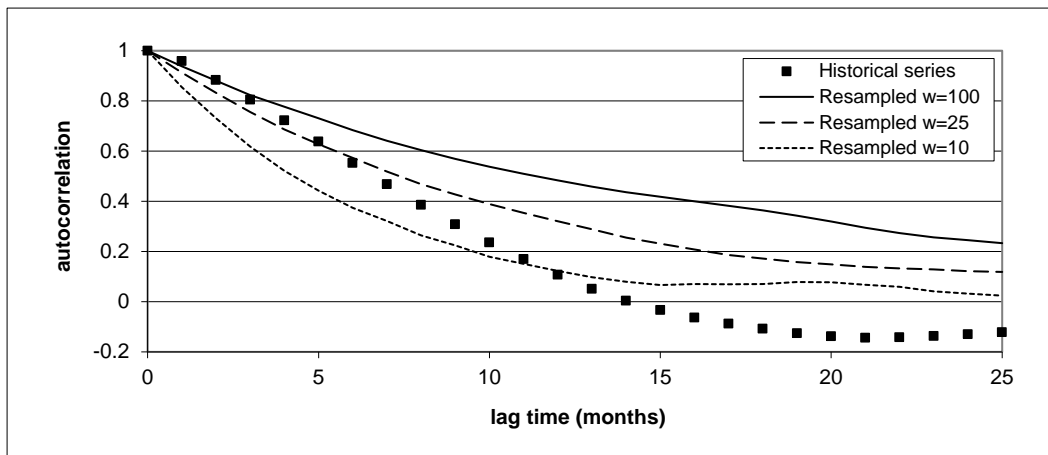
5 Figure 4: Autocorrelation of MEI signal for the historical and three resampled time series with w -values of 10, 25 and 100.
