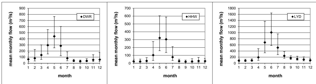
Figure 2: Median monthly streamflow and 10% and 90% percentiles for the test-basins Dworshak (DWR), Hungry Horse (HHW) and Libby (LYD).
