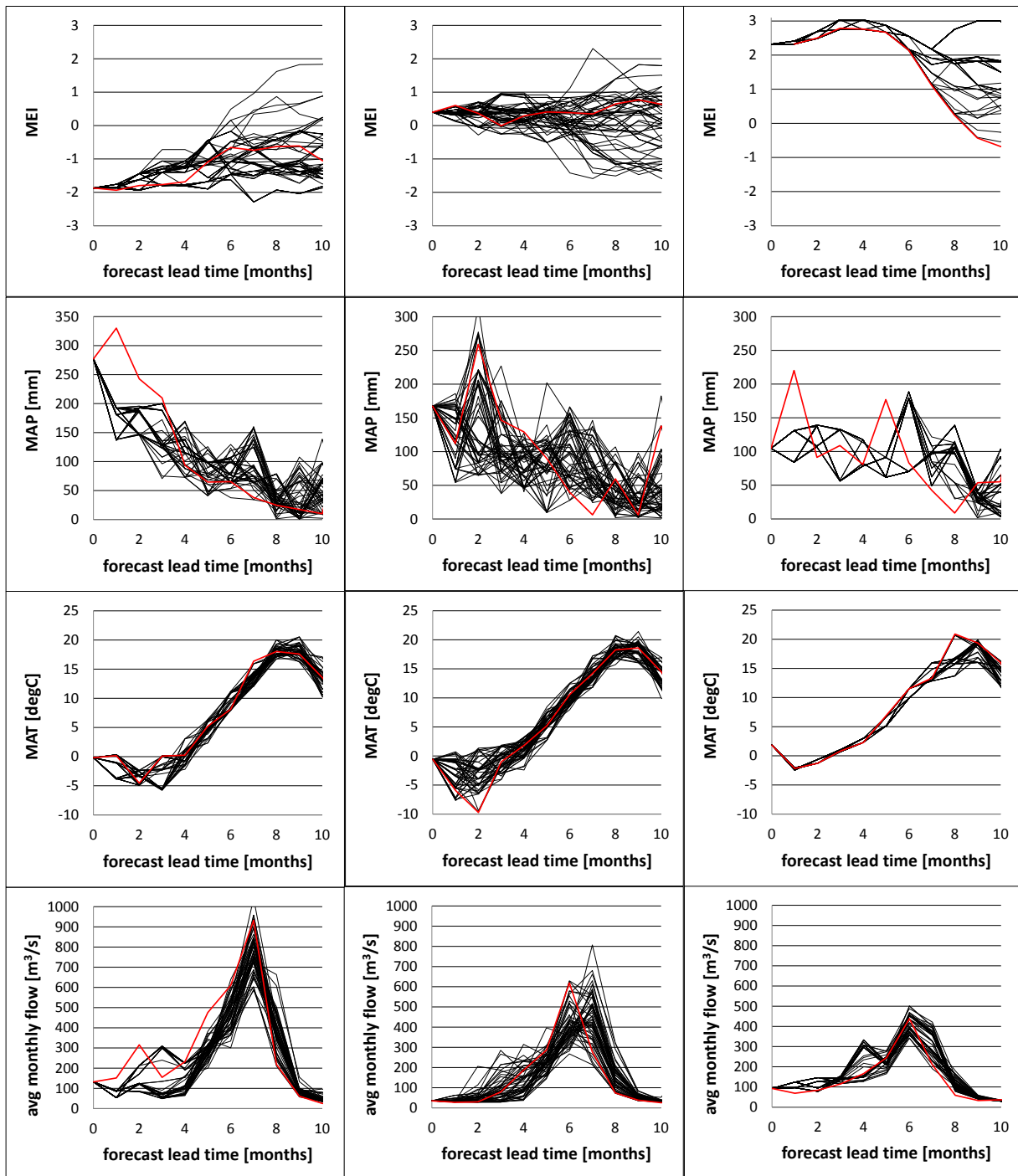
Figure 5: Resampled ensemble forecasts of (from top to bottom) MEI, MAP, MAT and streamflow at test location Dworshak. Forecast dates are December 1st 1973 (left), 1978 (middle) and 1997 (right). The historical runs are shown in red.
