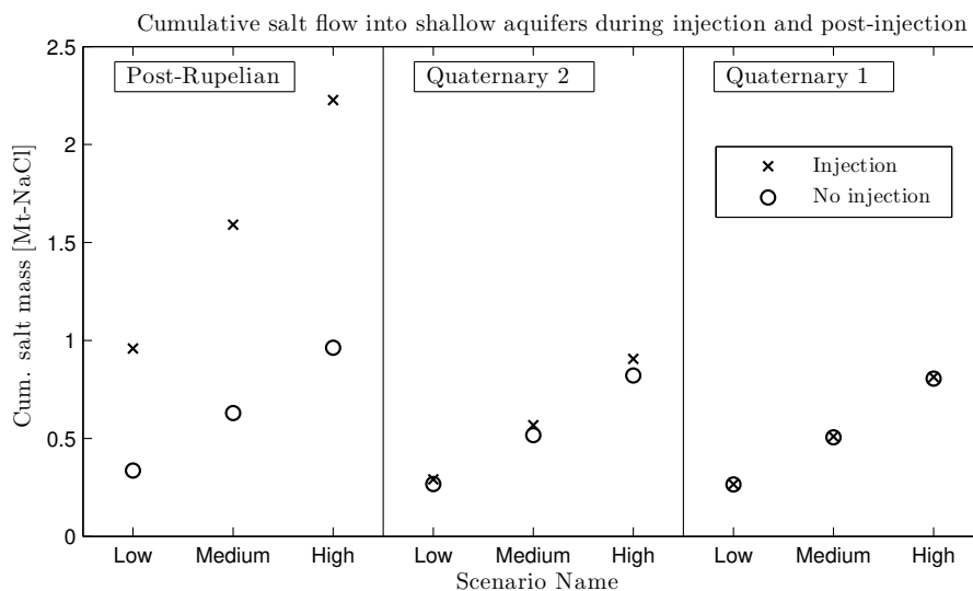
Figure 10. The cumulative salt flow for a period of 100 years (injection + post-injection) into the Tertiary Post-Rupelian, the Quaternary 2, and the Quaternary 1 each for the low, medium, and high scenario. The crosses correspond to simulations with injection, whereas the circles correspond to cases without injection, i.e. only the salt base flow.
