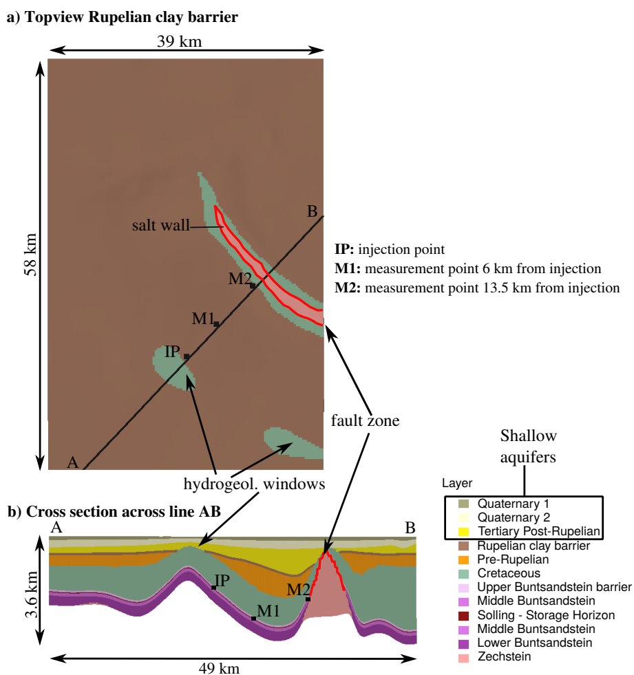
Figure 7. a) Top view on the Rupelian clay barrier. Also shown are the two hydrogeological windows in the Rupelian clay barrier layer and the salt wall piercing through the barrier layer. The fault zone is highlighted in red. b) shows a cross section (vertical exaggeration 4:1) across line A-B with approximate locations of the injection point (IP) and the two measurement points for pressure (M1 and M2).
