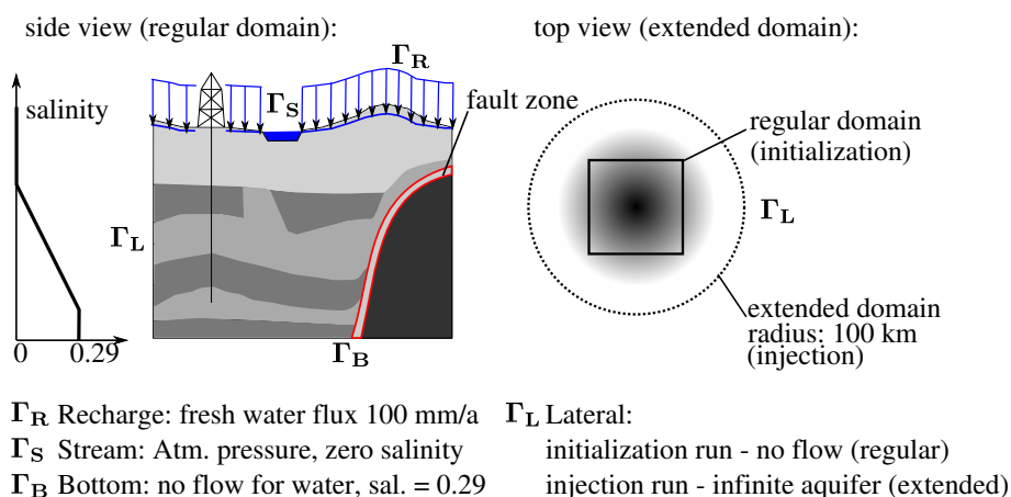
Figure 5. Boundary and initial conditions of the domain shown through a simplified sketch of the geological model. A linear salinity profile increasing with depth up to a maximum salinity (salt mass fraction) of 0.29 \text{ kg kg}^{-1} is assumed as an initial condition for the initialization run. Also shown is the position of the fault zone situated at the flank of the salt wall in red.
