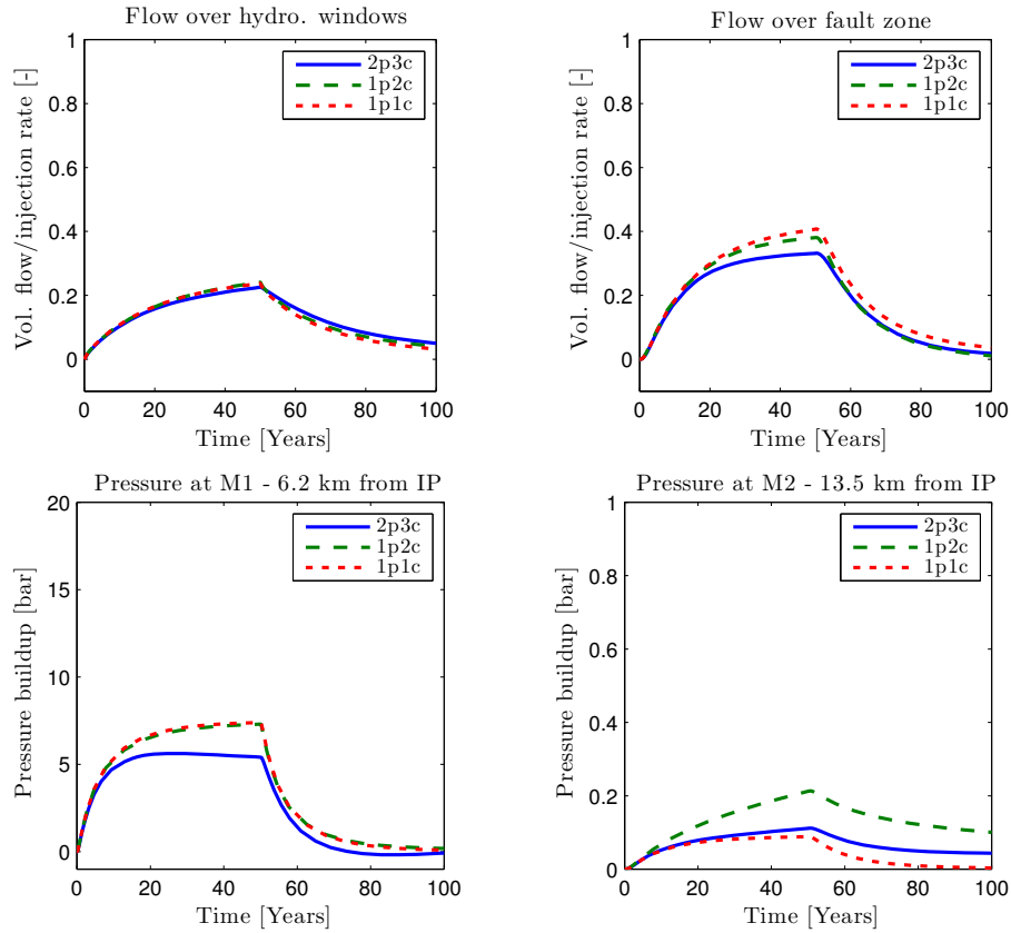
Figure 16. High diffuse migration over barrier (Upper Buntsandstein barrier permeability 1 \cdot 10^{-18} \text{ m}^2 ). Top row: Volumetric flow over the hydrogeological windows and the fault zone. Bottom row: Pressure buildup at measurement points M1 and M2.
