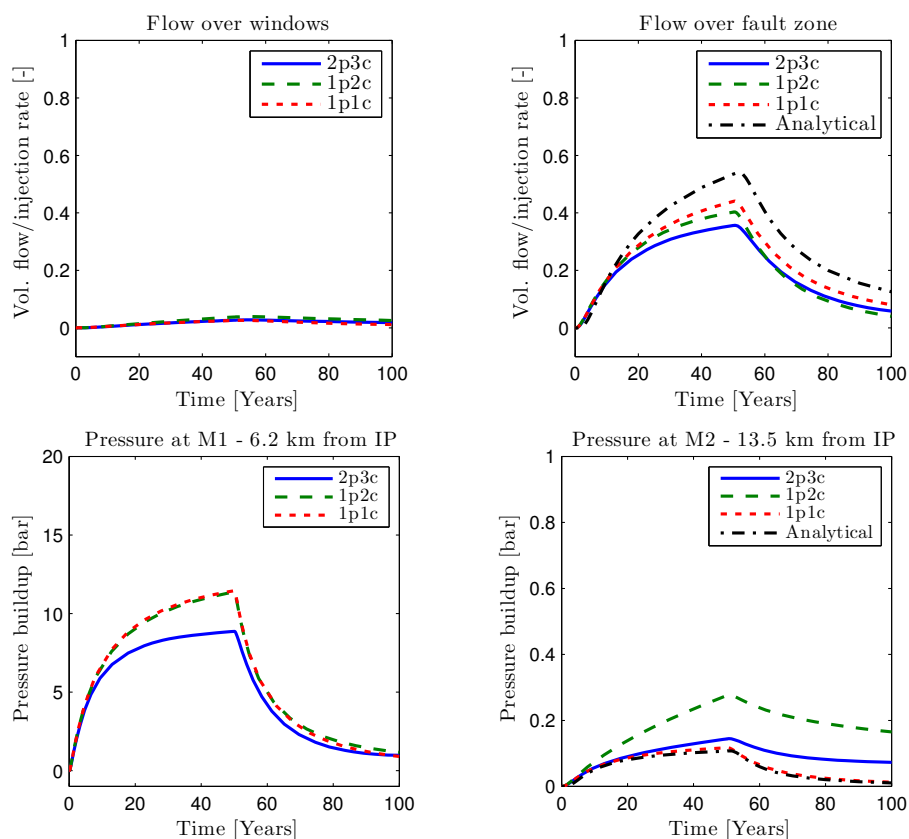
Figure 14. Results for the focused leakage scenario (Upper Buntsandstein barrier permeability 1 \cdot 10^{-20} \text{ m}^2 ). Top row: Volumetric flow over the hydrogeological windows and the fault zone. Bottom row: Pressure buildup at measurement points M1 and M2 in the injection horizon. Note, there are no results for the Analytical Model for the top left plot as the Analytical Model only accounts for flow over the fault zone. Additionally, only the pressure at the fault zone can be determined with the Analytical Model used here.
