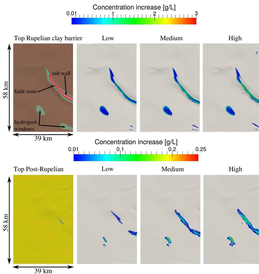
Figure 9. Top row: View on top of the Rupelian clay barrier. The top left figure shows the top view on the geology (as shown in Fig. 7 a). The three figures on the right show the salt concentration increase after 50 years of injection, for the three different scenarios Low, Medium and High with increasing initial salt gradients. Concentration increases below 0.01 g/L are not shown. Bottom row: View on top of the Post-Rupelian. The bottom left figure shows the top view on the geology of the Post-Rupelian. The three figures on the right show the salt concentration increase after 50 years of injection, again for the same three scenarios. Note the different scales on the legends for the top and bottom row.
