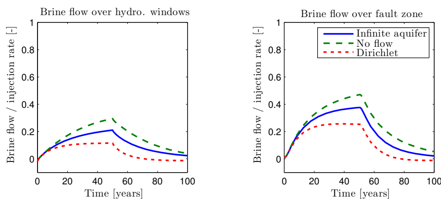
Figure 11. Left: brine flow over hydrogeological windows into the shallow aquifers (normalized by the injection rate). Right: brine flow over fault zone into the shallow aquifers.
