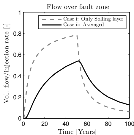
Figure 15. Results of the Analytical Model for the two cases: (i) the injection horizon comprises only the Solling sandstone layer and (ii) the injection horizon comprises all layers in the Middle and Lower Buntsandstein with an averaged injection horizon permeability and porosity.
