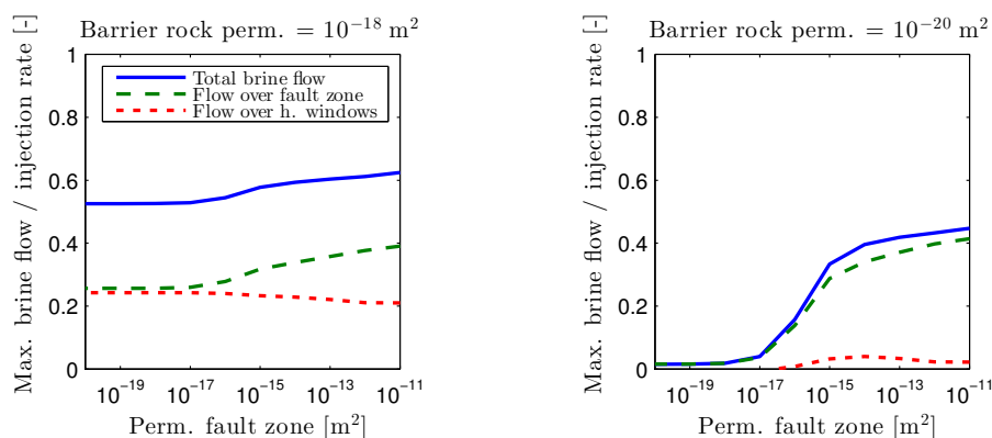
Figure 13. Maximum brine flow into the shallow aquifers reached after 50 years of injection (normalized by the injection rate) over the fault zone permeability. Left: high Upper Buntsandstein barrier permeability, high diffuse migration through barrier; right: low Upper Buntsandstein barrier permeability, high focused migration through fault zone.
