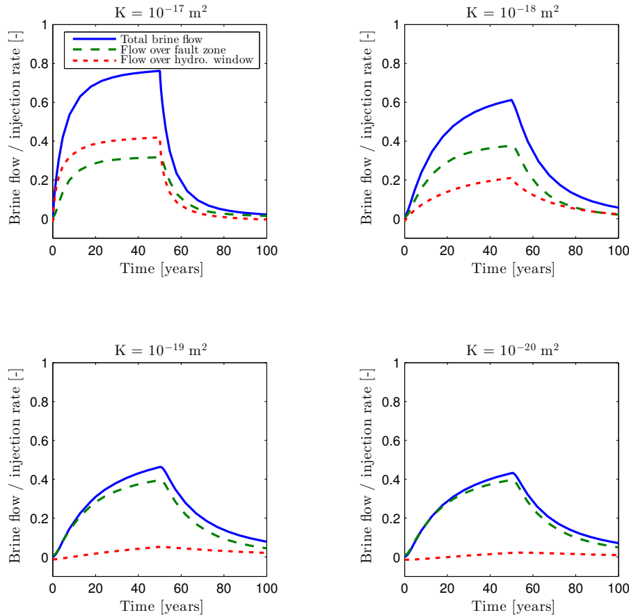
Figure 12. Brine flow normalized by the brine injection rate into the shallow aquifers, for different permeabilities of the Upper Buntsandstein barrier. The upper right scenario with a permeability of 1 \cdot 10^{-18} \text{ m}^2 corresponds to the reference case.
