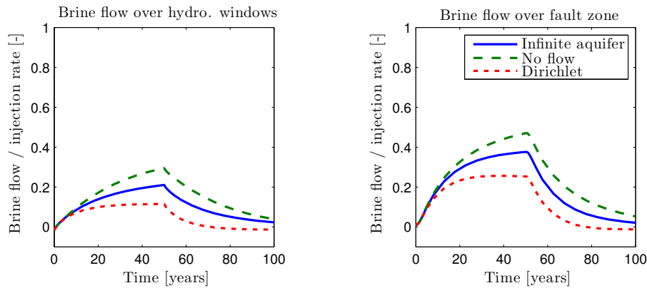
Figure 11. Scenario study 2 – Boundary conditions. Left: brine flow over hydrogeological windows into the shallow aquifers (normalized by the injection rate). Right: brine flow over fault zone into the shallow aquifers.
