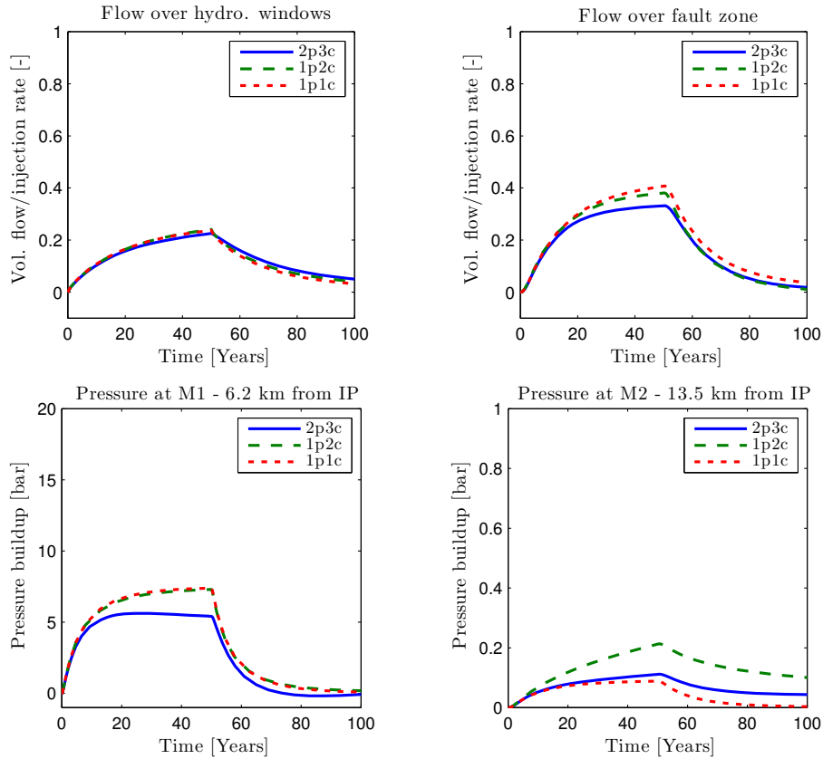
Figure 16. Diffuse leakage scenario – High diffuse migration over barrier (Upper Buntsandstein barrier permeability 1 \cdot 10^{-18} \text{ m}^2 ). Top row: Volumetric flow over the hydrogeological windows and the fault zone. Bottom row: Pressure buildup at measurement points M1 and M2.
