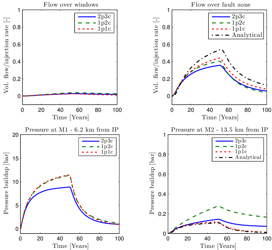
Figure 14. Focused leakage scenario – Results for the focused leakage scenario (Upper Buntsandstein barrier permeability 1 \cdot 10^{-20} \text{ m}^2 ). Top row: Volumetric flow over the hydrogeological windows and the fault zone. Bottom row: Pressure buildup at measurement points M1 and M2 in the injection horizon. Note, there are no results for the Analytical Model for the top left plot as the Analytical Model only accounts for flow over the fault zone. Additionally, only the pressure at the fault zone can be determined with the Analytical Model used here.
