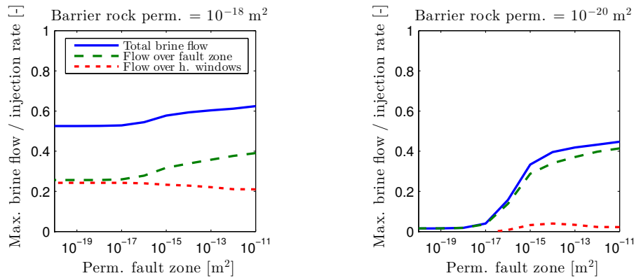
Figure 13. Scenario study 4 – Variable fault zone transmissivity. Maximum brine flow into the shallow aquifers reached after 50 years of injection (normalized by the injection rate) over the fault zone permeability. Left: high Upper Buntsandstein barrier permeability, high diffuse migration through barrier; right: low Upper Buntsandstein barrier permeability, high focused migration through fault zone.
