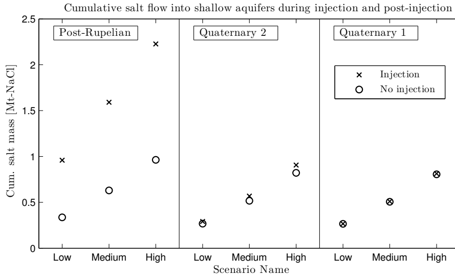
Figure 10. Scenario study 1 – The cumulative salt flow for a period of 100 years (injection + post-injection) into the Tertiary Post-Rupelian, the Quaternary 2, and the Quaternary 1 each for the low, medium, and high scenario. The crosses correspond to simulations with injection, whereas the circles correspond to cases without injection, i.e. only the salt base flow.
