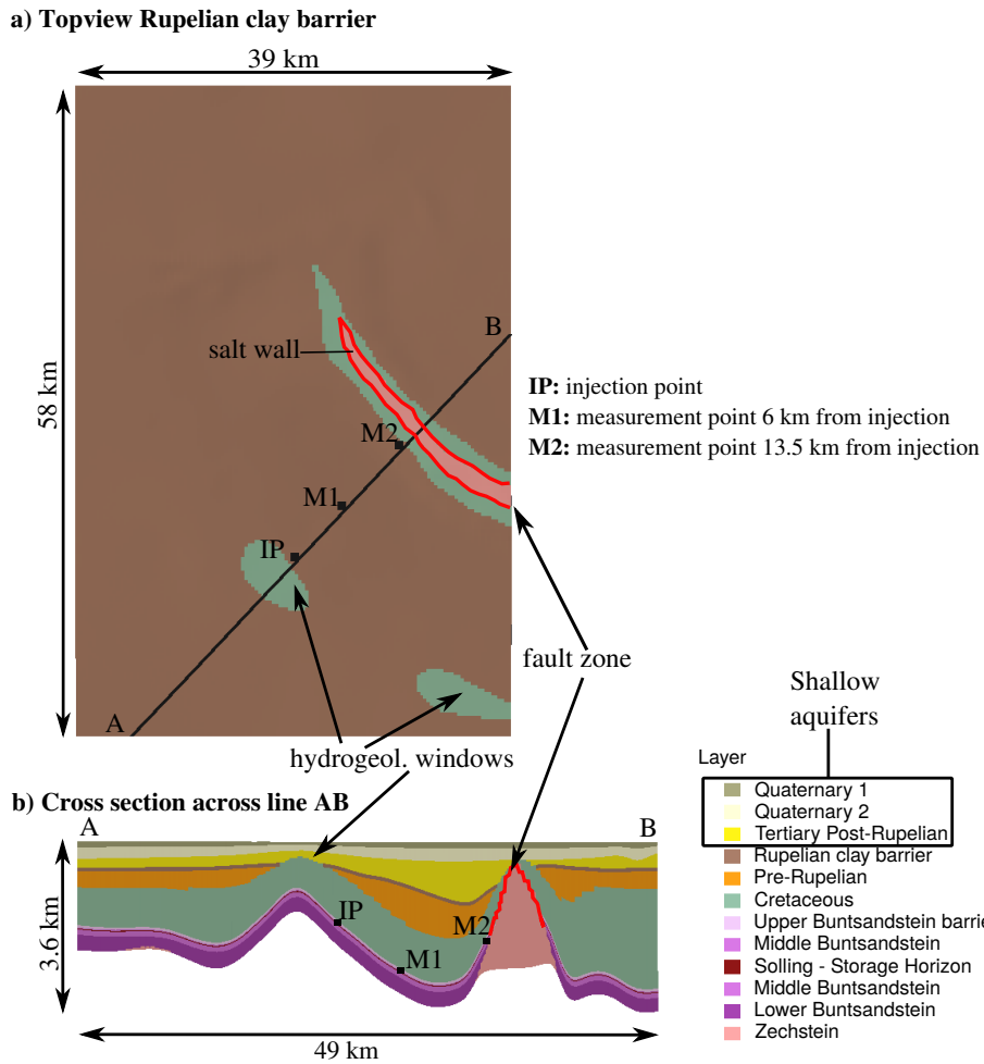
Figure 7. a) Top view on the Rupelian clay barrier. Also shown are the two hydrogeological windows in the Rupelian clay barrier layer and the salt wall piercing through the barrier layer. The fault zone is highlighted in red. b) shows a cross section (vertical exaggeration 4:1) across line A-B with approximate locations of the injection point (IP) and the two measurement points for pressure (M1 and M2).
