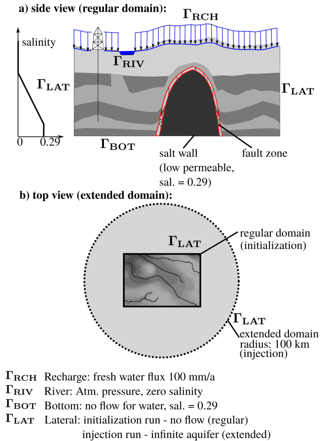
Figure 5. Simplified sketch of the model domain. a) Boundary and initial conditions of the domain shown through a simplified sketch of the geological model. A linear salinity profile increasing with depth up to a maximum salinity (salt mass fraction) of 0.29 \text{ kg kg}^{-1} is assumed as an initial condition for the initialization run. Also shown is the position of the fault zone situated at the flank of the salt wall in red. b) Top view of the domain showing regular domain boundary used during initialization runs and extended domain boundary used for injection runs.
