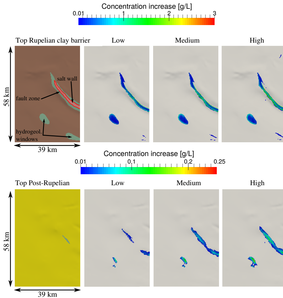
Figure 9. Scenario study 1 – Top row: View on top of the Rupelian clay barrier. The top left figure shows the top view on the geology (as shown in Fig. 7 a). The three figures on the right show the salt concentration increase after 50 years of injection, for the three different scenarios Low, Medium and High with increasing initial salt gradients. Concentration increases below 0.01 g/L are not shown. Bottom row: View on top of the Post-Rupelian. The bottom left figure shows the top view on the geology of the Post-Rupelian. The three figures on the right show the salt concentration increase after 50 years of injection, again for the same three scenarios. Note the different scales on the legends for the top and bottom row.
