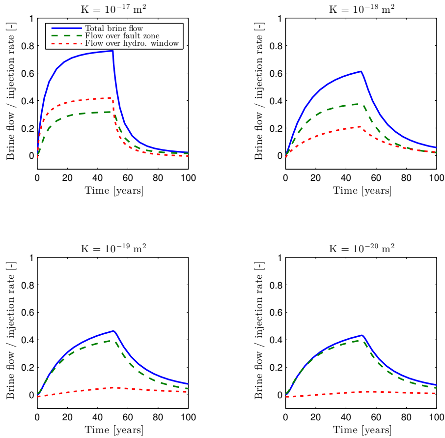
Figure 12. Scenario study 3 – Variable Upper Buntsandstein barrier permeability. Brine flow normalized by the brine injection rate into the shallow aquifers, for different permeabilities of the Upper Buntsandstein barrier. The upper right scenario with a permeability of 1 \cdot 10^{-18} \text{ m}^2 corresponds to the reference case.
