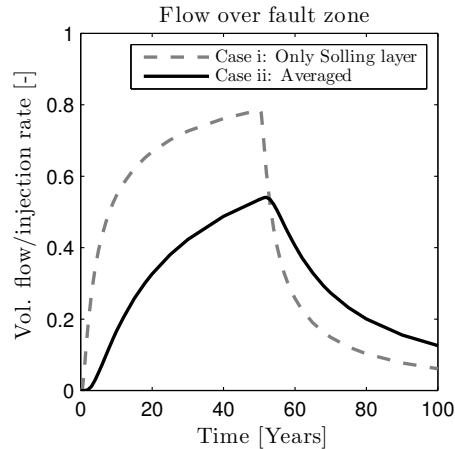
Figure 15. Focused leakage scenario – Results of the Analytical Model for the two cases: (i) the injection horizon comprises only the Solling sandstone layer and (ii) the injection horizon comprises all layers in the Middle and Lower Buntsandstein with an averaged injection horizon permeability and porosity.
