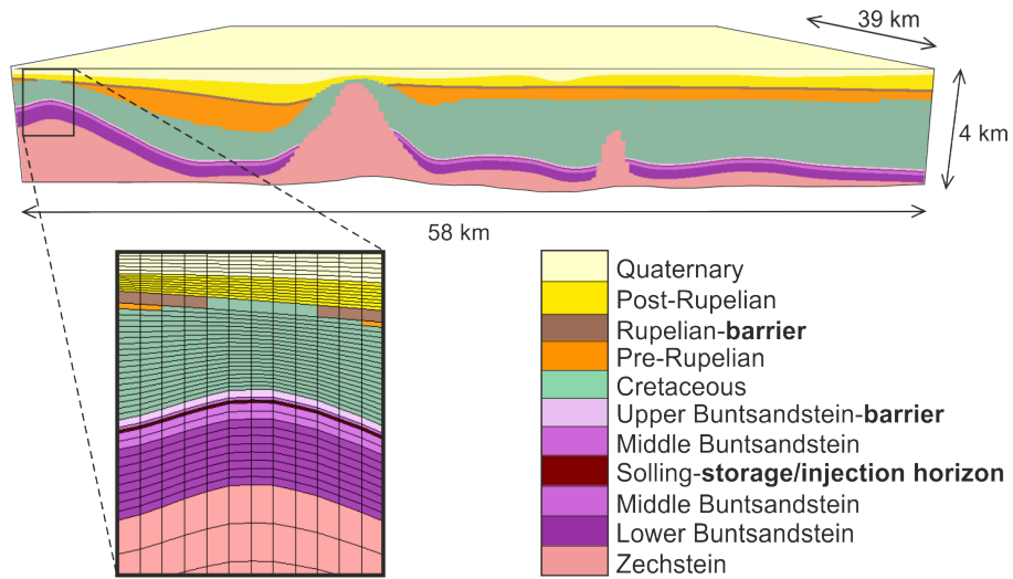
Figure 2. Perspective view on the 3D geological model with zoom in on the anticlinal structure showing the mesh of the 3D volume model. Vertical exaggeration 2:1.
