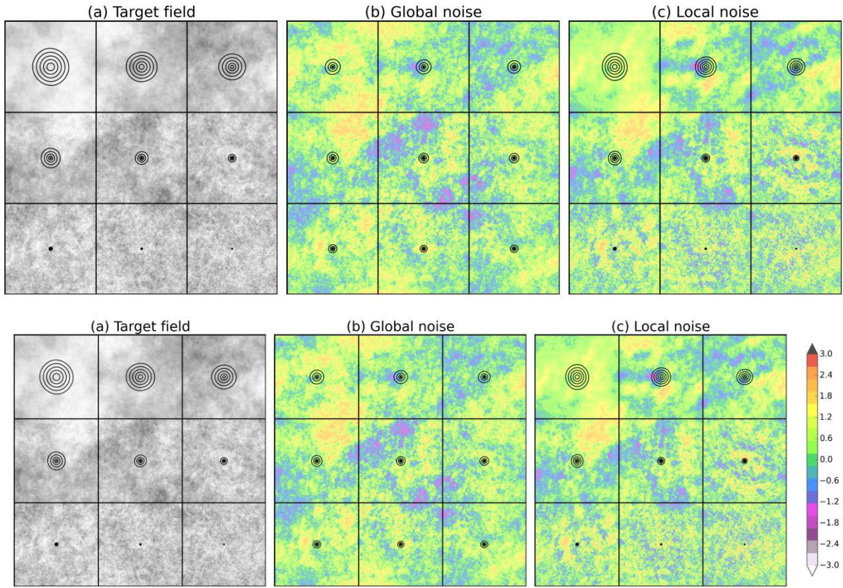
Figure 4. (a) An example of 512x512 pixel non-stationary correlated Gaussian noise generated using parametric filtering. The spectral slope \beta increases from -3.0 to -1.5 from the top towards the bottom of the image as represented by black
