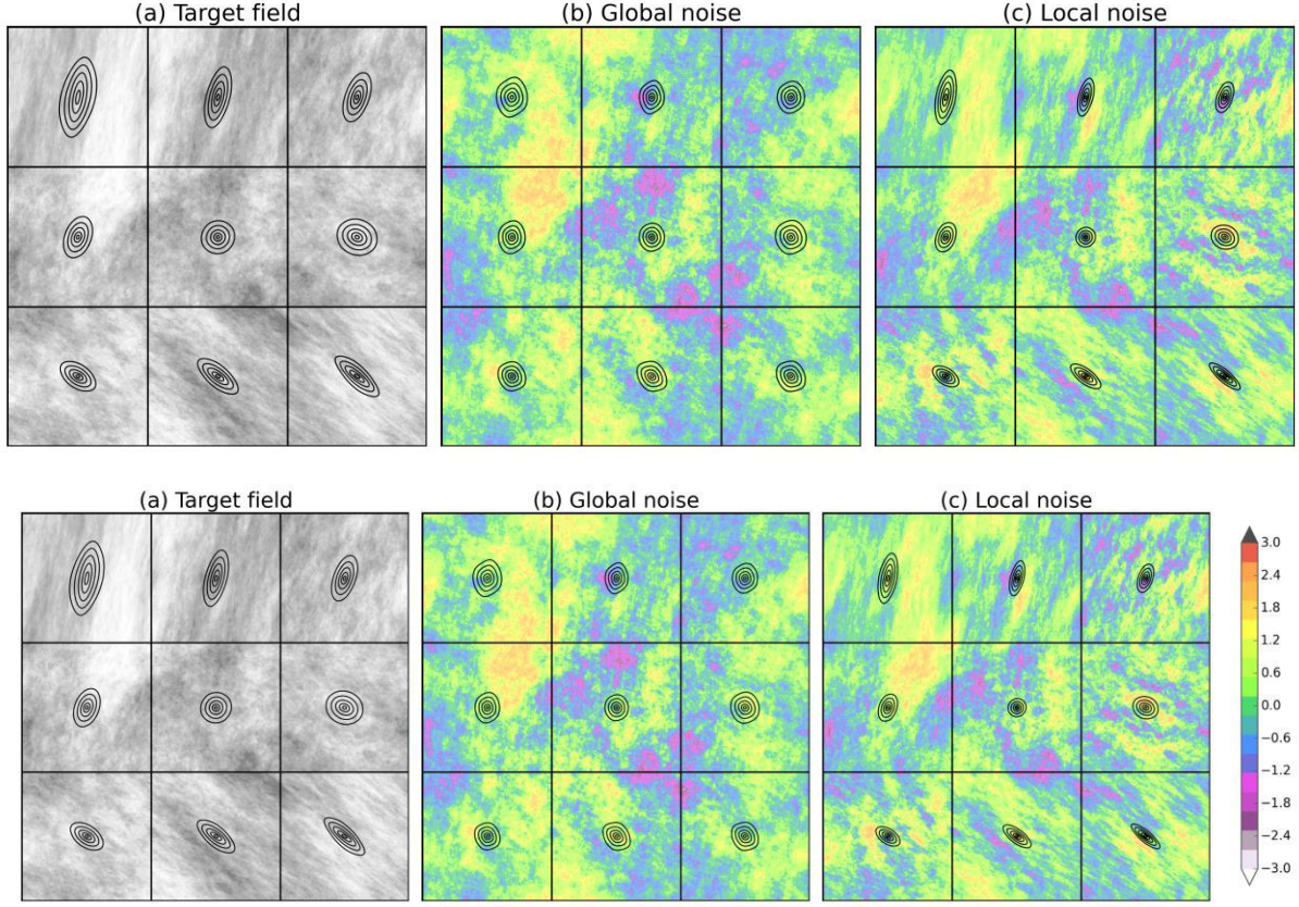
Figure 5. (a) An example of 512x512 pixel non-stationary correlated Gaussian noise generated using parametric filtering. The GSI parameters (see Niemi et al. , 2014 for details) linearly evolve from G(-0.12, -0.12, -0.12) and I_s = 5 at the upper left corner to G(0.12, 0.12, 0.12) and I_s = 5 at the lower right corner of the image. The black contours show the corresponding autocorrelation functions at 0.5, 0.6, 0.7, 0.8 and 0.9 correlation coefficients. Non-parametric stochastic realisations of the target field using a global generator (b) and a local SSFT generator (c) with Hanning windows centred over the grid boxes in the image. All simulations have been drawn from the standard normal distribution and share the same random seed.
