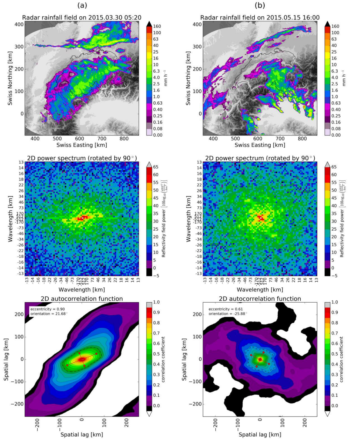
Figure 8. Radar rainfall fields (top row), 2D Fourier spectra zoomed on frequencies wavelengths > 13 km and rotated by 90^\circ (centre row) and corresponding 2D autocorrelation functions (bottom row) for case studies on (a) 30 March 2015 and (b) 15 May 2015. The autocorrelation function is obtained as inverse FFT of the 2D power spectrum. The 90^\circ rotation is performed in order to align the anisotropies of the 2D spectra and spatial autocorrelation functions. The anisotropy is estimated by eigenvalue decomposition of the autocorrelation function using values only inside the dashed region and shifted to start from 0. The eccentricity is obtained as \sqrt{1 - \frac{\text{minor axis}}{\text{major axis}}} and is comprised constrained between 0 (perfect circle) and 1 ( minor axis \ll major axis ; a_{\text{minor}} \ll a_{\text{major}} ).
