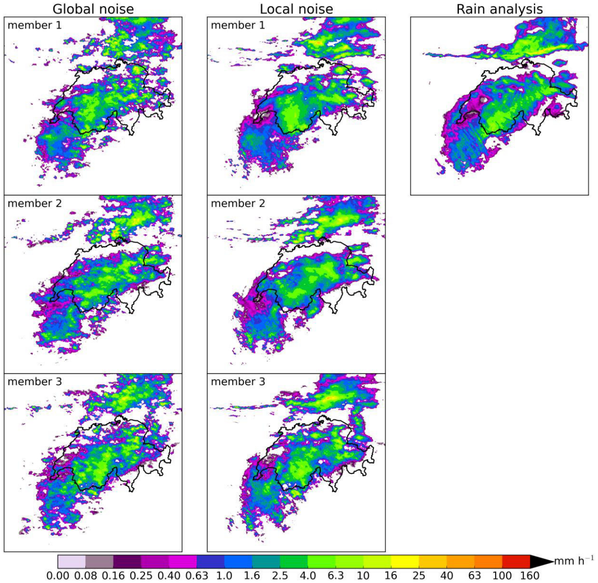
5 | Figure 12. Three stochastic realisations conditioned to case study 1 (30 March 2015) after local adjustment at 64 km resolution of correlated global FFT ( left ) and local SSFT ( centre ) Gaussian noise. The top right panel shows the actual observed field. Parameters of the local SSFT generator: window size = 128 km, overlapping = 50%. The national borders of Switzerland are included as spatial reference (black contour).
