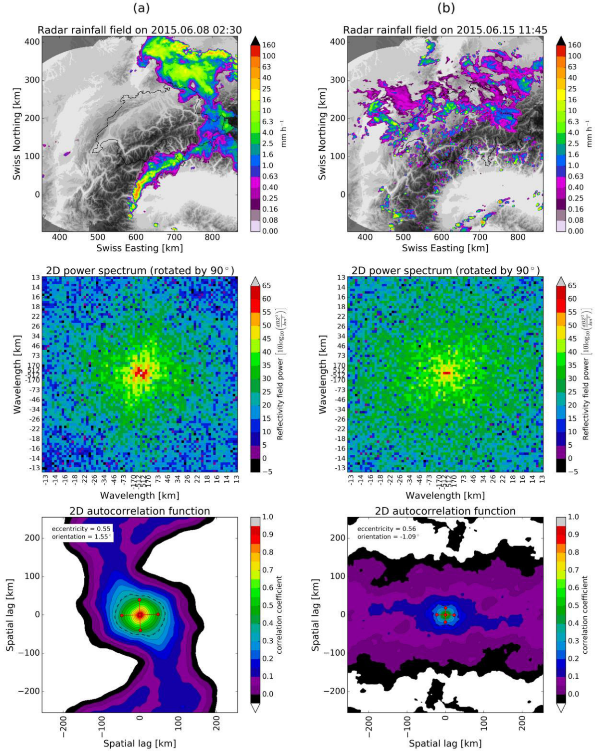
Figure 9. Radar rainfall fields (top row), 2D Fourier spectra zoomed on frequencies wavelengths > 13 km and rotated by 90^\circ (centre row) and corresponding 2D autocorrelation functions (bottom row) for case studies on (a) 8 June 2015 and (b) 15 June 2015. More details are provided in the caption of Fig. 8.
