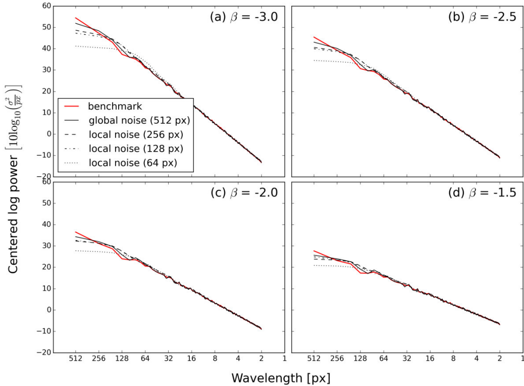
5 Figure 6. The radially averaged 1D centred power spectra of synthetic realisations with spectral slope (a) \beta = -3.0 , (b) \beta = -2.5 , (c) \beta = -2.0 and (d) \beta = -1.5 (in red). In black are the corresponding average spectra of 20 non-parametric realisations for decreasing window sizes. The same experiment was realized with real precipitation fields (see Fig. 11).
