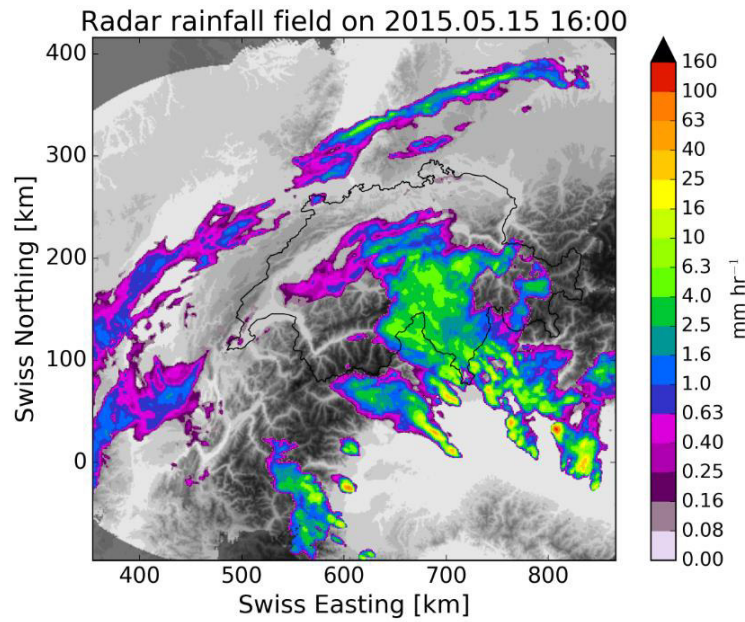
Figure 1. Example of non-stationarities in a radar rainfall field of -512x512 km centred over Switzerland. Two distinct anisotropies coexist in the same image, while convection develops only to the south of the Alps.
