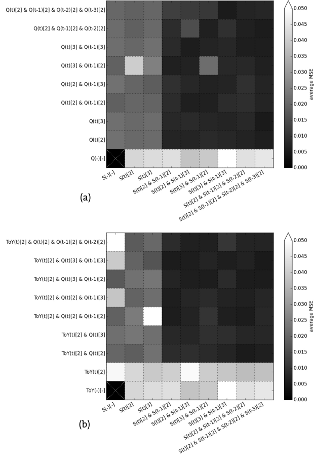
Figure 12. Matrix showing the average test MSEs of the 11 considered reservoirs as the number of input variables and membership functions increases. (a) shows combinations of storage and inflow input variables and (b) also includes the Time-of-Year variable.
