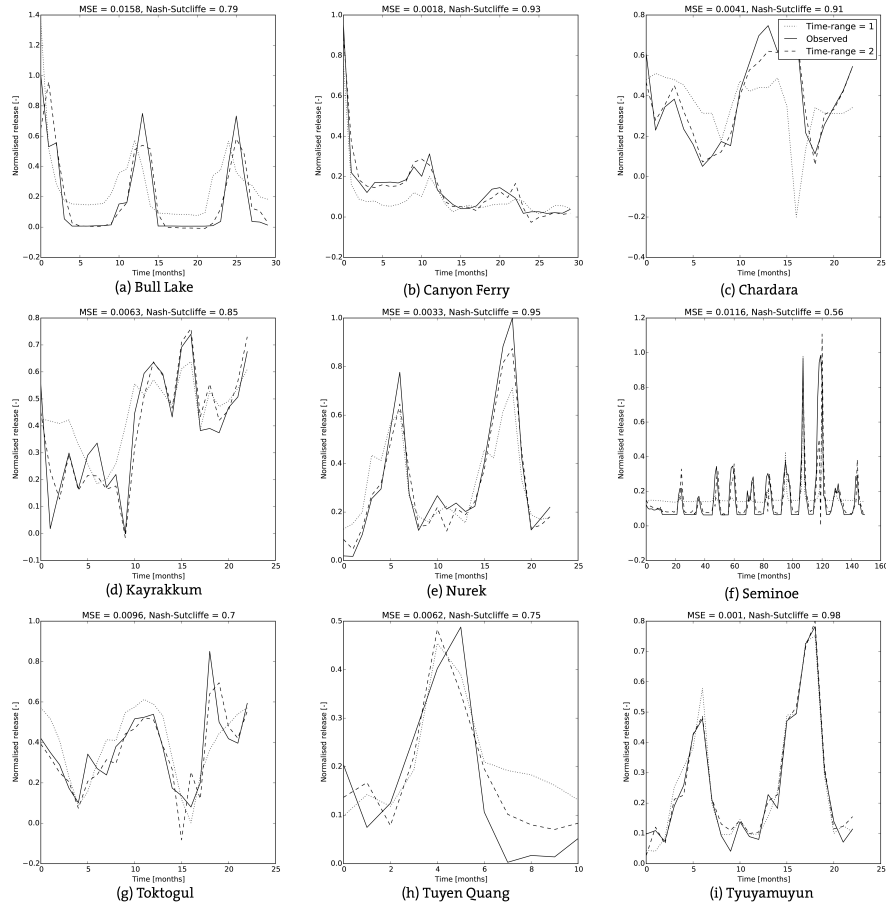
Figure 15. Simulated and observed reservoir releases for nine reservoirs when simulated with a time-range of one or two.
