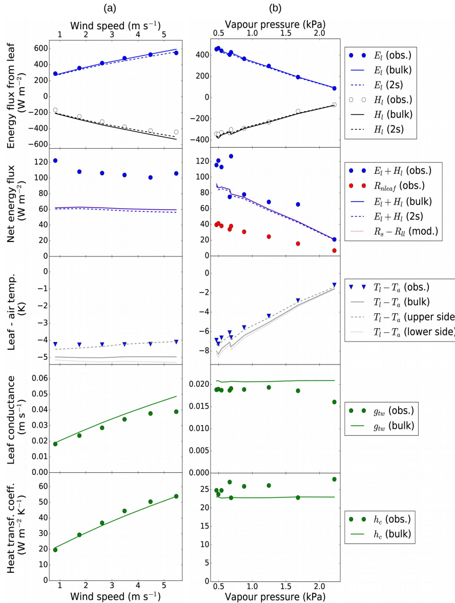
Figure 9. Artificial leaf with wet surface on the lower side (no stomatal resistance), under (a) varying wind speed and (b) varying vapour pressure. Numerical model results (lines) based on the same boundary conditions as observations (symbols). E_l : latent heat flux; H_l : sensible heat flux; R_s - R_{ll} : absorbed net radiation; T_l - T_a : leaf-air temperature difference; g_{tw} : total leaf conductance to water vapour; h_c : convective heat transfer coefficient; “bulk”: bulk leaf temperature model; “2s”: model based on different leaf temperatures on both leaf sides. Boundary conditions: g_{sw} = 999 \text{ m s}^{-1} ; R_s = 0 ; T_a = 295.4 - 295.6 \text{ K} (a) and 295.4 - 296.6 (b); P_{wa} = 1200 - 1342 \text{ Pa} (a); v_w = 1.0 \text{ m s}^{-1} (b); k_l = 0.1 \text{ W K}^{-1} \text{ m}^{-1} ; z_l = 0.5 \text{ mm} .
