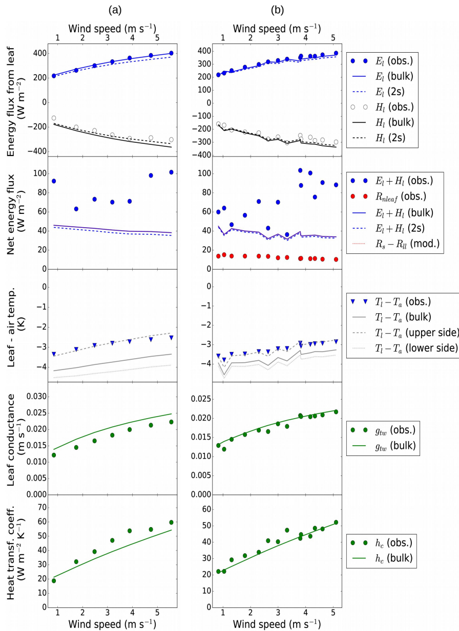
Figure A6. Artificial leaves with (a) 65 and (b) 35 pores mm -2 under varying wind speed. Numerical model results (lines) based on the same boundary conditions as observations (symbols). E_l : latent heat flux; H_l : sensible heat flux; R_s - R_{ll} : absorbed net radiation; T_l - T_a : leaf-air temperature difference; g_{tw} : total leaf conductance to water vapour; h_c : convective heat transfer coefficient; “bulk”: bulk leaf temperature model; “2s”: model based on different leaf temperatures on both leaf sides. Boundary conditions: g_{sw} = 0.05 m s -1 (a) and 0.042 m s -1 (b); R_s = 0 ; T_a = 295.1 - 295.3 K (a) and 295.0–296.5 (b); P_{wa} = 1200 - 1340 Pa (a) and 1190–1280 (b); k_l = 0.03 W K -1 m -1 (a) and 0.1 W K -1 m -1 (b); z_l = 0.35 mm (a) and 0.6 mm (b).
