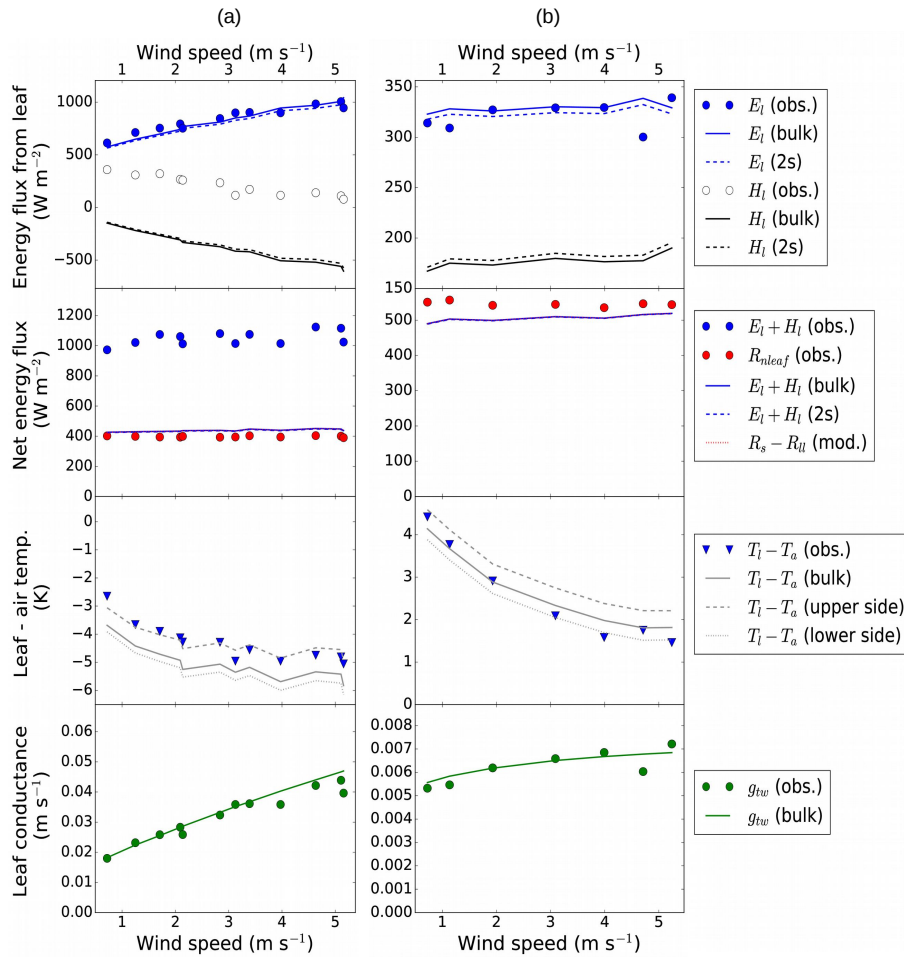
Figure 10. Artificial leaves with (a) wet surface on the lower side and (b) 7 perforations \text{mm}^{-2} . Numerical model results (lines) based on the same boundary conditions as observations (symbols). E_l : latent heat flux; H_l : sensible heat flux; R_s - R_{ll} : absorbed net radiation; T_l - T_a : leaf-air temperature difference; g_{tw} : total leaf conductance to water vapour; h_c : convective heat transfer coefficient; “bulk”: bulk leaf temperature model; “2s”: model based on different leaf temperatures on both leaf sides. Boundary conditions: g_{sw} = 999 (a) and 0.008 (b) \text{m s}^{-1} ; R_s = 370\text{--}380 \text{W m}^{-2} (a) and 530\text{--}550 \text{W m}^{-2} (b); T_a = 295.8\text{--}296.6 K (a) and 295.4\text{--}296.6 K (b); P_{wa} = 521\text{--}802 Pa (a) and 341\text{--}356 Pa (b); k_l = 0.27 \text{W K}^{-1} \text{m}^{-1} (a) and 0.3 (b) \text{W K}^{-1} \text{m}^{-1} ; z_l = 0.5 mm.
