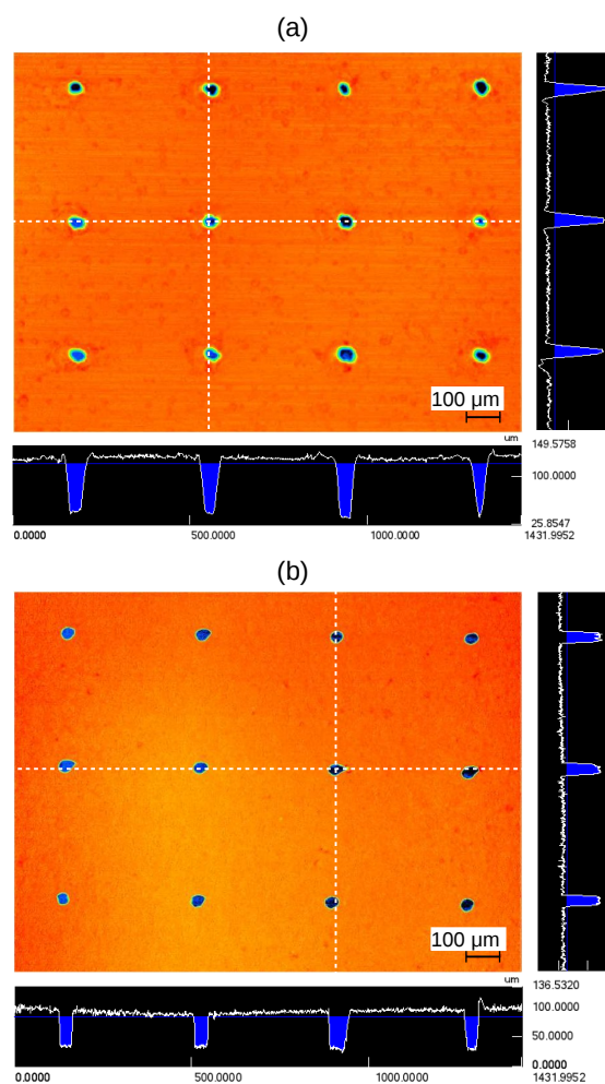
Figure A1. Perforations of the same foil (7 pores \text{mm}^2 ), scanned on the shiny side (a) and on the matte side (b). Colours represent surface elevation as shown in the profile below and to the right of each panel. Ranges of pore sizes and densities are given in Tab. A1.
