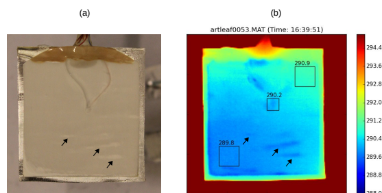
Figure 7. Wet side of thin artificial leaf at 3 \text{ m s}^{-1} wind speed. (a) Photographic image, (b) infrared temperature map, with average temperatures in different sub-areas. Arrows indicate air pockets between wet filter paper and underlying aluminium tape. Wind direction is from bottom to top of the images. Colour bar indicates temperatures in K.
