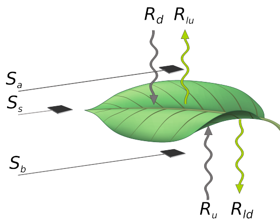
Figure 4. Leaf radiative energy exchange components and net radiation sensors in the radiative field. R_d : downwelling radiation, R_{lu} : longwave radiation emitted upwards by leaf surface, R_u : upwelling radiation, R_{ld} : longwave radiation emitted downwards by leaf, S_a : sensor above leaf, S_s : sensor beside leaf, S_b : sensor below leaf. See Fig. 3 for a picture of the sensors.
