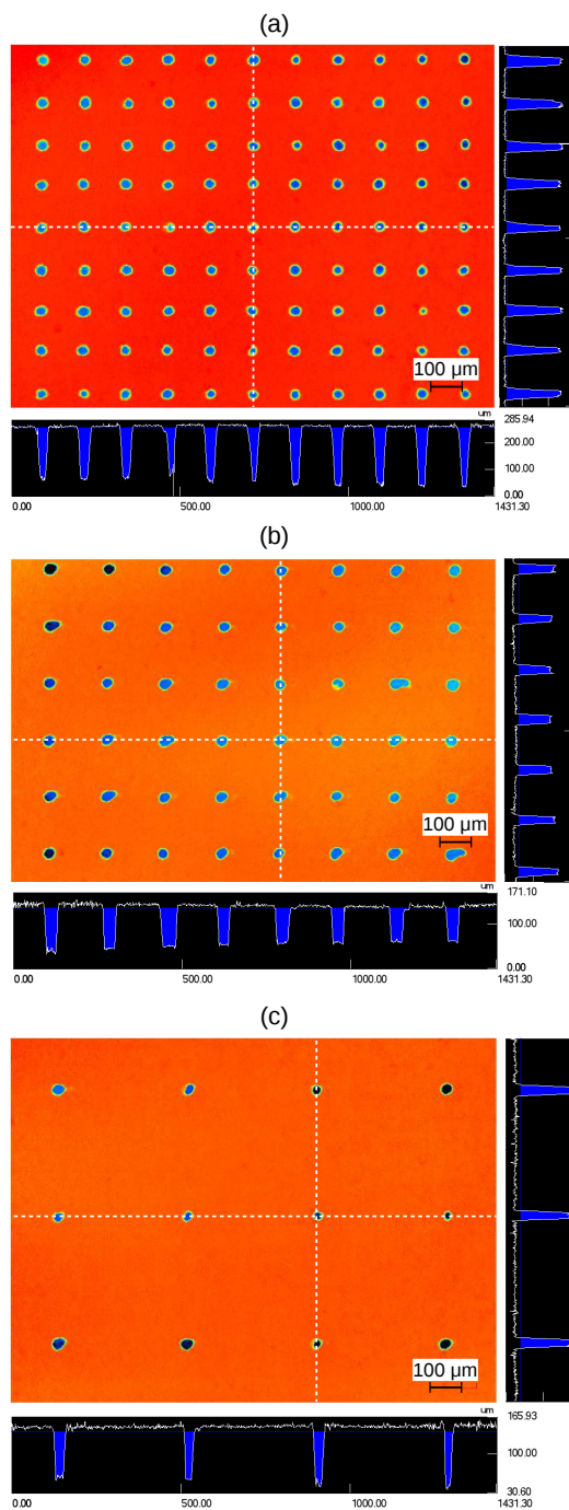
Figure 6. Example confocal laser scanning microscope (CLSM) images of perforated foils summarised in Tab. 1. (a) 64 perforations per \text{mm}^2 , (b) 35 perforations per \text{mm}^2 , (c) 7.8 perforations per \text{mm}^2 . Black bars at the bottom and on the right of each picture show topographic profiles of transects crossing perforations (white dashed lines in main images), with the detection thresholds marked as blue filled areas.
