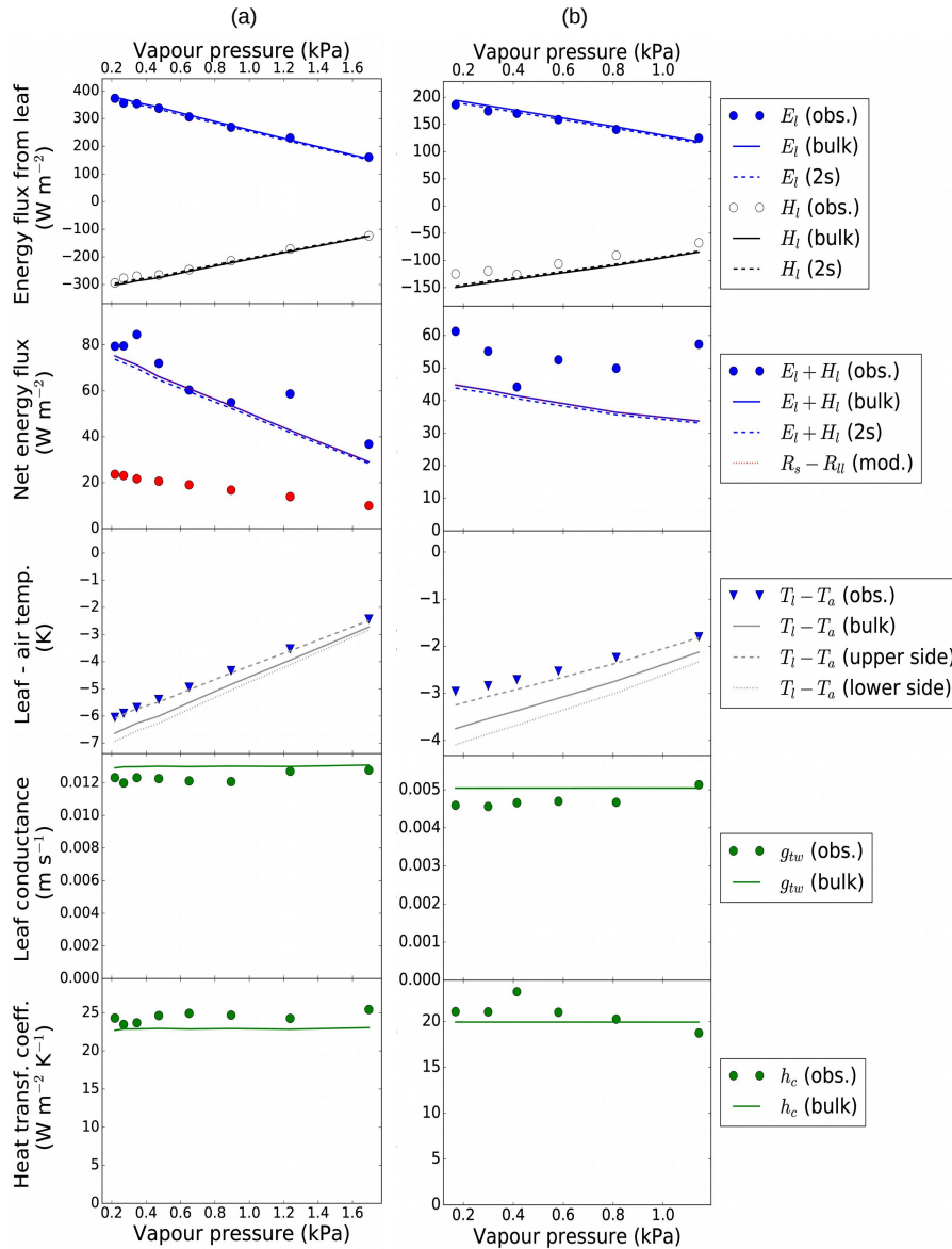
Figure A7. Artificial leaves with (a) 37 and (b) 7 pores \text{mm}^{-2} under varying vapour pressure. Numerical model results (lines) based on the same boundary conditions as observations (symbols). E_l : latent heat flux; H_l : sensible heat flux; R_s - R_{ll} : absorbed net radiation; T_l - T_a : leaf-air temperature difference; g_{tw} : total leaf conductance to water vapour; h_c : convective heat transfer coefficient; “bulk”: bulk leaf temperature model; “2s”: model based on different leaf temperatures on both leaf sides. Boundary conditions: g_{sw} = 0.035 \text{ m s}^{-1} (a) and 0.007 \text{ m s}^{-1} (b); R_s = 0 ; T_a = 295.7\text{--}296.0 \text{ K} (a) and 296.1\text{--}296.7 \text{ K} (b); v_w = 1 \text{ m s}^{-1} (a) and 0.7 \text{ m s}^{-1} (b); k_l = 0.1 \text{ W K}^{-1} \text{ m}^{-1} (a) and 0.05 \text{ W K}^{-1} \text{ m}^{-1} (b); z_l = 0.5 \text{ mm} .
