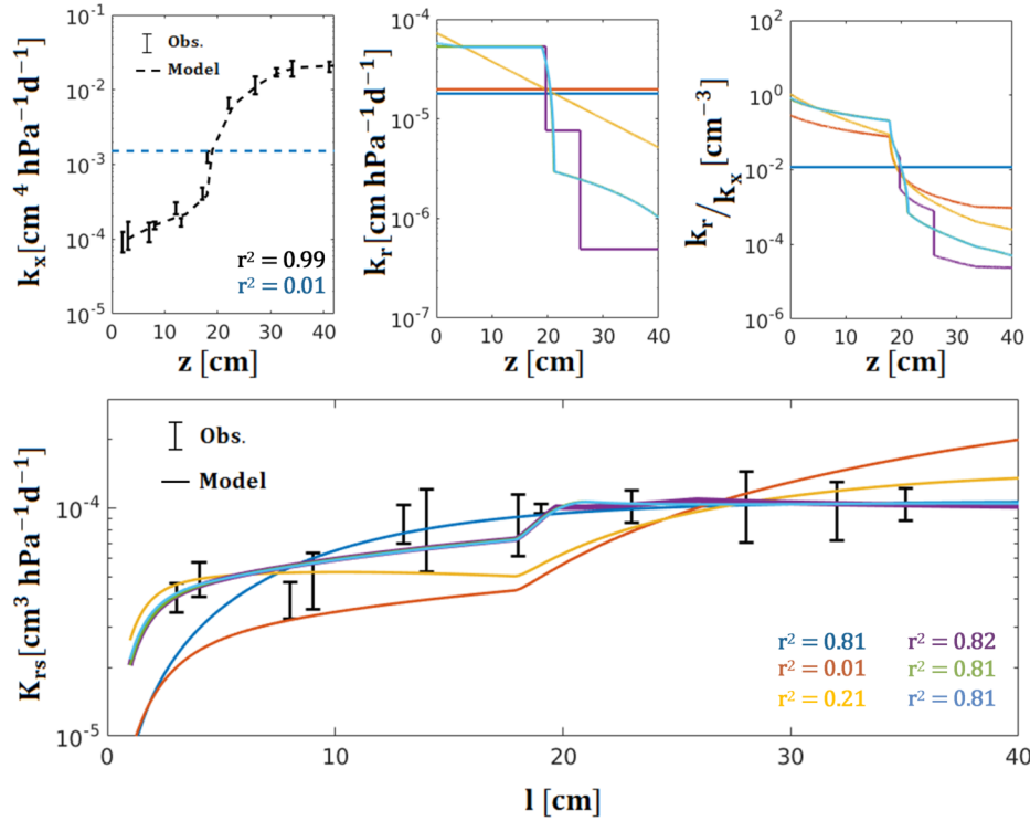
Figure 9. Hydraulic properties of the maize brace roots: axial and total hydraulic conductance of different root types as function of distance from root tip (dark symbols, first and last subplot, respectively). Data presented as dots are average of 5 measurements and the error bars represent the standard divisions. Profiles plotted as solid lines are the best profiles obtained from simulation of water flow into unbranched roots of varying length (last subplot). Second subplot: best fitted profiles of radial conductivity that reproduce measured profiles of total hydraulic conductance. Third subplot: ratio of radial conductivity to axial conductance derived from the analysis along the root axis. The best fitted axial conductance profile was used for each scenario except for the uniform root (dark blue).
