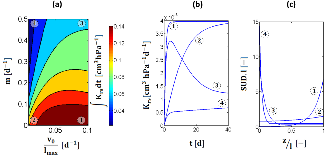
Figure 12. Integral of the root conductance over time when changing the elongation rate \frac{v_0}{l_{max}} (x-axis) and the maturation rate m (y-axis) (a). Root hydraulic conductances of the four extreme cases numbered and indicated in (a) as a function of time (b). Relative uptake of the four single roots after 20 days as a function of the relative position to the root tip ( l is the root length and z = 0 at the tip) (c).
