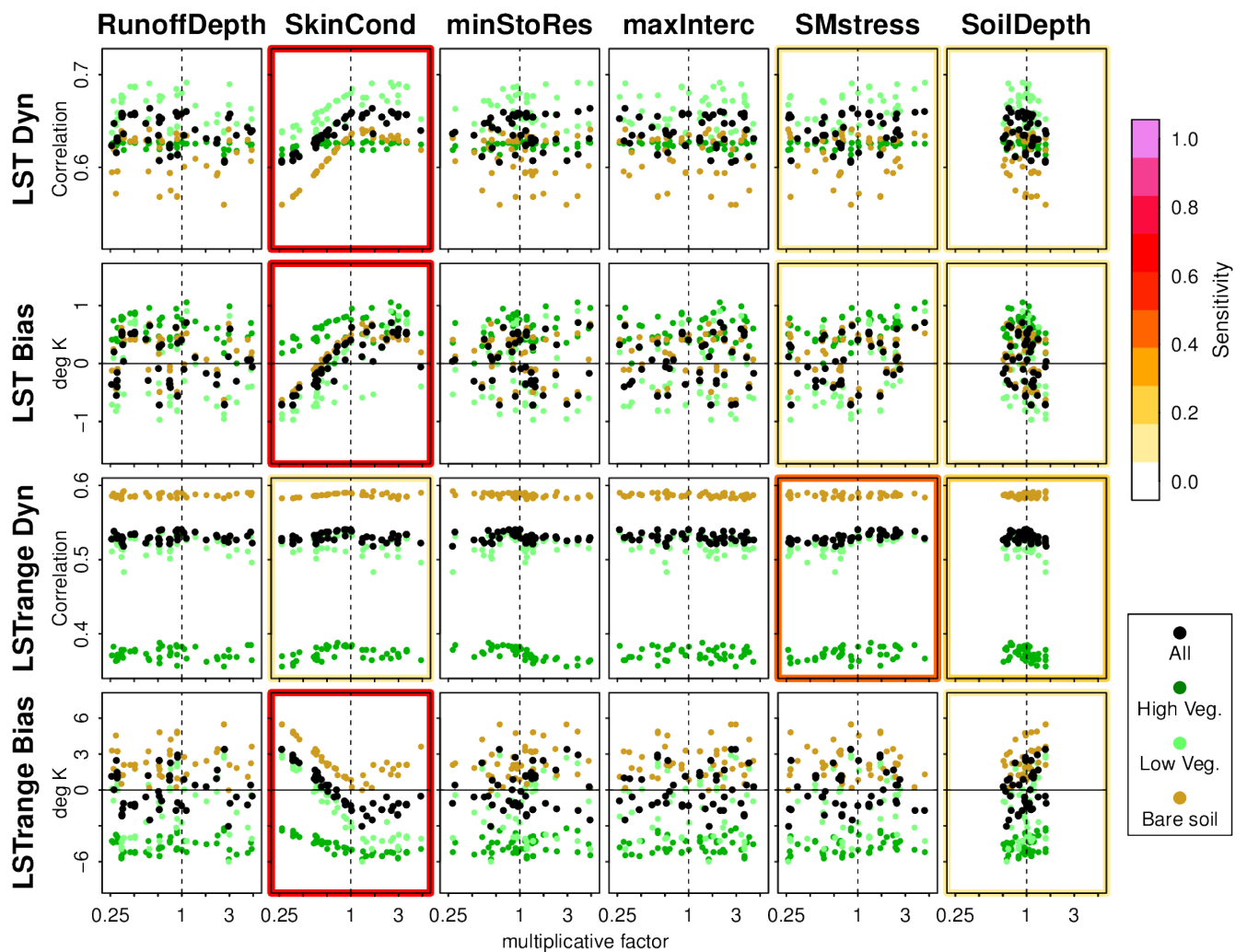
6 Figure S1: As in the lower part of Figure 2, but for the entire domain displayed in
