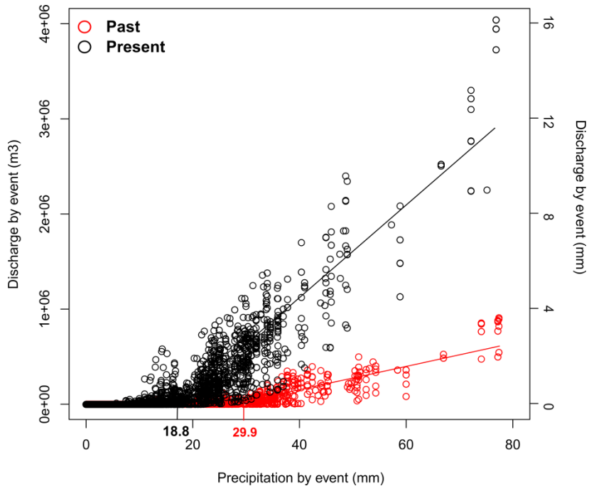
Fig. 7: Relation between precipitation and discharge for all events in the 15 years period in the past (red points) and the present (black points).
