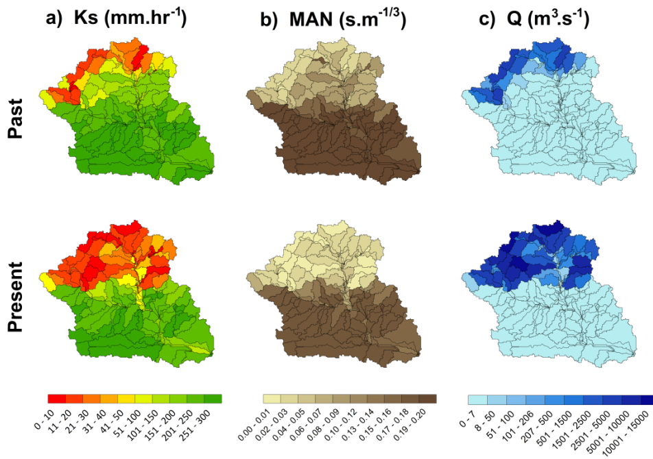
5 Fig. 9: Spatial patterns of the a) saturated hydraulic conductivity (Ks), b) Manning's roughness coefficient (Man) and c) Discharge (Q) between the past and the period for the monsoon season (JAS).
