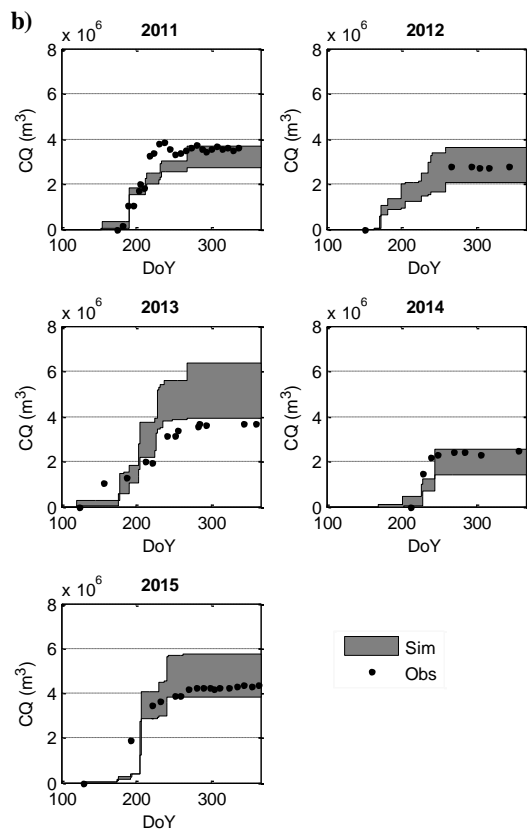
Fig. 5: Cumulative discharge (CQ) for years with observation data over 2000–2015. For each year, black dots are for the observations and the gray-shaded envelop represents the maximum and minimum of the ten members of the ensemble simulations. (a) is for the validation period and (b) is for the channel set-up period.
