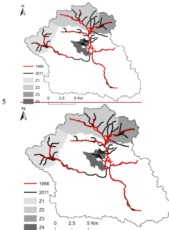
Fig. 4: Identification of the four sub-watersheds (grey shades) which display the largest changes between the drainage network in 1956 (red line) and in 2011 (black line).
