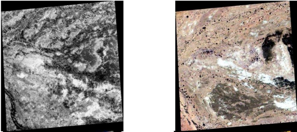
Figure 2: Landscape evolution between 1954 (left) and 2007(right) for the Tin Adjar watershed (Kergoat et al., 2015).
