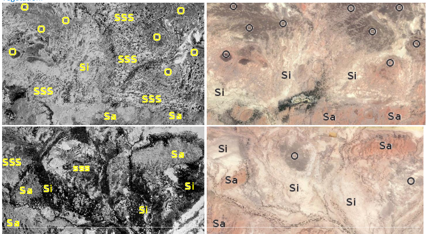
Figure 1: Landscape evolution between 1956 (left) and 2011 (right) for the Agoufou watershed. With SSS: Shallow Sandy Soil; Sa: Sandy soil; Si: Silty soil and O: Outcrop.
