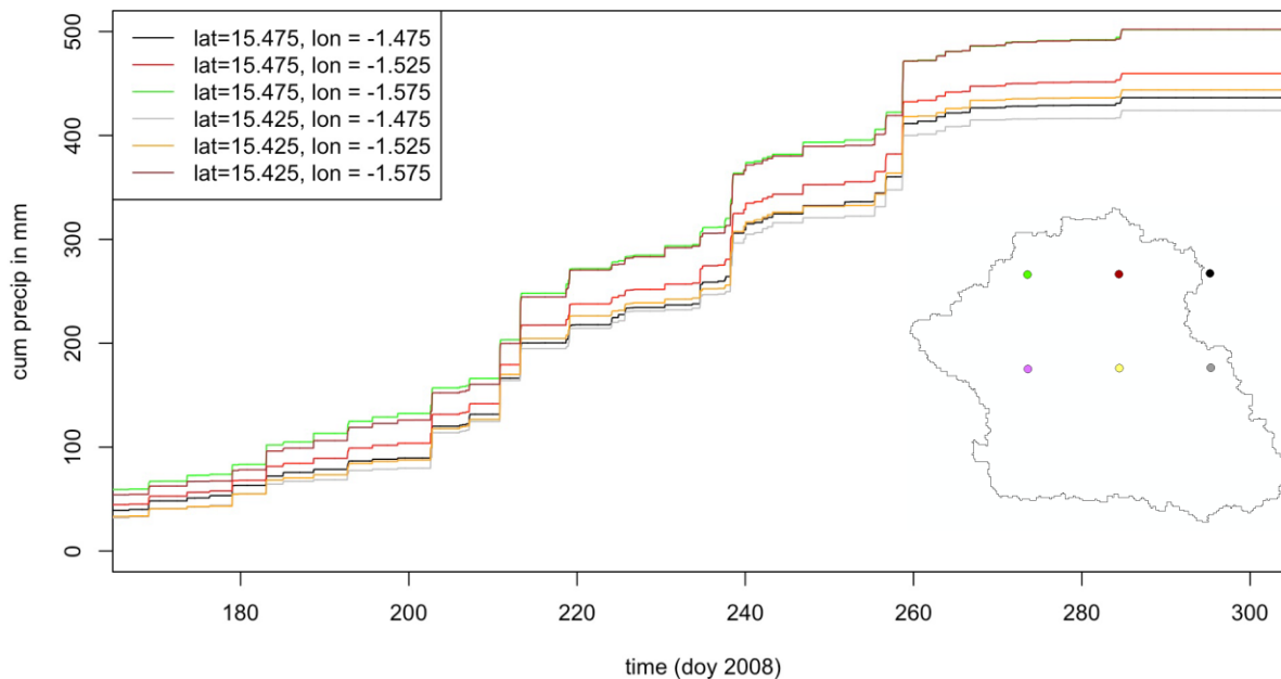
Figure 1: Cumulative rainfall for 2008 in the northern part of the Agoufou watershed (6 pixels located on the map at the right hand side).
