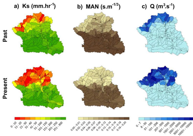
5 | Fig. 9: Spatial patterns of the (a) saturated hydraulic conductivity (Ks), (b) Manning's roughness coefficient (Man) and (c) Discharge (Q) between the past and the period for the monsoon season (JAS).
