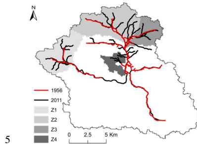
Fig. 4: Identification of the four sub-watersheds (grey shades) which display the largest changes between the drainage network in 1956 (red line) and in 2011 (black line).
