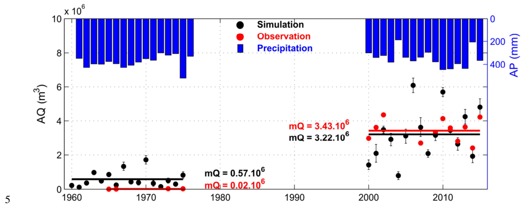
Fig. 6: Evolution of annual discharge (AQ in m^3 ) between 1960 and 2015: simulations with standard deviation of the ten members (black dots with error bar) and observations (red dots) together with annual precipitation (AP in mm, blue bars).
