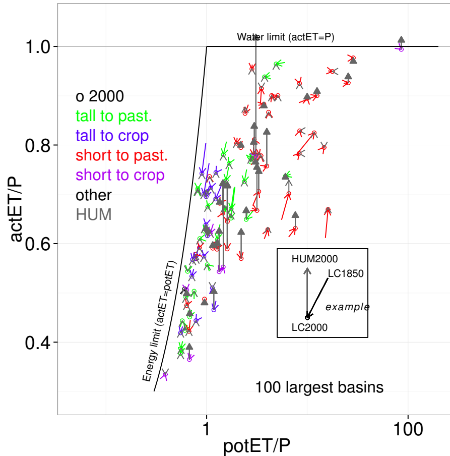
Figure 10. Annual climatological means of actET/P (y-axis) and potET/P (x-axis) for the 100 largest river basins (on our model grid). The x-axis is on a log scale. Circles represent actET/P and potET/P for the LC2000 experiment, colors indicate the land cover change, grey is for human water use. Arrows point from values for the LC1850 to those for the LC2000 experiment (colors), or from LC2000 to HUM2000 (grey), see the example. Solid arrowheads indicate that the change in actET/P induced by human water use is larger than the change induced by land cover. This occurs in 26-33 of the 100 basins. Here we re-classified the land cover changes for the entire basins, we did not group the subbasins that were used in Section 3.3. Figure A7 shows which basins were used for this Budyko analysis.
