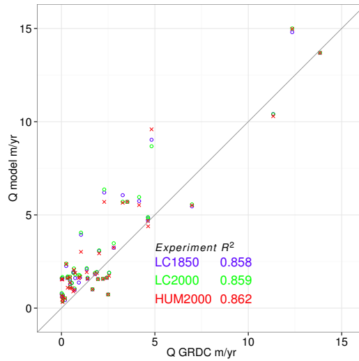
(a) Average discharge Q in m/yr
