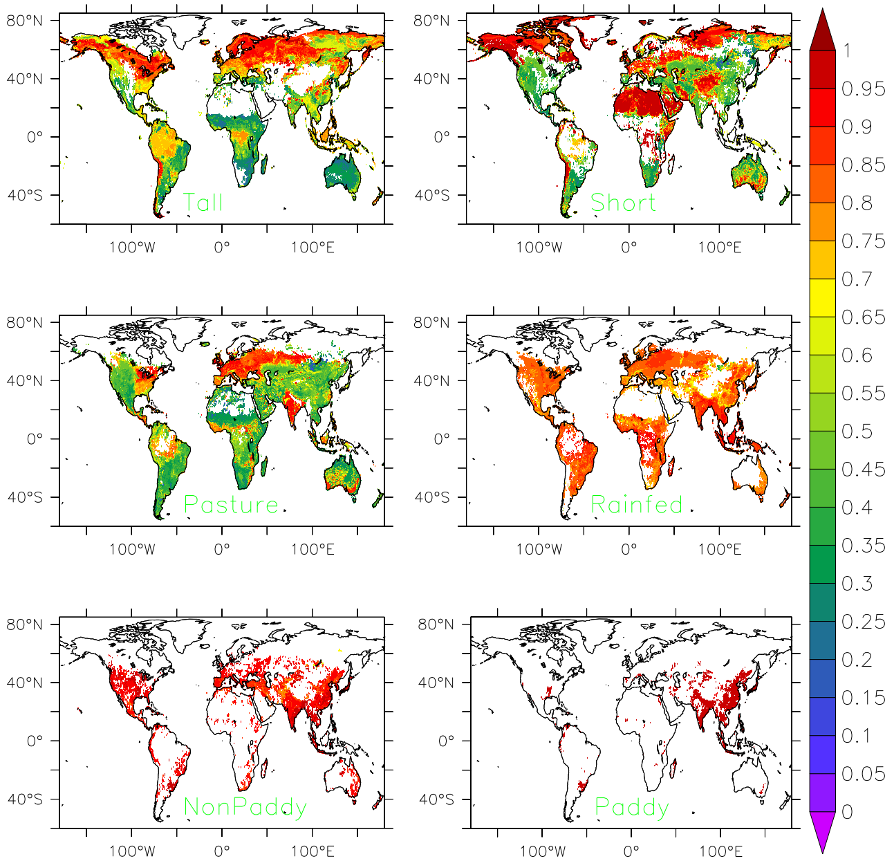
Figure A3. Root fraction in soil layer 1 (upper soil layer, reaching 0.13 to 0.3m depth) in LC2000 per land cover type, used to compute land cover-specific transpiration. A fraction of 1 indicates that all roots are in the upper layer, i.e. no water is taken by the roots from the deeper soil layer. Values are given where a land cover type covers more than 1 % of a grid cell.
