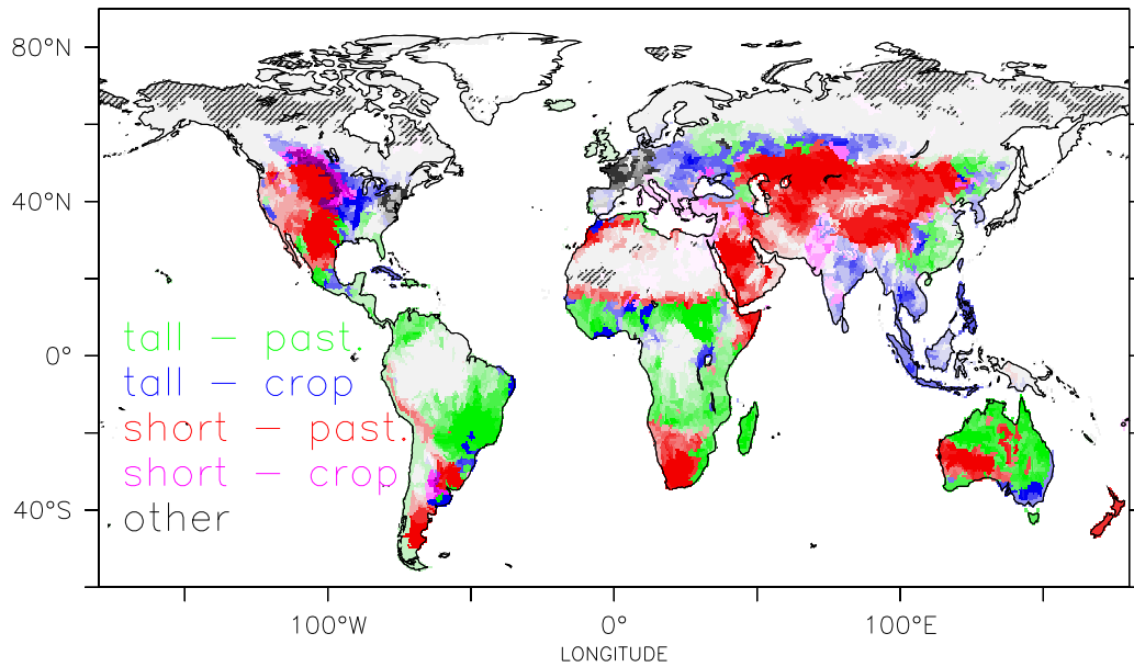
Figure A5. Areas covered by selected subbasins (3995 in total, see Table 2 and Section 3.1). Green areas indicate where the main change in the subbasin is from tall natural to pasture, blue represents tall natural to crops, red represents short natural to pasture and purple represents short natural to crops. Grey indicates subbasins where the main change is from crops or pasture to tall or short natural (e.g. in western Europe, eastern North America). Dashed black indicates where there is no land cover change (e.g. high polar latitudes). Color intensity indicates the change in natural vegetation, with near-white indicating almost no change and most saturated colors indicating that tall or short natural vegetation has de- or increased at least 50%. Table 2 shows the surface areas in each of these areas.
