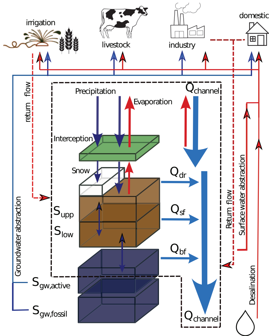
Figure 1. Overview of the PCRaster Global Water Balance model, PCR-GLOBWB. The vertical structure, within the black dashed lines, consists of canopy, two soil layers and a groundwater reservoir. Potential evapotranspiration is broken down into canopy transpiration and bare soil evaporation. Evaporation can occur from the canopy, depending on interception capacity and precipitation intensity, from the soil (depending on soil saturation). Transpiration depends on soil moisture and crop coefficients. Discharge along the channel network consists of direct runoff, interflow or subsurface flow and baseflow. In experiment HUM2000 water abstraction, irrigation and reservoirs are included, as is the use of desalinated water (Wada et al., 2014), hence all fluxes including those outside the black dashed lines are computed. Figure courtesy of S. Pessenteiner.
