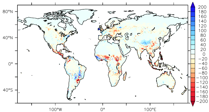
(a) Impact of landcover change (LC2000-LC1850)
