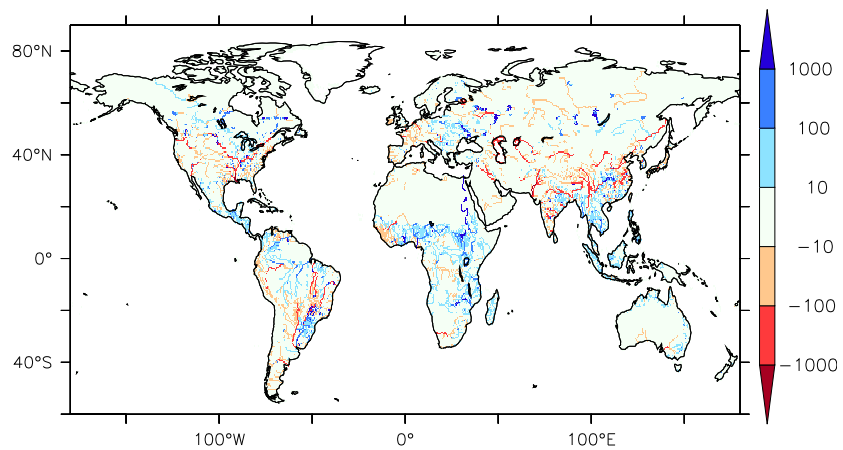
(c) Impact of both (HUM2000-LC1850)
