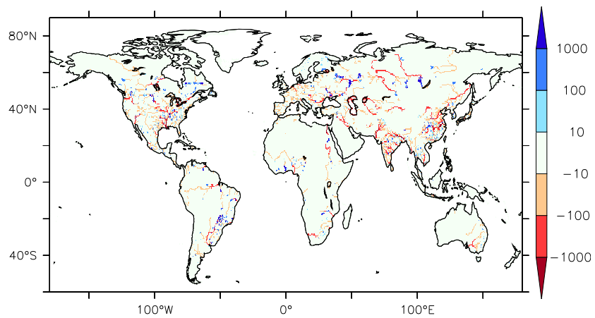
(b) Impact of water use (HUM2000-LC2000)
