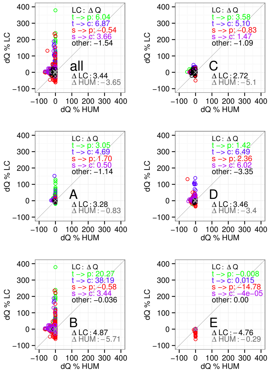
Figure A6. River discharge (Q) changes in % per subbasin for all Köppen classes in the top left as well as per Köppen class. Change due to human water use is represented on the x-axis (HUM, (HUM2000-LC2000)*100/LC2000), change due to land cover change is given on the y-axis (LC, (LC2000-LC1850)*100/LC1850). Each circle color represents a land cover change: tall to pasture (green), tall to crop (blue), short to pasture (red), short to crop (purple), or other (black, crop or pasture to short or tall natural). Grey crosses represent subbasins where no land cover change occurs. Köppen class A is equatorial, B is arid, C is warm temperate, D is snow and E is polar climates. In each figure the top right numbers are the average discharge change per land cover change in %, in the bottom right are the total land cover changes as well as the changes due to human water use in %. Areas and number of subbasins per land cover change are given in Table 2. One subbasin in B, short to pasture, was removed from this figure; with very low Q ( < 1 \text{ m}^3/\text{s} ), dQ in this basin became > 1000\% . Figure 8 shows the absolute changes.
