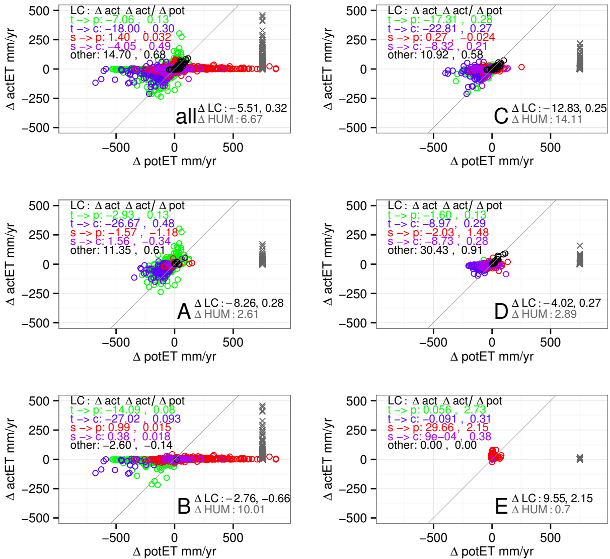
Figure 9. Changes in actual evapotranspiration (actET, y-axis) and potential evapotranspiration (potET, x-axis) from land per subbasin. Circles represent land cover change (LC2000 - LC1850), grey crosses represent human water use (HUM200 - LC2000). Note that there is no change in potET between HUM2000 and LC2000; the grey crosses have been moved along the x-axis for visibility. Each circle color represents a land cover change: tall to pasture (green), tall to crop (blue), short to pasture (red), short to crop (purple), or other (black, crop or pasture to short or tall natural). The top left panel represents all subbasins, the other figures represent a Köppen class. A is equatorial, B is arid, C is warm temperate, D is snow and E is polar climates. In each panel the top left numbers are the average actET change per land cover change and the change in actET divided by the change in potET, in the bottom right are the total land cover changes ( \Delta \text{LC} , LC2000 - LC1850) as well as the changes due to redistribution ( \Delta \text{HUM} , HUM2000 - LC2000). No circles are drawn for subbasins where no land cover change occurs. In all figures the 1:1 line is drawn in grey. Note that in some cases the change in actET is larger than the change in potET, or of opposite sign. This generally occurs where changes in potET are small, such as high latitudes or the Amazon or Congo basins. It may also reflect areas where changes in e.g. soil moisture content or rooting depth alters the response to changed potET. Areas and number of subbasins per land cover change are given in Table 2.
