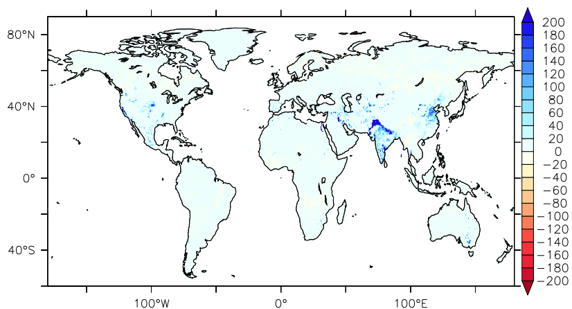
(b) Impact of human water use (HUM2000-LC2000)
