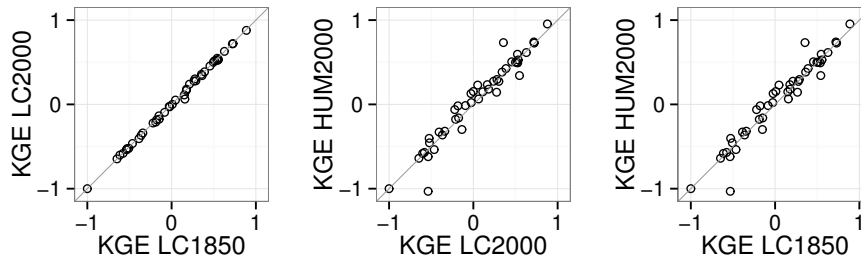
(c) Kling-Gupta efficiency
