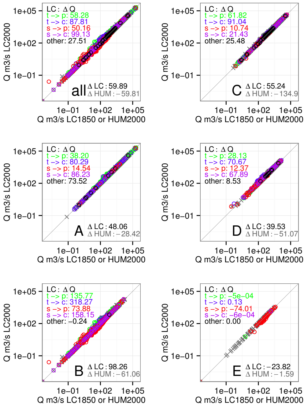
Figure 8. River discharge (Q) changes in m 3 /s per subbasin for all Köppen classes in the top left as well as per Köppen class. The axes are on a log-scale. Each circle color represents a land cover change: tall to pasture (green), tall to crop (blue), short to pasture (red), short to crop (purple), or other (black, crop or pasture to short or tall natural). No circles are drawn in subbasins where no land cover change occurs. Grey crosses represent discharge in LC2000 and HUM2000. Köppen class A is equatorial, B is arid, C is warm temperate, D is snow and E is polar climates. In each figure the top left numbers are the average discharge change per land cover change m 3 /s, in the bottom right are the total land cover changes as well as the changes due to human water use. Areas and number of subbasins per land cover change are given in Table 2.
