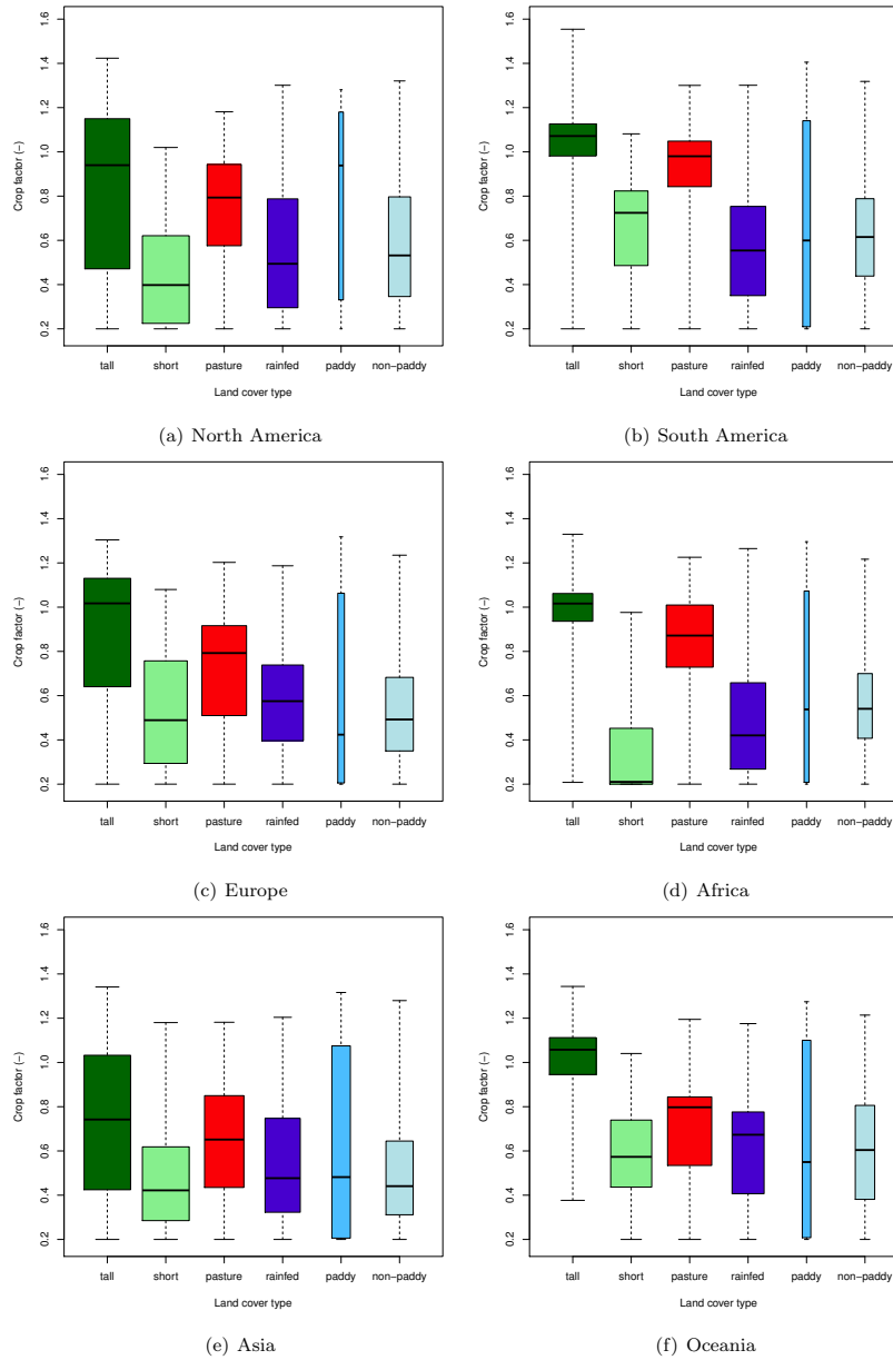
Figure A1. Variation in crop factor ( k_c ) in LC2000, used to compute land cover-specific potential evapotranspiration ( ET_{pot} = k_c * ET_{refpot} ), per continent and per land cover type. All daily k_c values are included. Box plots indicate the minimum and maximum values by the whiskers, the interquartile range (between the first and third quartile) by the box and the median value by the black line within the box. Width of the boxes is proportional to the amount of grid cells within a continent where a land cover type is present. The spread for paddy irrigated crops is high because k_c is high during the growing season but rather low (near 0.2) outside the growing season. Continental masks were derived using basins (see Fig. A2), with North and South America separated through central Mexico, Europe and Africa separated through the Arabian Peninsula, Europe and Asia separated through the Ural mountains, and Asia and Oceania separated roughly along the border of Malaysia and Indonesia.
