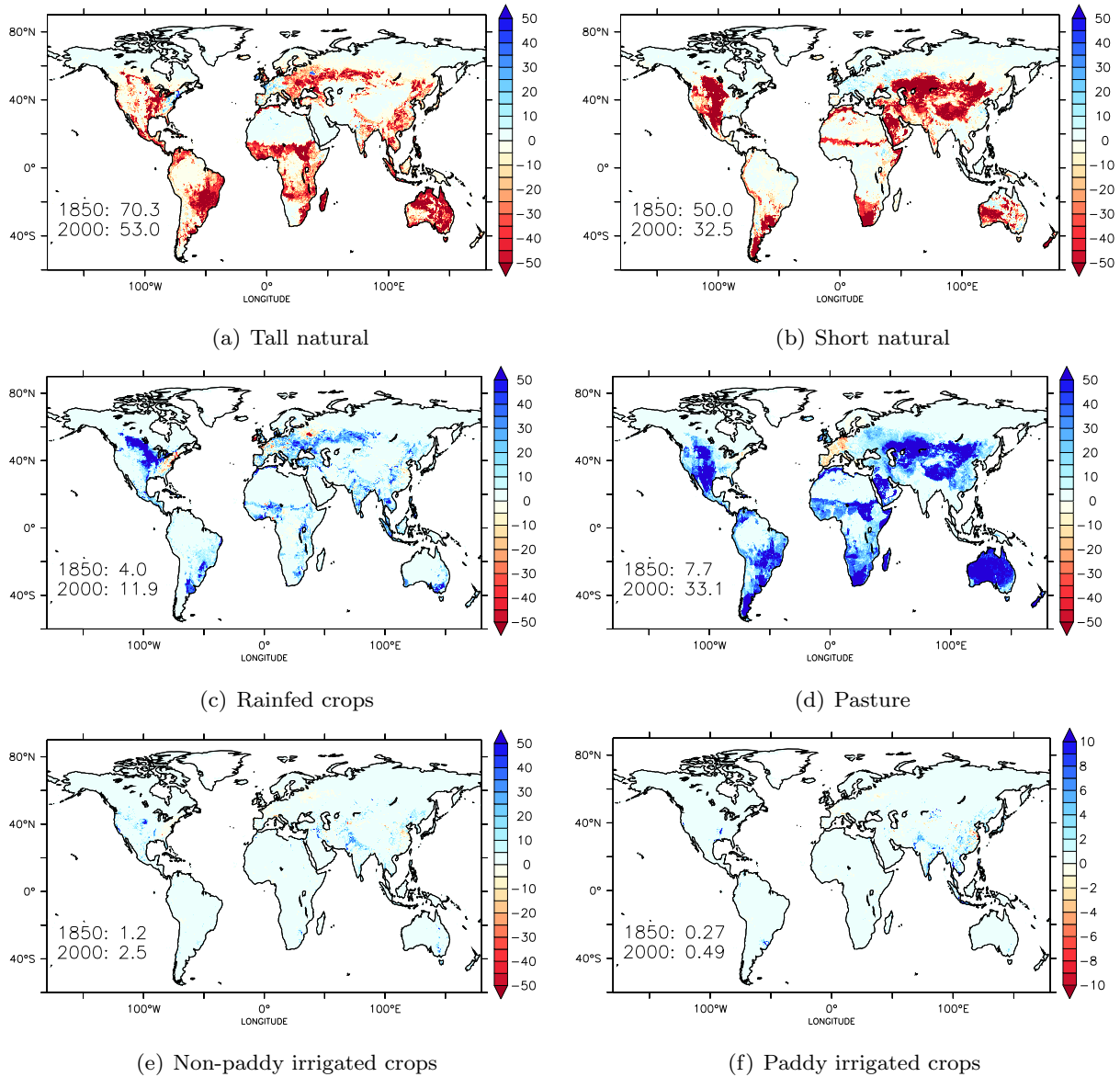
Figure 4. Changes in land cover in each of the 6 land cover classes, expressed in percentage of grid cells. Note that in figures a-e the scale reaches 50%, while in figure f, for paddy irrigated crops, it reaches 10%. The numbers indicate the surface area covered by a land cover type in 1850 and 2000 in 10^6 km 2 . Total land surface area in our experiments is 133 \times 10^6 km 2 (Antarctica is excluded). In experiments LC1850 and LC2000 all crop fields are rainfed, only in HUM2000 do the paddy and non-paddy irrigated fields receive additional water.
