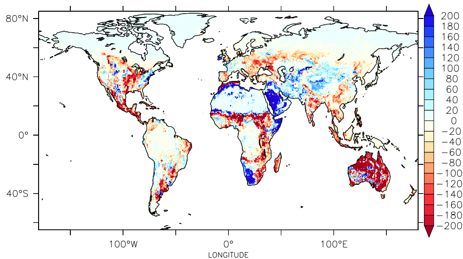
Figure 7. Difference in potential evapotranspiration, averaged over 1979-2010, between LC2000 and LC1850, in mm/yr (average of annual totals). Note that there is no difference in potential evapotranspiration between HUM2000 and LC2000.
