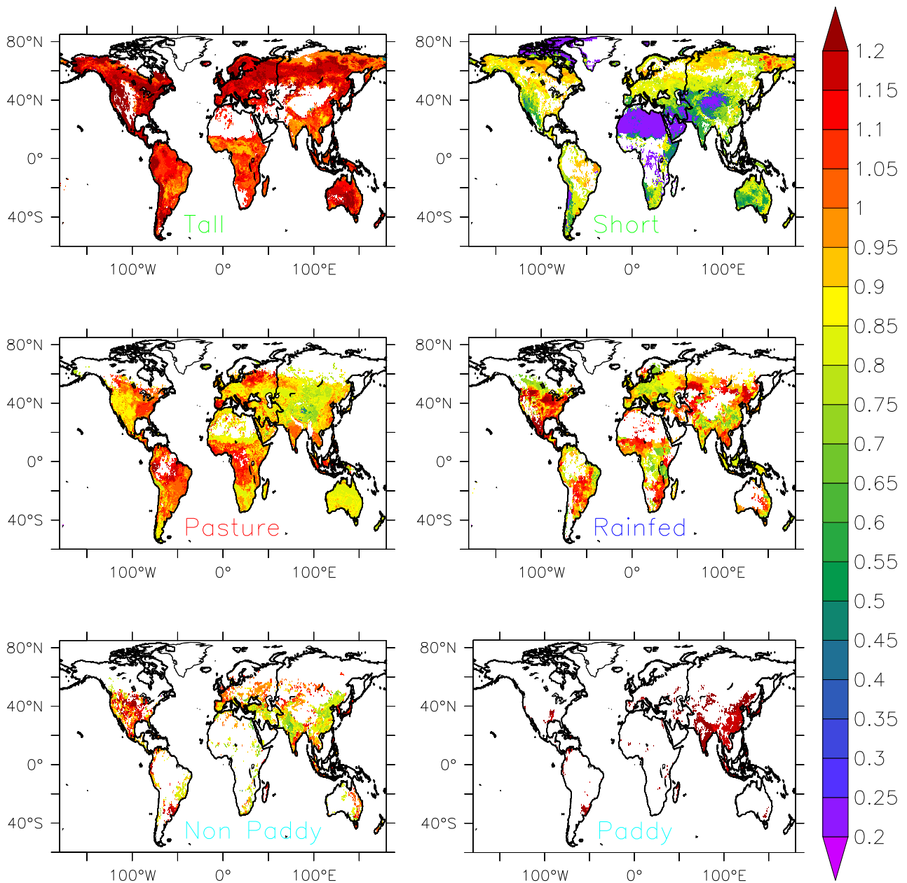
Figure A2. Maximum crop factors ( k_c ) in LC2000 per land cover type, used to compute land cover-specific potential evapotranspiration ( ET_{pot} = k_c * ET_{refpot} ). For each grid cell the maximum value is given, which may occur at different times during the year. Values are given where a land cover type covers more than 1 % of a grid cell. Black lines indicate the masks used for the continents in Figure A1. Note that short natural vegetation includes desert areas where the crop factor is set to a minimum value of 0.2, hence the low crop factors for short natural vegetation in e.g. Africa (see Fig. A1). Low crop factors for short natural vegetation in North Africa derive from Arctic vegetation.
