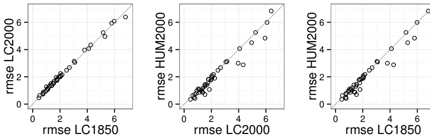
(b) Root mean square error in m/yr
