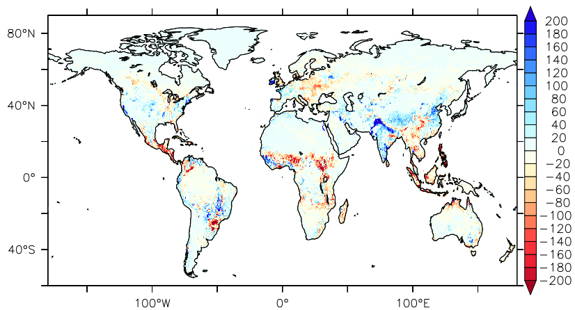
(c) Impact of both (HUM2000-LC1850)
