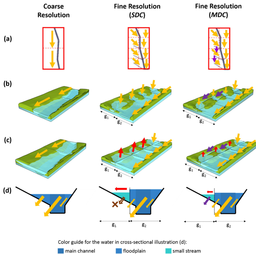
Figure 9. Schematic diagram of the initial distribution of water in coarse and fine resolution simulations. (a) Top view of the river flow network. (b) Isometric 3D representation of the section of the river. Here, to visualize the small rivers and main channels, vertical features of the floodplain are illustrated with exaggeration. Arrows depict flow direction during non-flood conditions. (c) Isometric and (d) cross-sectional illustration of the flow direction in the river network during flooding. Yellow orange arrows indicate the flow of water to the downstream, purple arrows indicate flow in MDC pathways, red arrows indicate backflows, and brown arrows succeeded by "X" marks indicate no flow connectivity in that direction.
