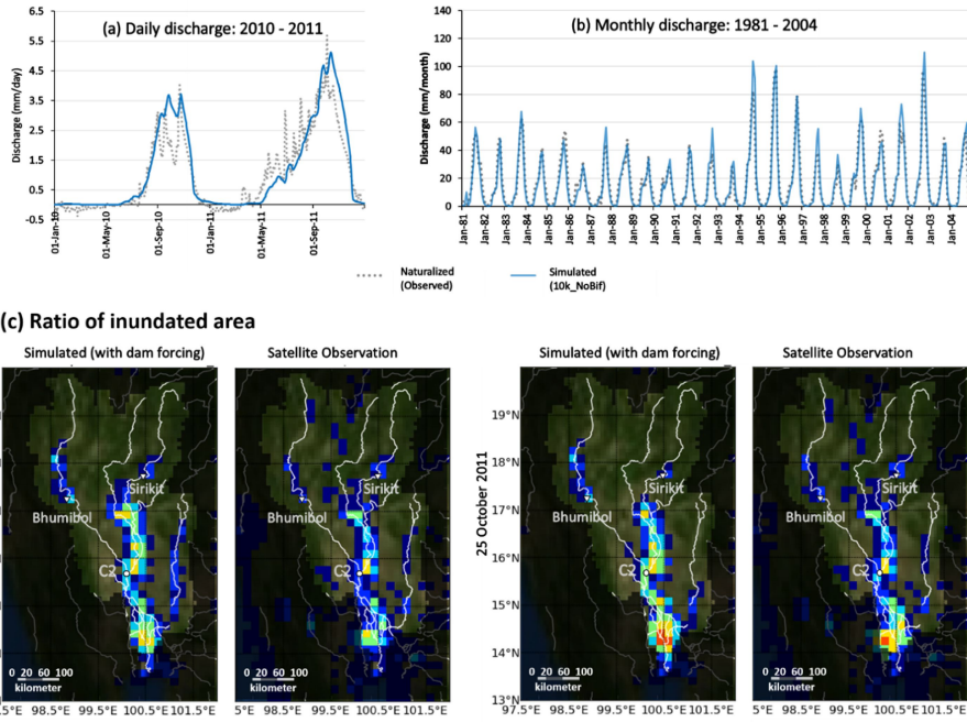
Figure 3. Validation of SDC simulation at 10k resolution. The simulated (a) daily discharge for the years 2010-2011 and the (b) monthly discharge from 1981-2004 were compared with the naturalized observed discharge. The (c) ratio of inundated area in September 25, 2011 and October 25, 2011 were compared with satellite data. Dam forcing indicates the simulations constrained using actual dam outflows as boundary conditions. All figures were modified from Mateo et al. (2014).
