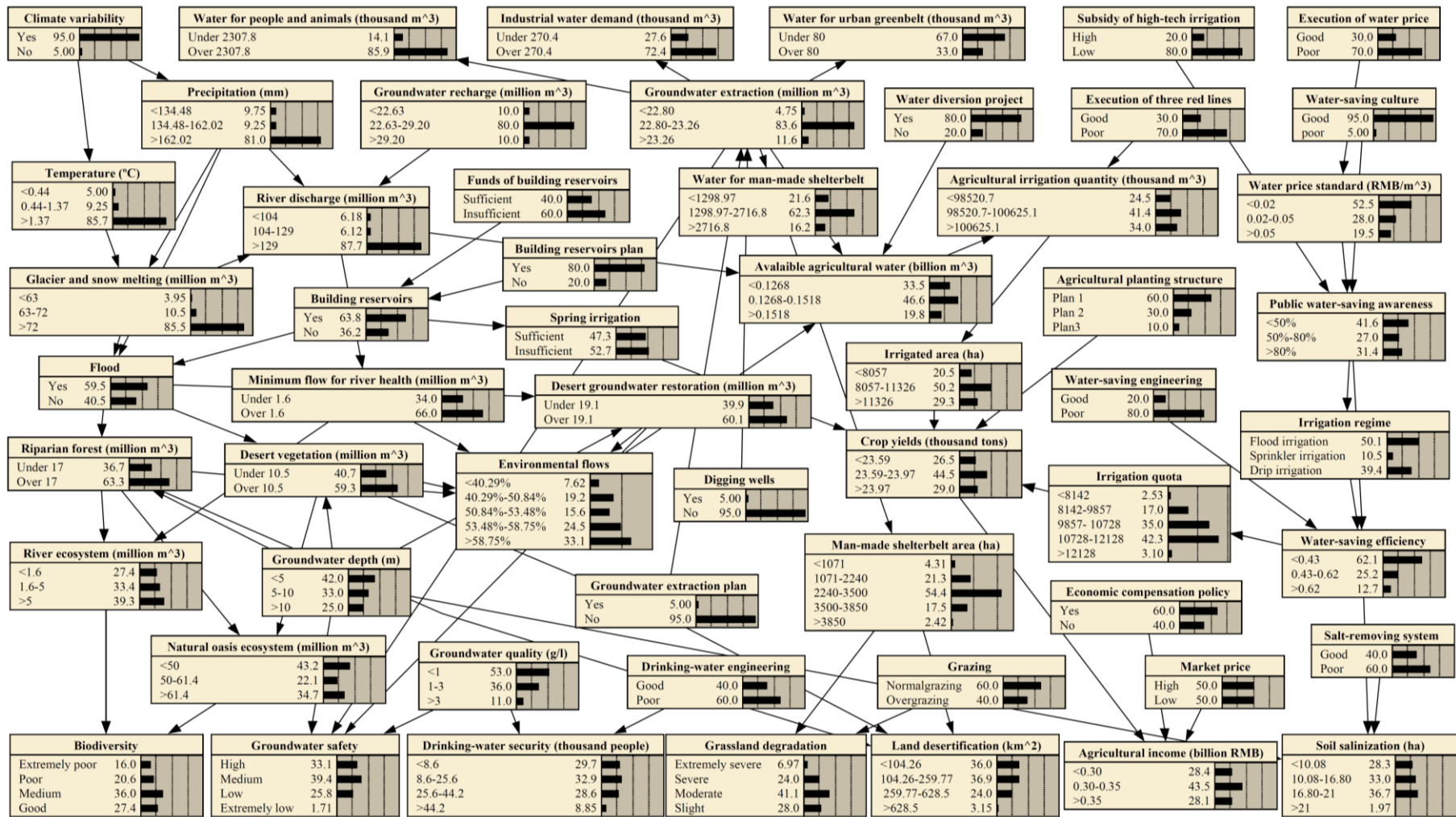
Figure 89. Participatory BN model simulation with elicited CPTs.
