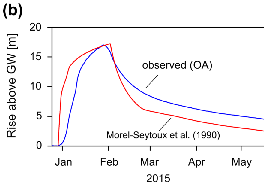
Figure 8. Testing models assumptions. (a) Unit-gradient assumption: the hydraulic gradients (HG) were calculated from the numerical model to test the HG of the lumped model (average HG above the fluctuating groundwater table) and of the seepage model (HG at 6 m depth). (b) 1D flow assumption along the variably-saturated zone: measured groundwater rise above the original groundwater table compared to the analytical solution of Morel-Seytoux et al. (1990) calculated using the infiltration and recharge fluxes of the numerical model.
