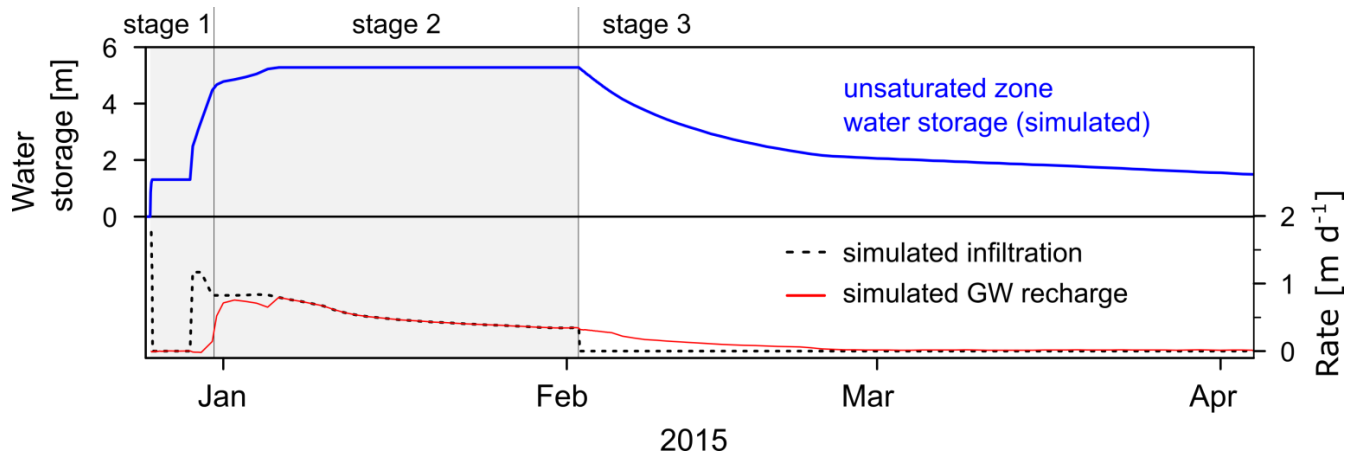
Figure 8 Figure 9. Change in water storage in the unsaturated zone (i.e., above the original water table) during ponding (stage 1 and 2) and drainage (stage 3). Simulated rates of surface infiltration and groundwater recharge are also shown as a reference.
