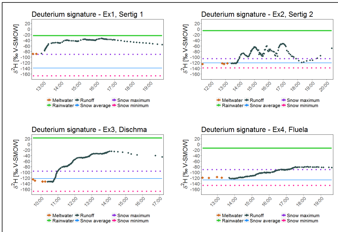
Figure 4 – Deuterium signature of the snowpack runoff during sprinkling (blue dots) or pre sprinkling meltwater (red dots). The lines represent the range (minimum and maximum) and averages of the deuterium signature derived for snow samples and the sprinkling water (Rain).
