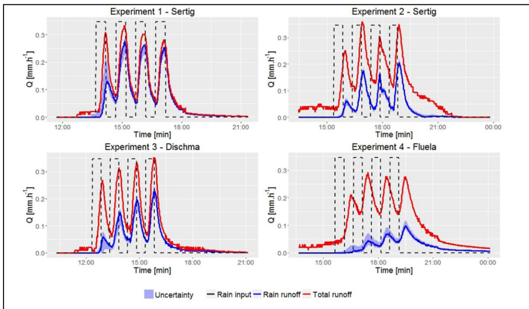
Figure 5 - Runoff from the experimental snow block during all sprinkling experiments.
