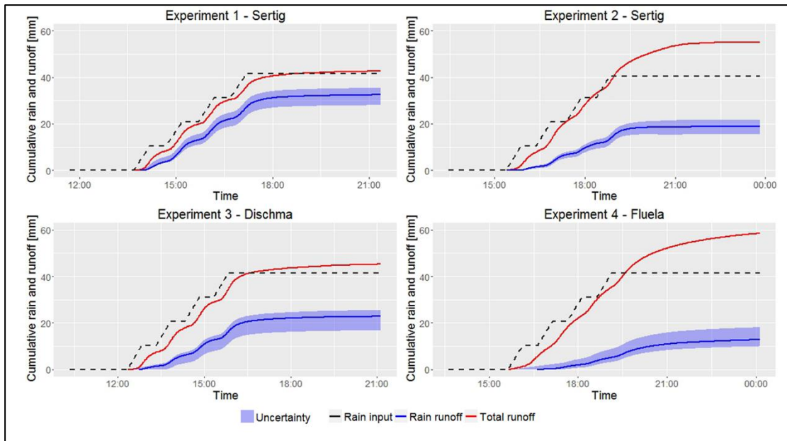
Figure 6 – Cumulative runoff from the investigated snow cube.
