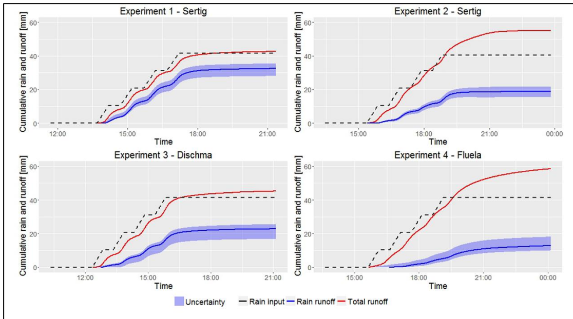
Figure 6 – Cumulative outflow runoff from the investigated snow cube.
