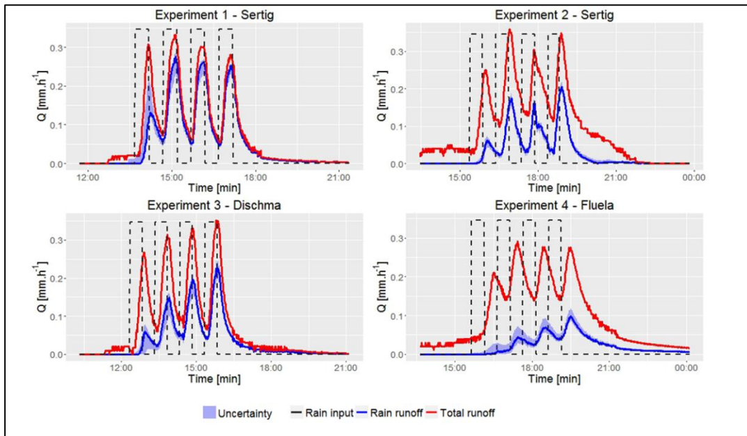
Figure 5 - Runoff from the experimental snow block during all artificial ROS sprinkling experiments .
