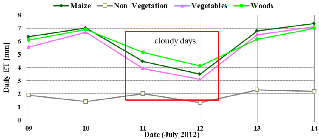
Fig. 1. EC dis-aggregated daily ET for each land covers from 9 to 14 July 2012
