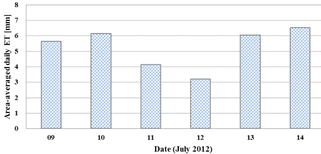
Fig. 2. Area-averaged daily ET over the study area
