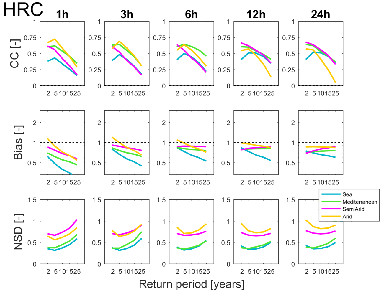
Figure 7: Comparison of IDF values between HRC and radar for different climatic regions. Blue lines represent sea areas while green, pink and orange lines represent Mediterranean, semiarid and arid climates respectively. The first row of panels shows the CC for different durations, the second row the Bias and the third row the NSD.
