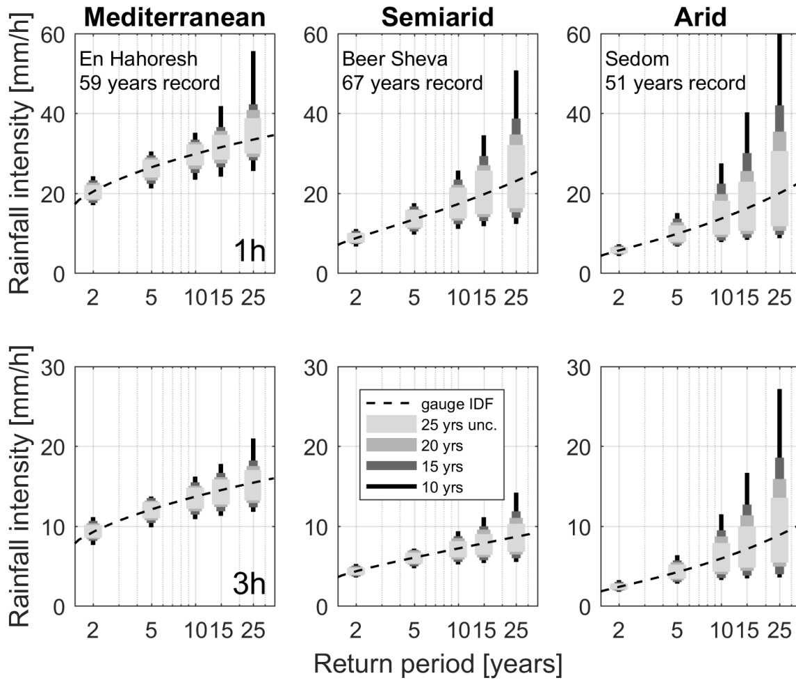
Figure 9: Uncertainty related to the record length for 1 and 3 h durations for three example cases in Mediterranean (En Hahoresht), semiarid (Beer Sheva) and arid (Sedom) climates. The dashed lines show the IDF curves from the full records (59, 67 and 51 years, respectively) and the vertical bars show the width of the 5-95 th quantile interval of the 999 bootstrap sampling repetitions for record lengths of 10, 15, 20 and 25 years. Width and light of the colour of the bars increase with the record length.
