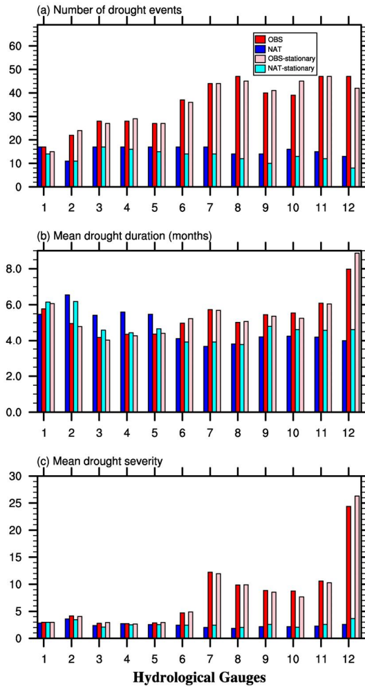
Figure 8. Characteristics of hydrological drought events based on streamflow time series with or without human influences during 1961-2010 for 12 hydrological gauges. A hydrological drought event is selected when the Standardized Streamflow Index (SSI) is continuously below -0.8 for at least 3 months. Blue and red bars are for the results based on transient 30-year climatologies, and cyan and pink bars are for results based on the 50-year (1961-2010) climatology.
