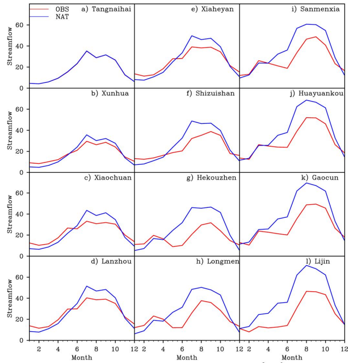
Figure 3. Monthly mean naturalized (blue) and observed (red) streamflow ( 10^8 \text{ m}^3 ) averaged over 1961-2010 for 12 hydrological gauges located from upper to lower mainstream of Yellow River.
