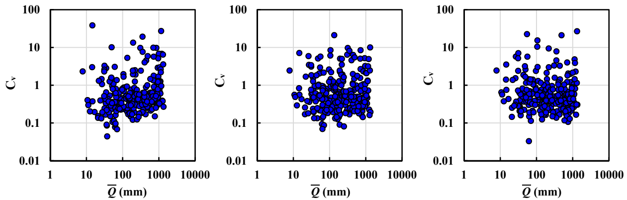
Figure 132: C_v values of projected future trends \Delta\bar{Q}_e under (left) RCP2.6, (middle) RCP4.5 and (right) RCP8.5 Scenarios.
