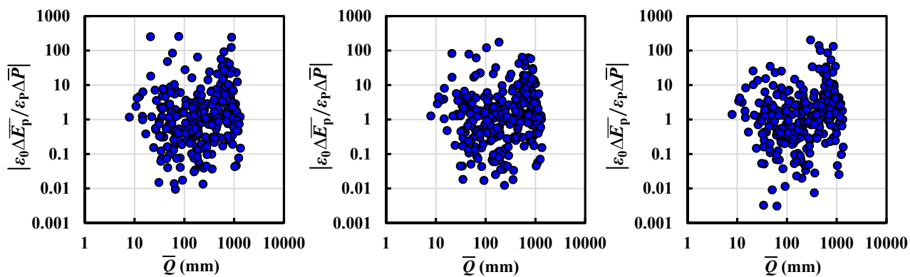
Figure 134: Exploring the controlling factor in the projected climate change under (left) RCP2.6, (middle) RCP4.5 and (right) RCP8.5.
