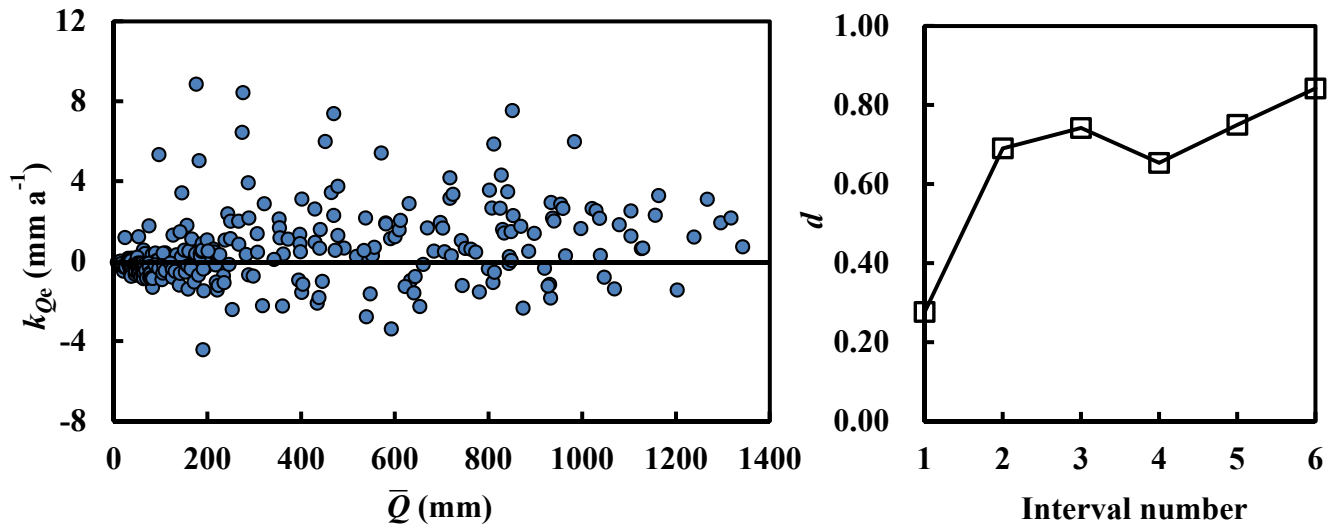
Figure 89: Relationship between observed runoff trends k_{Qe} and mean annual runoff \bar{Q} for the study catchments (left) and values of d in each interval according to \bar{Q} (right). Interval numbers 1 to 6 correspond to six intervals 0–200, 200–400, 400–600, 600–800, 800–1000 and 1000–1400.
