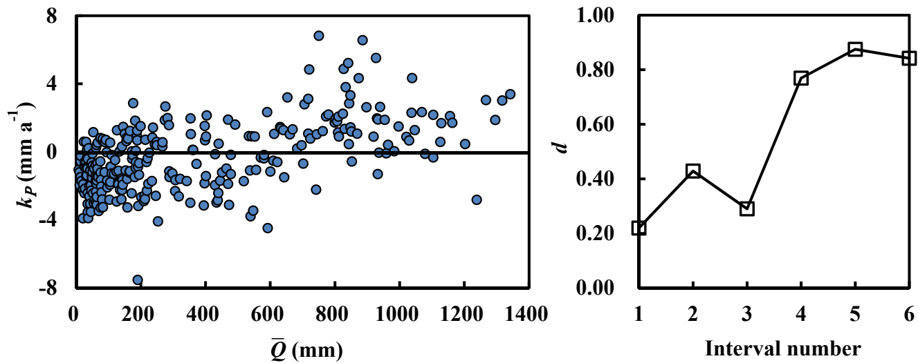
Figure 10: Relationship between observed runoff trends k_P and mean annual runoff \bar{Q} for the study catchments (left) and values of d in each interval according to \bar{Q} (right). Interval numbers 1 to 6 correspond to six intervals 0–200, 200–400, 400–600, 600–800, 800–1000 and 1000–1400.
