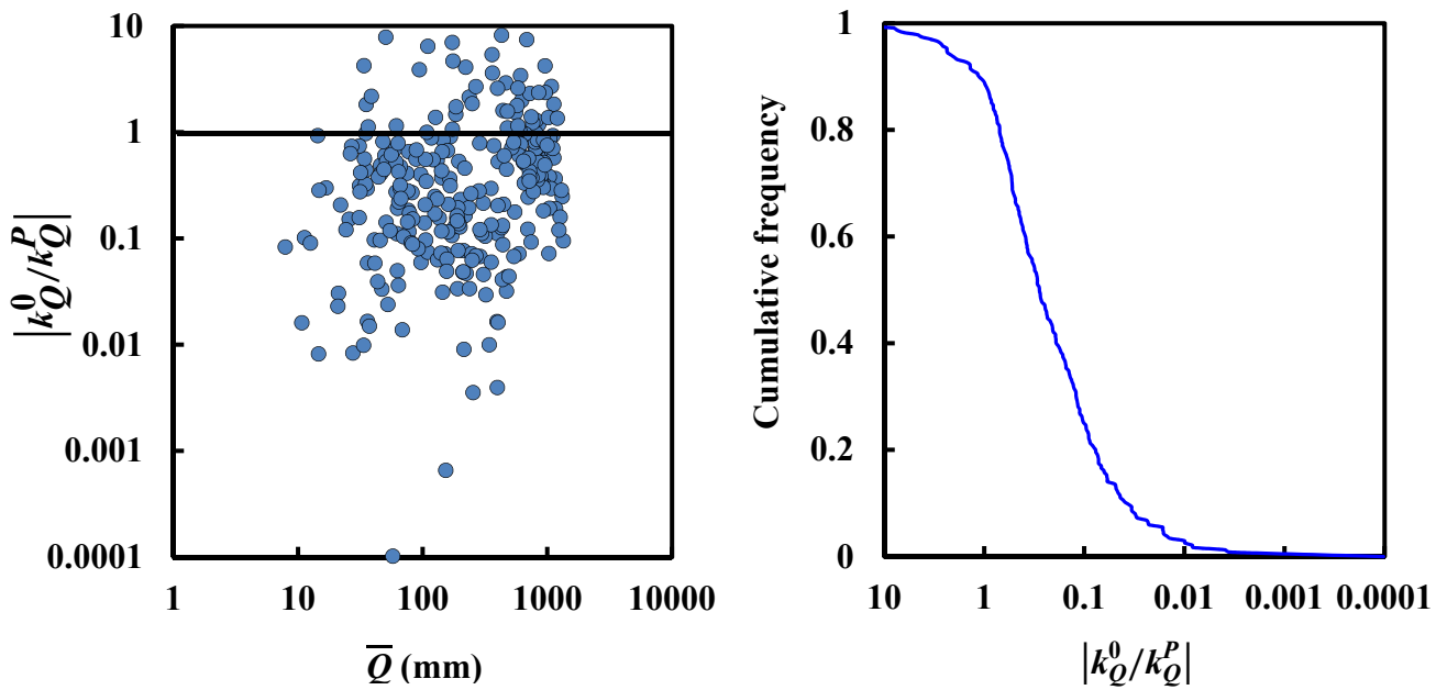
Figure 910: Exploring the controlling factor in the DDWW pattern according to the Budyko hypothesis. (left) Relationship between the ratio of absolute k_Q^0 ( =\varepsilon_0 k_{E_p} , the part of the estimated runoff trends k_{Qe} generated from potential evapotranspiration changes) to absolute k_Q^P ( =\varepsilon_p k_p , the part of k_{Qe} generated from precipitation changes) and the mean annual runoff \bar{Q} . (right) The cumulative frequency curve of |k_Q^0/k_Q^P| .
