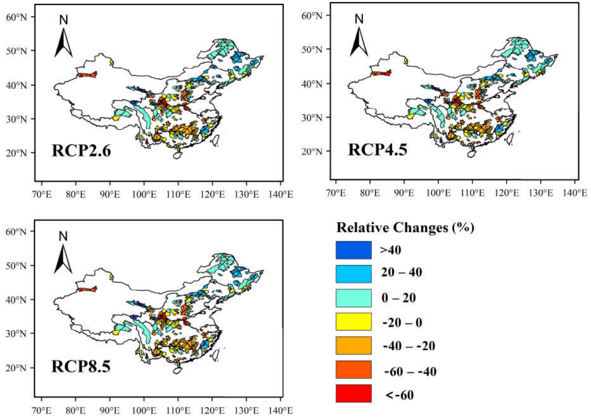
Figure 145: Spatial distribution of the model-averaged relative changes in mean annual runoff \bar{Q} ( =\Delta\bar{Q}_v/\bar{Q} ) for the period of 2001 to 2050 under three different scenarios. Hatched areas denote regions with C_v values smaller than 0.5, whereas double-hatched areas represent regions with C_v values smaller than 1.
