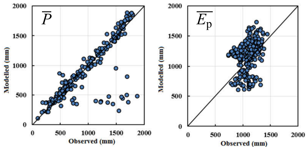
Figure 156: Comparison of the observed meteorological data with the simulations from the GFDL-ESM2M model for the period 1956–2000.
