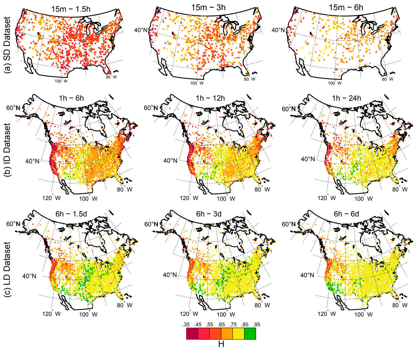
Figure 4. Spatial distribution of the scaling exponent for the first (i.e. with minimum d_1 ) 6-, 12-, and 24-duration scaling intervals (first, second, and third col., respectively) for SD, ID, and LD datasets (first, second, and third row, respectively). These scaling intervals correspond to the first column of matrices in Fig. 1 and 2.
