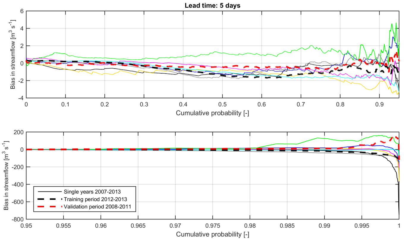
Figure 11: Difference between CDFs of the measurements and CDFs of the uncorrected streamflow forecasts per hydrological year (upper panel cumulative probability 0 – 0.95 and lower panel 0.95 – 1.0). Each thin line refers to a single year between 2007 and 2013. This figure is for a lead time of 5 days.
