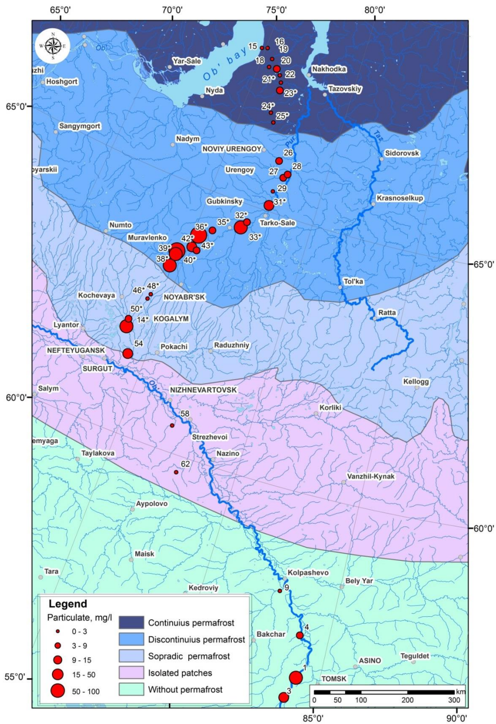
884 Figure 1. Map of the study site, with permafrost zone boundaries. The size of the sampling points reflects the 885 concentration of particulate fraction (mg/L snw water ). The boundaries of permafrost zones are from Brown et al. (1997). 886
