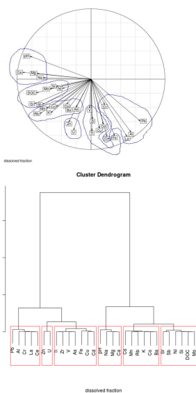
Figure 1 Reply: PCA Factorial map F1x2 of elements of a reconstructed table for the dissolved fraction. Partition of elements into 6 groups revealed by a CAH is shown by a contour line. B: Dendrogram of a hierarchical cluster performed on variables of a reconstructed table for the dissolved fraction using the Pearson correlation as a distance measure and Ward's method for the linkage rule.
