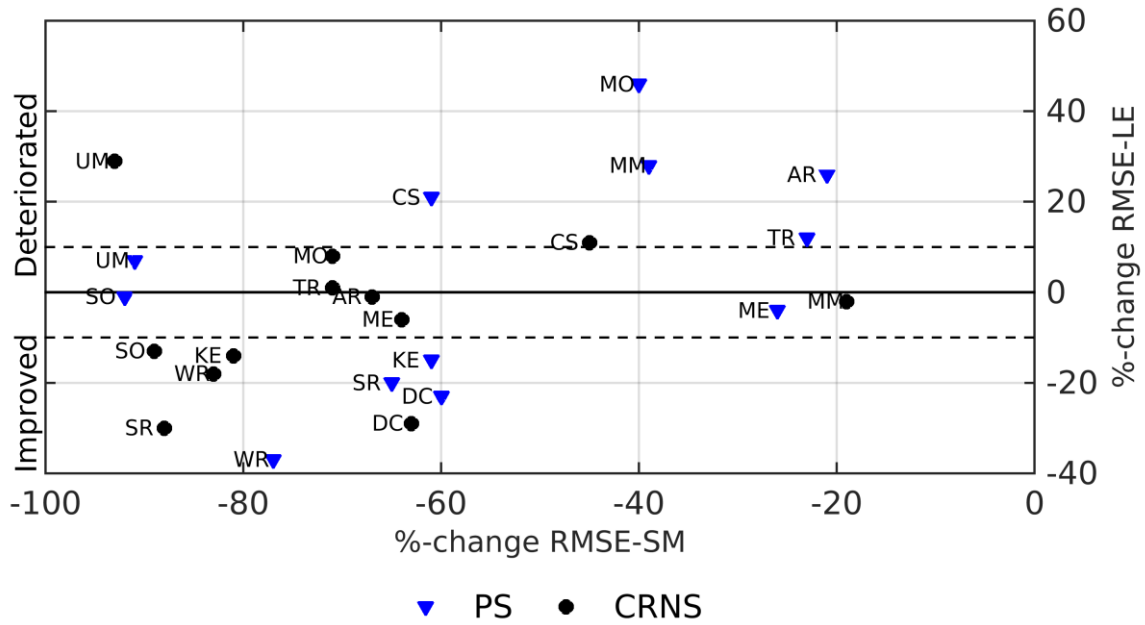
5 Figure 6: Relative change in Root Mean Square Error (RMSE) values after single-objective calibration against PS soil moisture and CRNS neutron count data. Change in RMSE between observed and simulated latent heat flux (LE) is plotted against change in RMSE between observed and simulated soil moisture.
