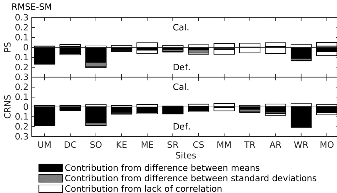
5 Figure 4: Objective function (Root Mean Square Error; RMSE ( \text{m}^3\text{m}^{-3} )) values between observed PS/CRNS soil moisture and JULES simulated soil moisture. For each calibration the RMSE of the default run is shown from the horizontal axis down, and the result after calibration is shown in the upward directions. The different error contributions from the MSE decomposition are shown as stacked bar plots.
