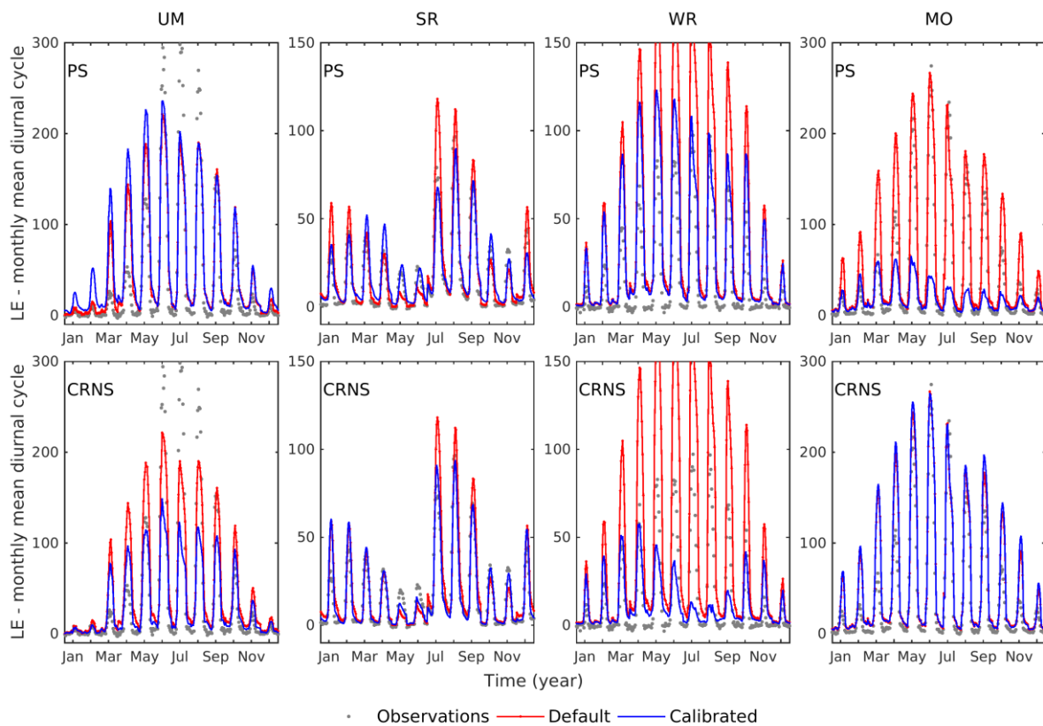
Figure 7: Monthly mean diurnal latent heat flux (LE) cycles. The upper row contains PS calibrated solutions, the lower row shows the CRNS calibrated solutions. The upper row contains PS calibrated solutions, the lower row shows the CRNS calibrated solutions.
