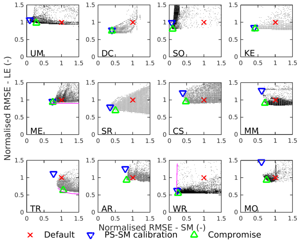
5 Figure 9: All runs from the two-objective calibrations against PS soil moisture and day time hourly latent heat flux (LE) at each site. Default run, PS-SM single objective calibrated run, and compromise solution runs are shown on top. All values were normalised to the values of the Default run. The plots were zoomed in to the area of 0 to 1.5 times the Default values.
