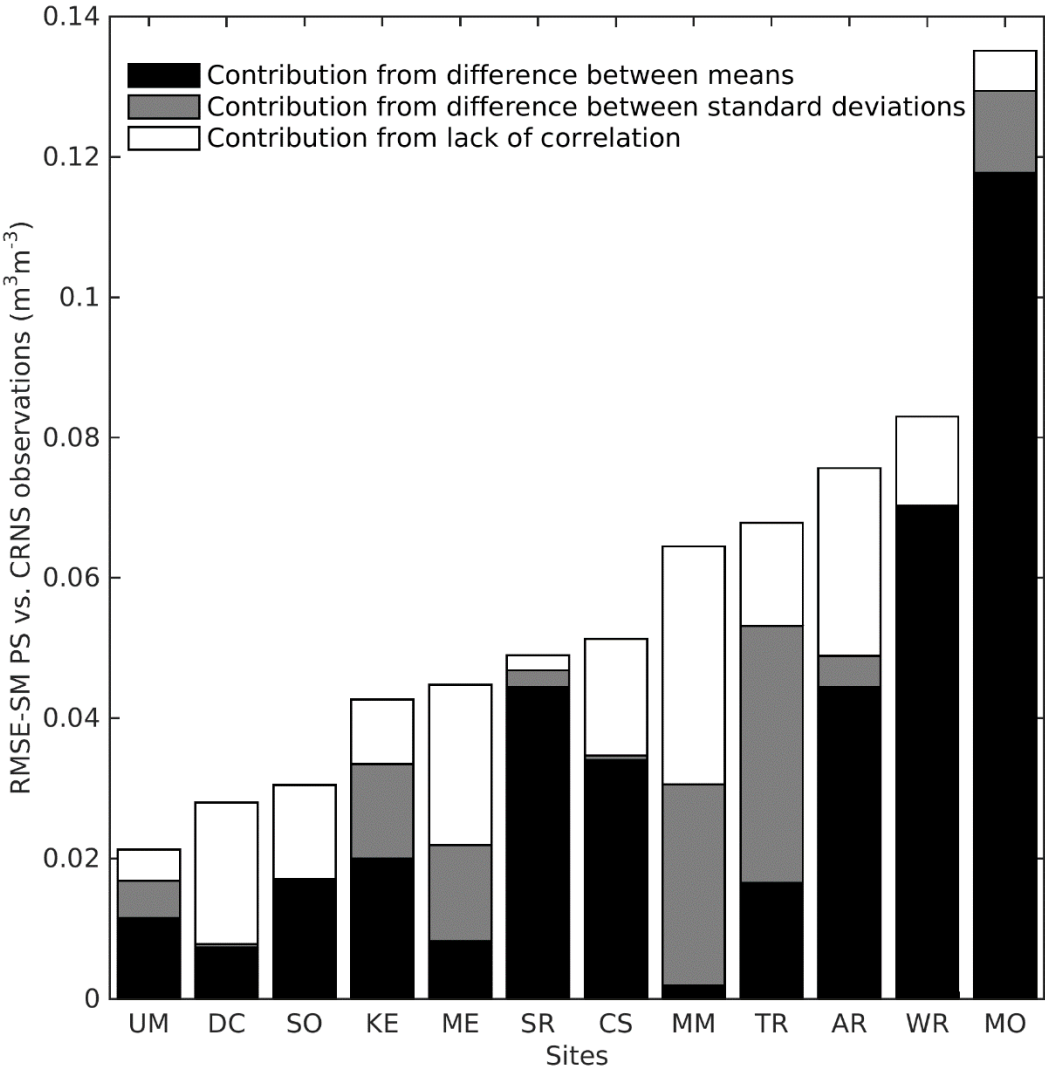
Figure 3: Root Mean Squared Error (RMSE) between observed PS and CRNS soil moisture (SM; \text{m}^3\text{m}^{-3} ). MSE decomposition (Gupta et al., 2009) was calculated and the fractions were then applied to the RMSE values. Sites are ranked from most similar to most different.
