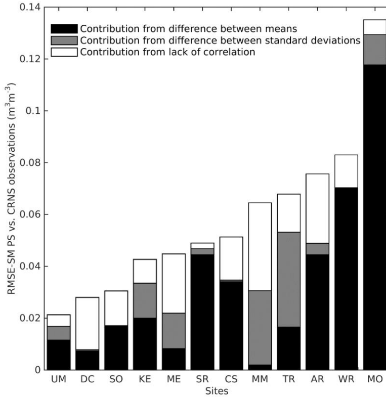
Figure 3: Root-Mean-Squared-Error (RMSE) between observed PS and CRNS soil moisture (SM; \text{m}^3\text{m}^{-3} ). MSE decomposition (Gupta et al., 2009) was calculated and the fractions were then applied to the RMSE values. Sites are ranked from most similar to most different.
