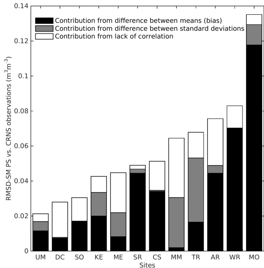
Figure 3: Root Mean Squared Deviation (RMSD) between observed PS and CRNS soil moisture (SM; m^3m^{-3} ). MSD decomposition (Gupta et al., 2009) was calculated and the fractions were then applied to the RMSD values. Sites ranked from most similar to most different.
